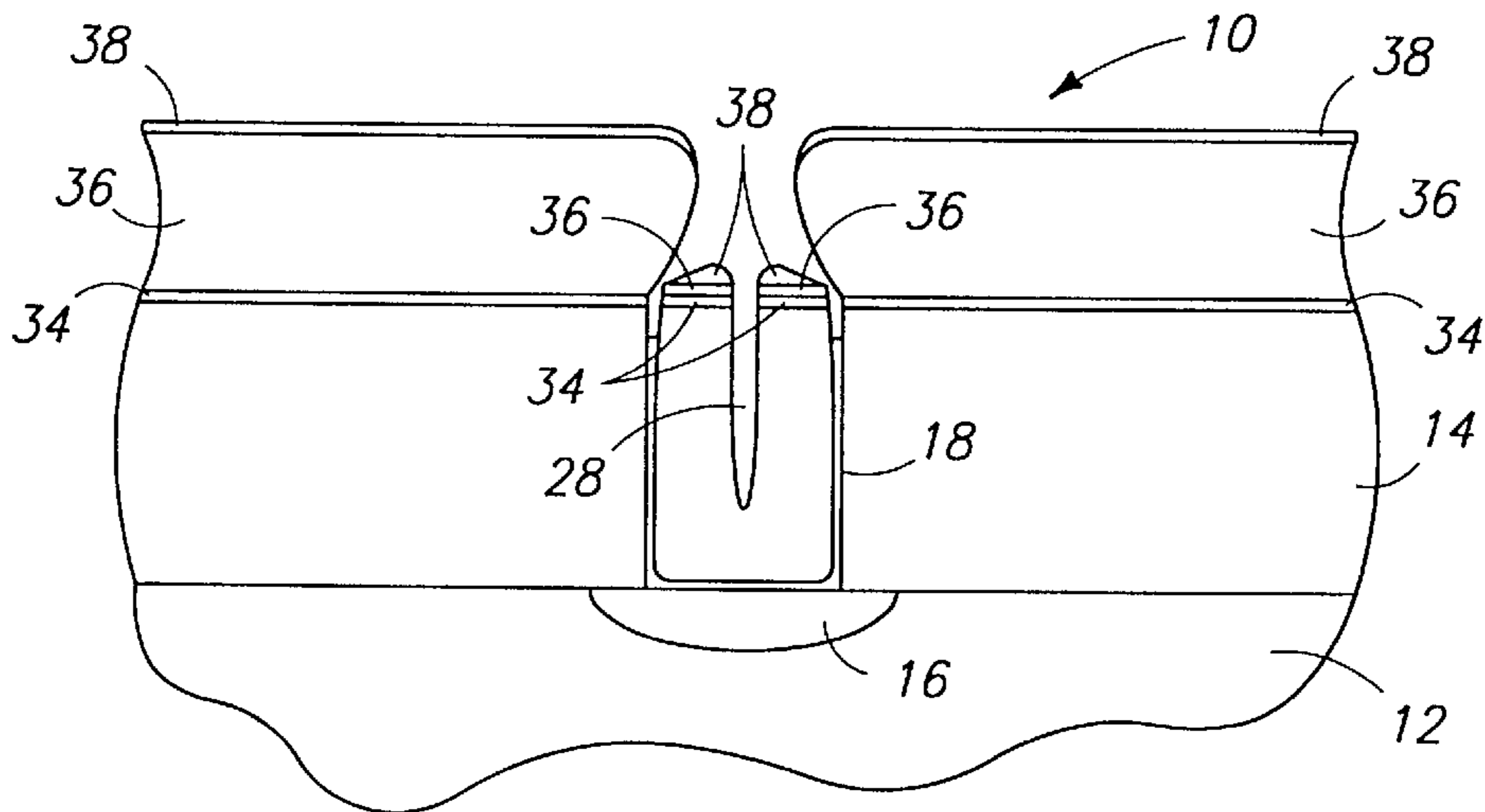
FIG. 3 PRIOR ART
