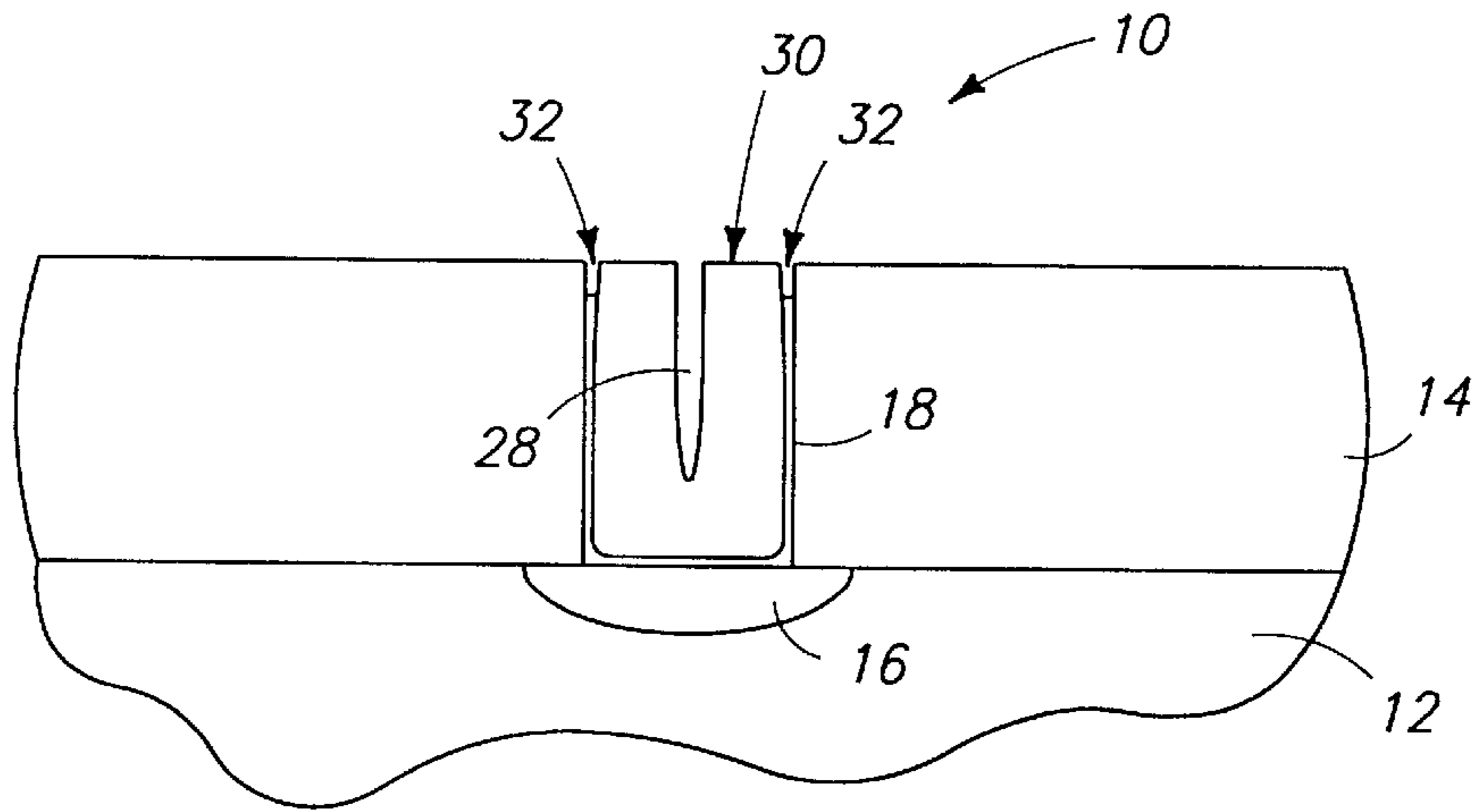
FIG. 2 PRIOR ART
