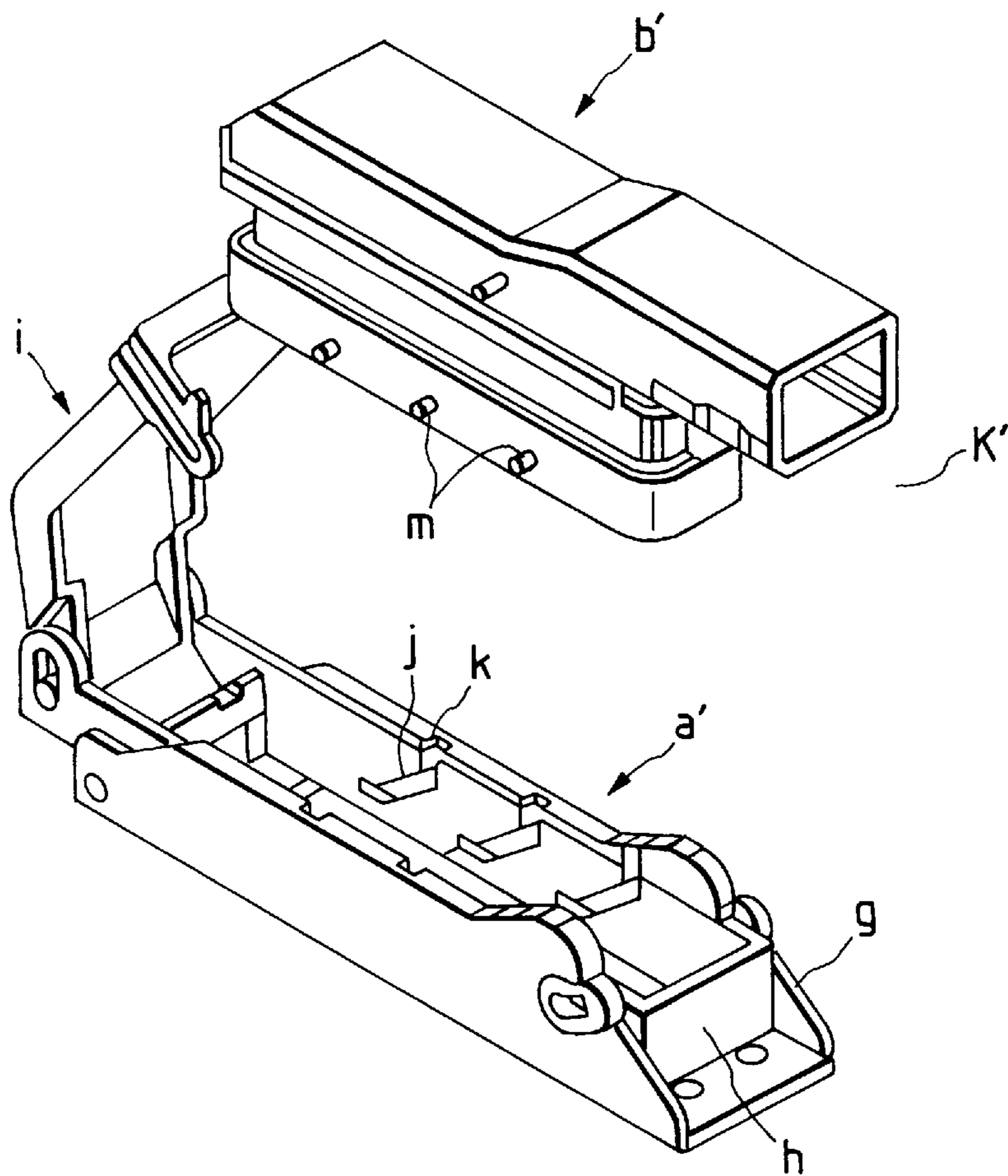
FIG. 11 PRIOR ART
