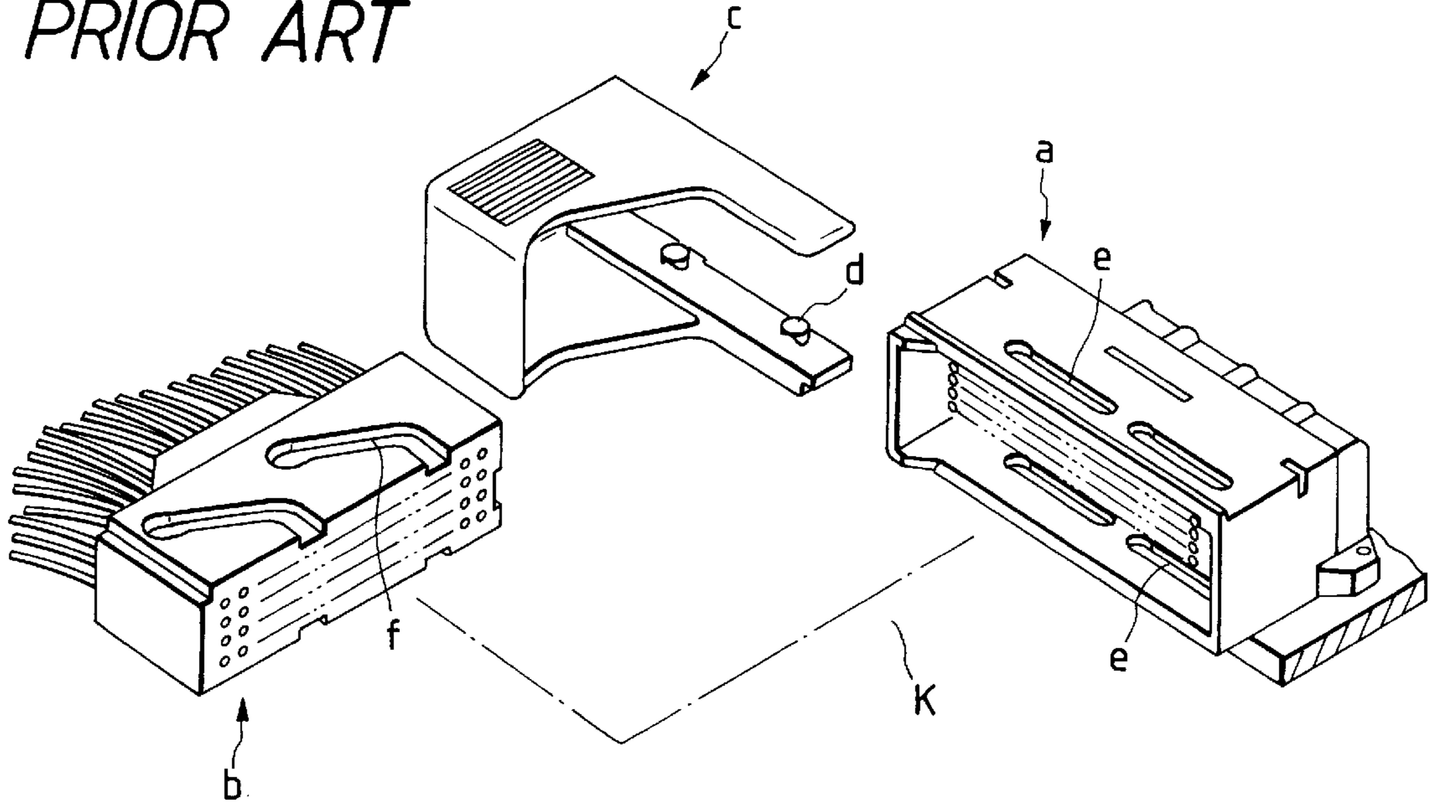
FIG. 9 PRIOR ART
