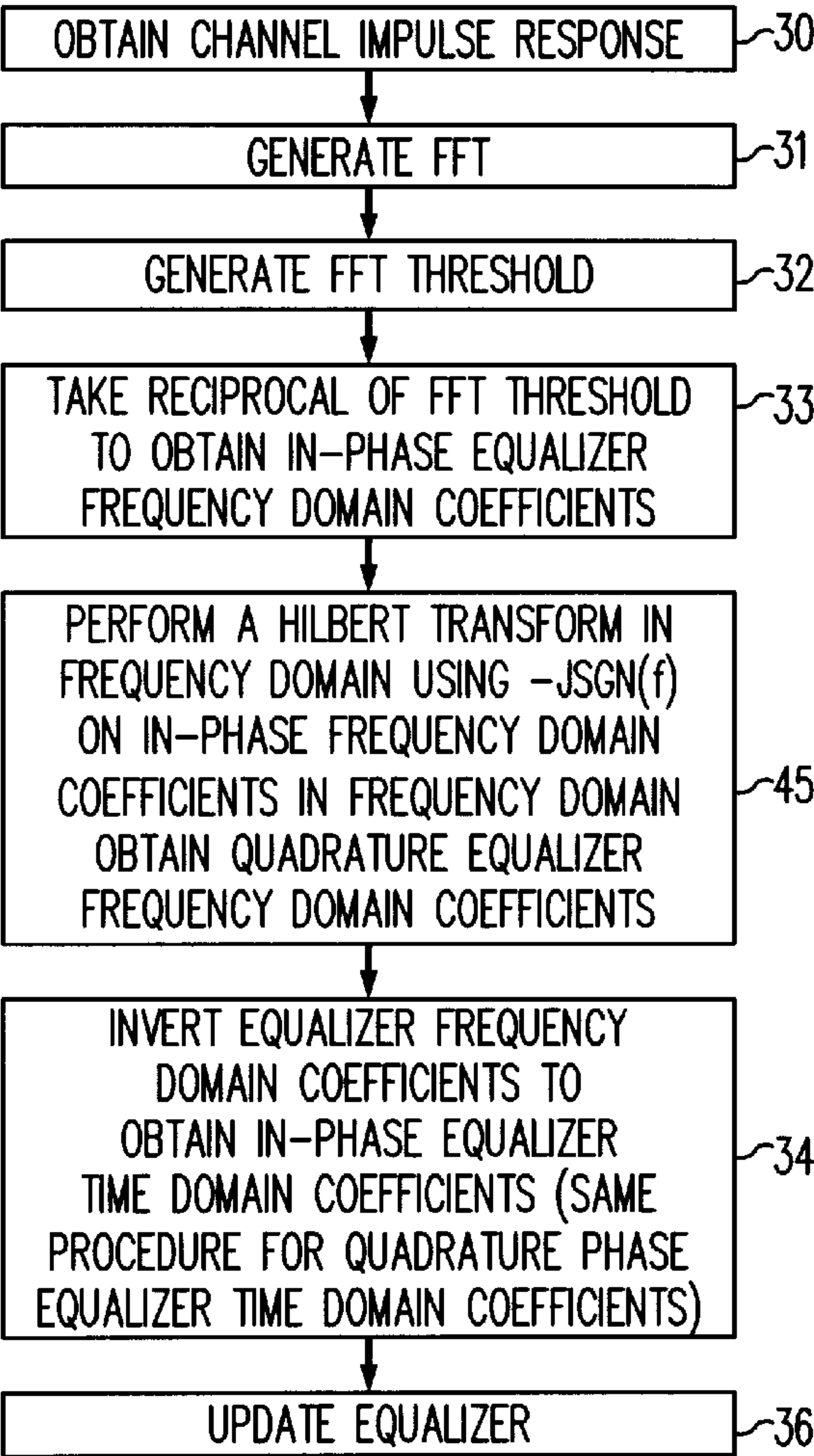
FIG. 16 CHANNEL SOUNDING PROCESS
