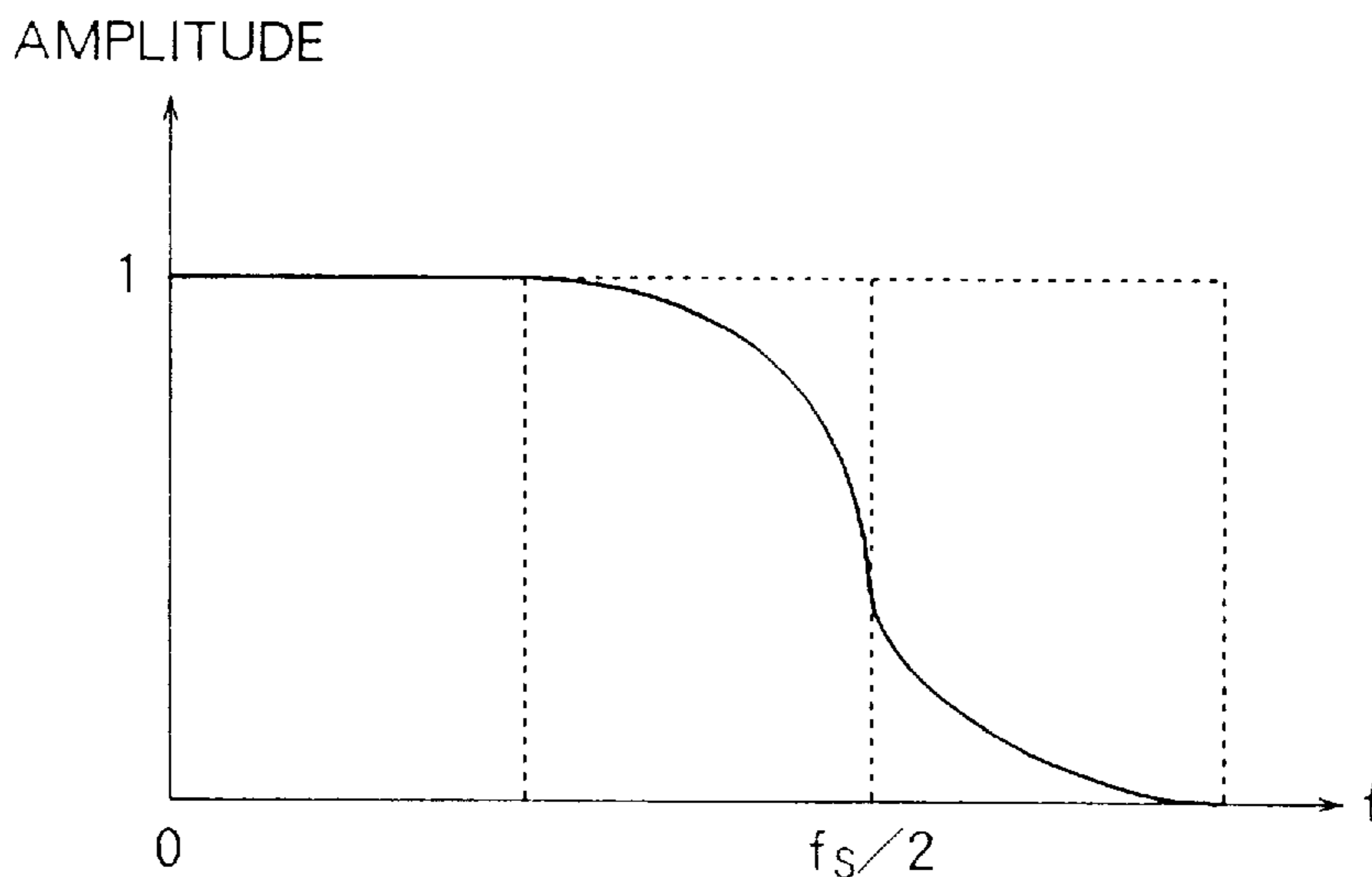
EXAMPLE OF TRANSFER FUNCTION OF LPF
