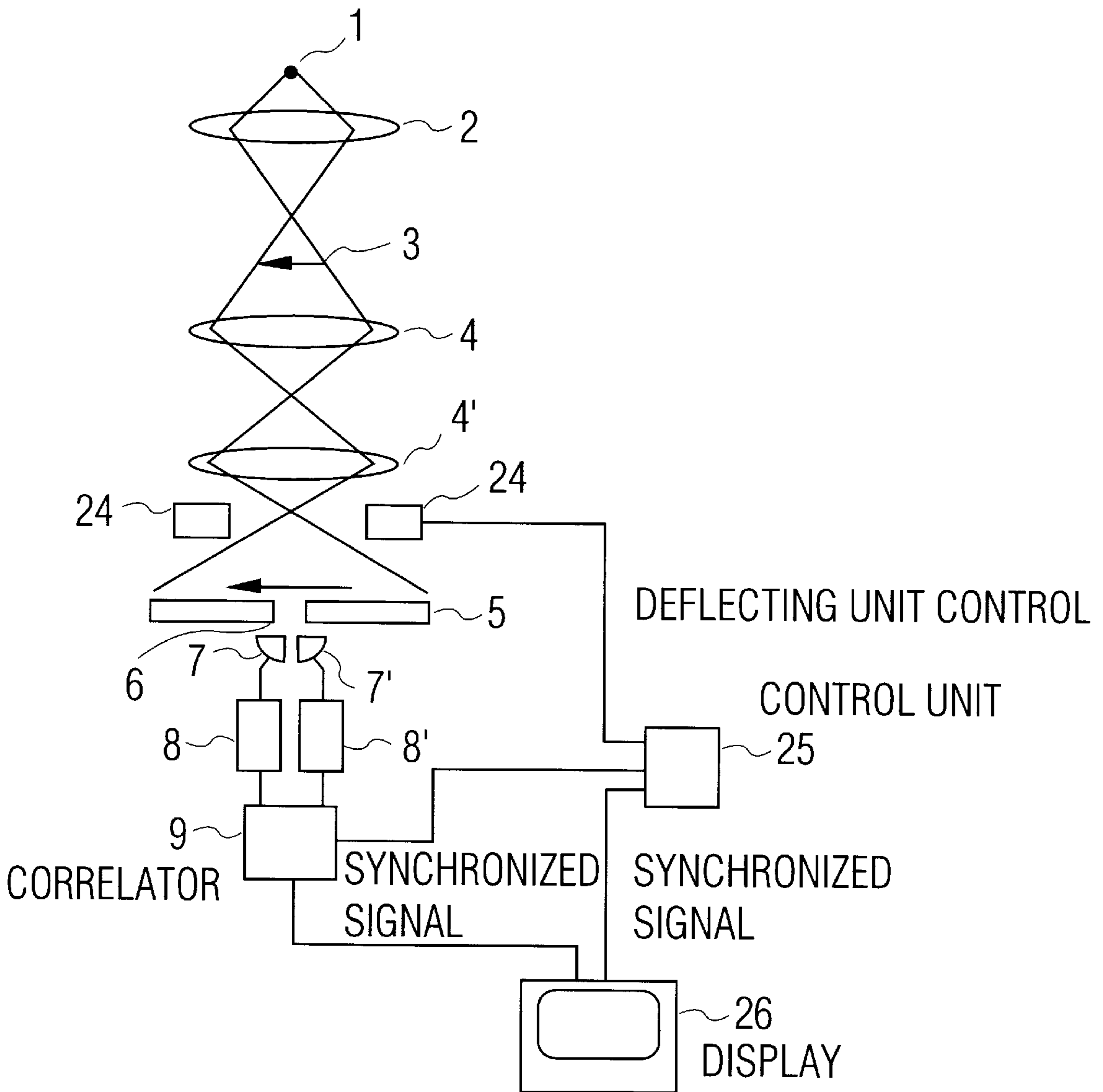
BLOCK DIAGRAM OF THE FOURTH EMBODIMENT OF THIS INVENTION
