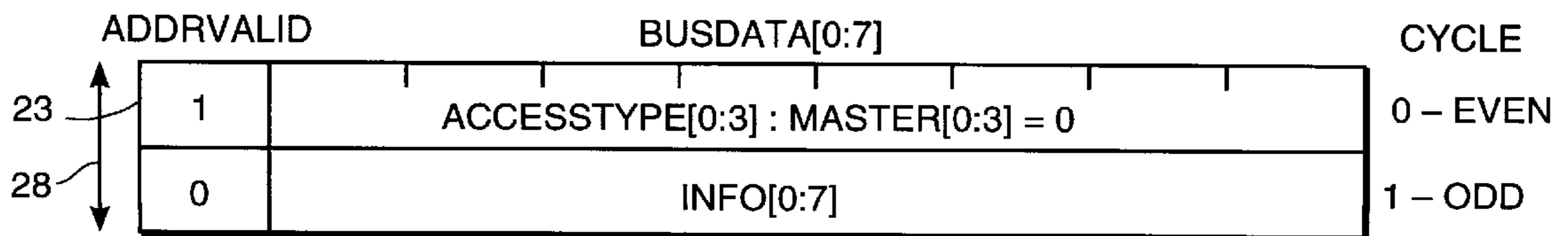
FIG 5 REJECT (NACK) CONTROL PACKET
