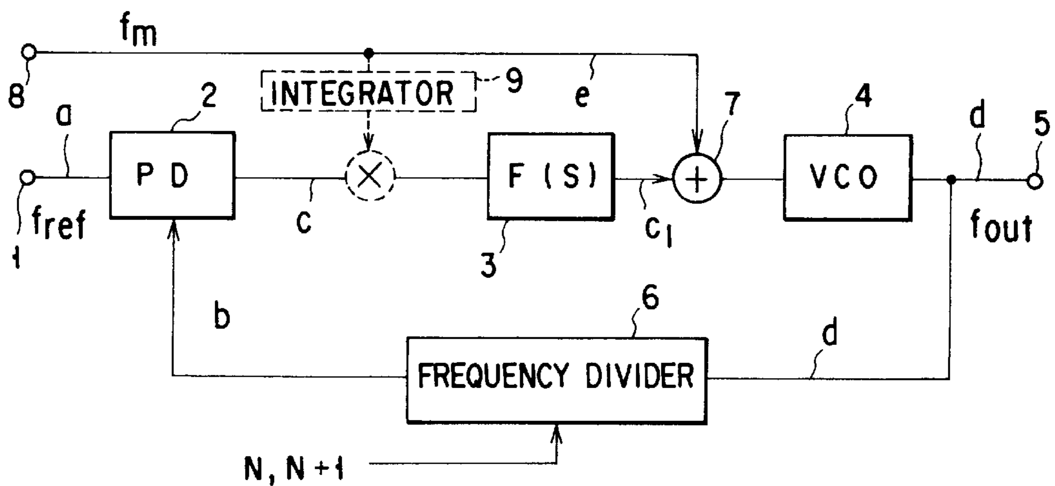
FIG. 15 (PRIOR ART)
