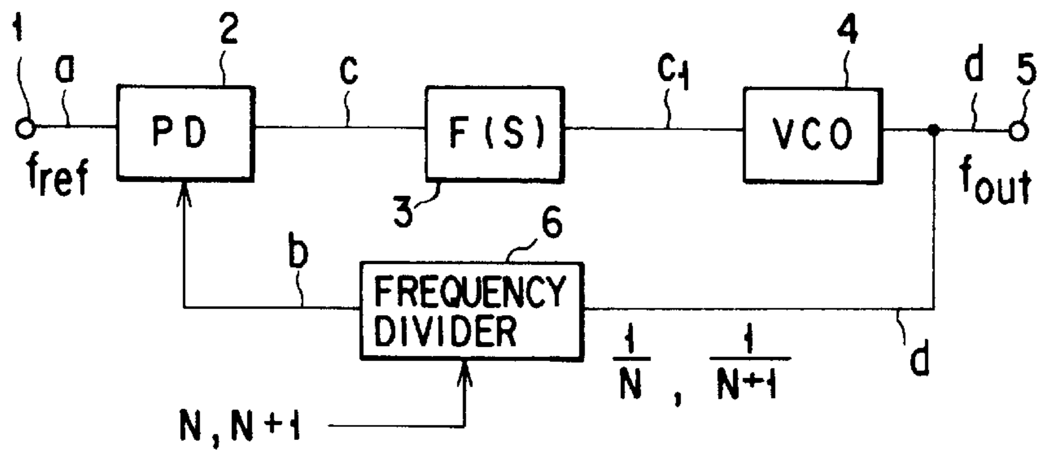
FIG. 13 (PRIOR ART)
