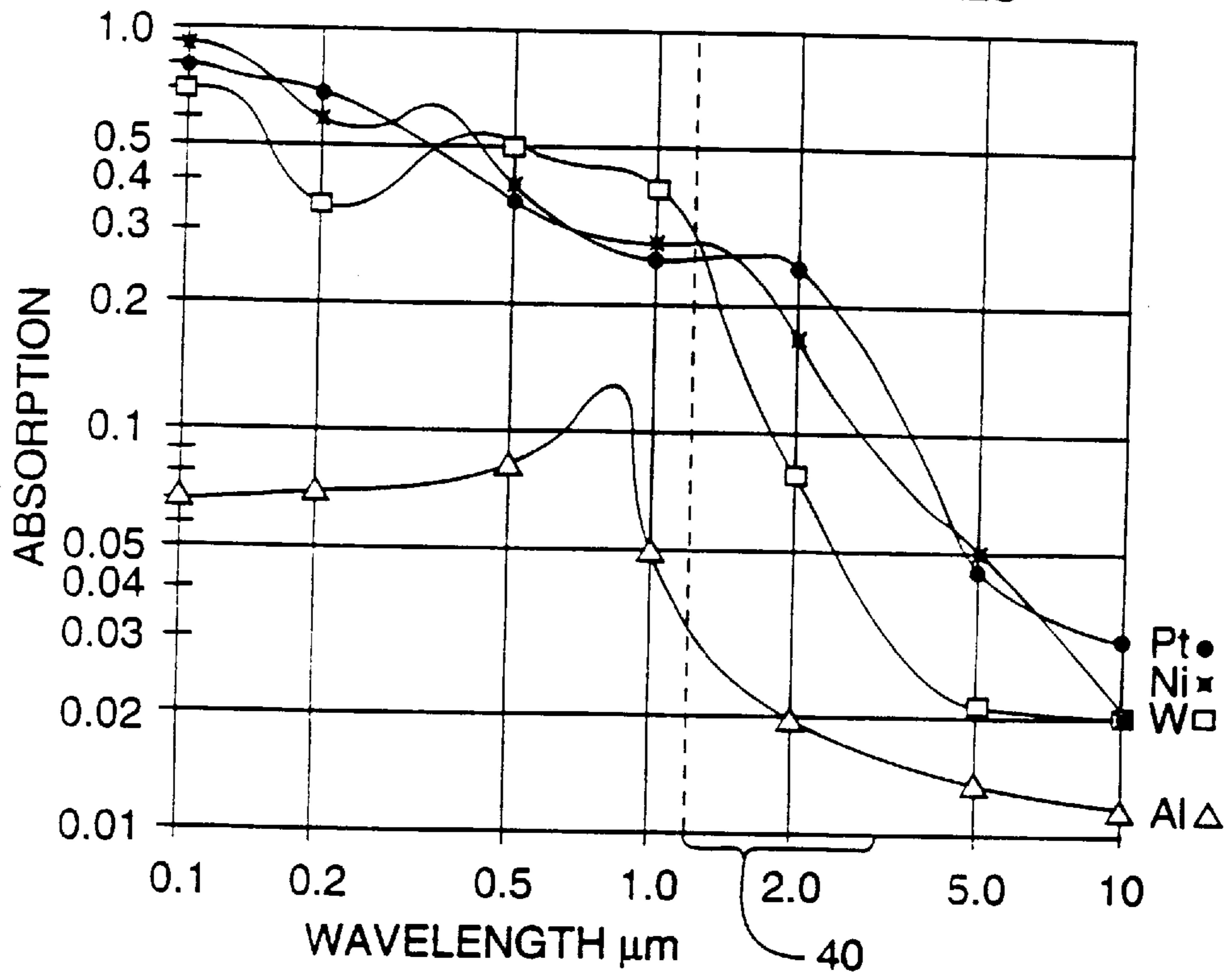
FIG. 7 OPTICAL ENERGY ABSORPTION VS. WAVELENGTH FOR METALS
