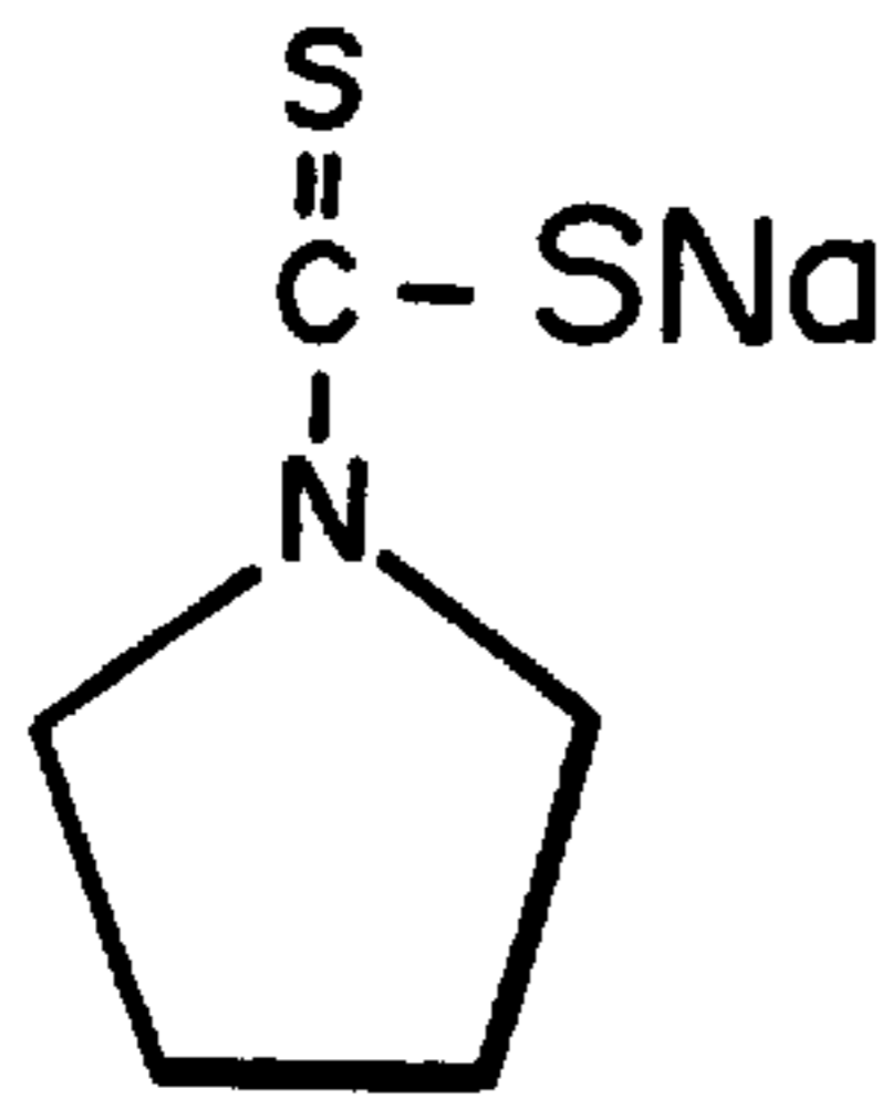
SODIUM PYRROLIDINE- N -CARBODITHIOATE
