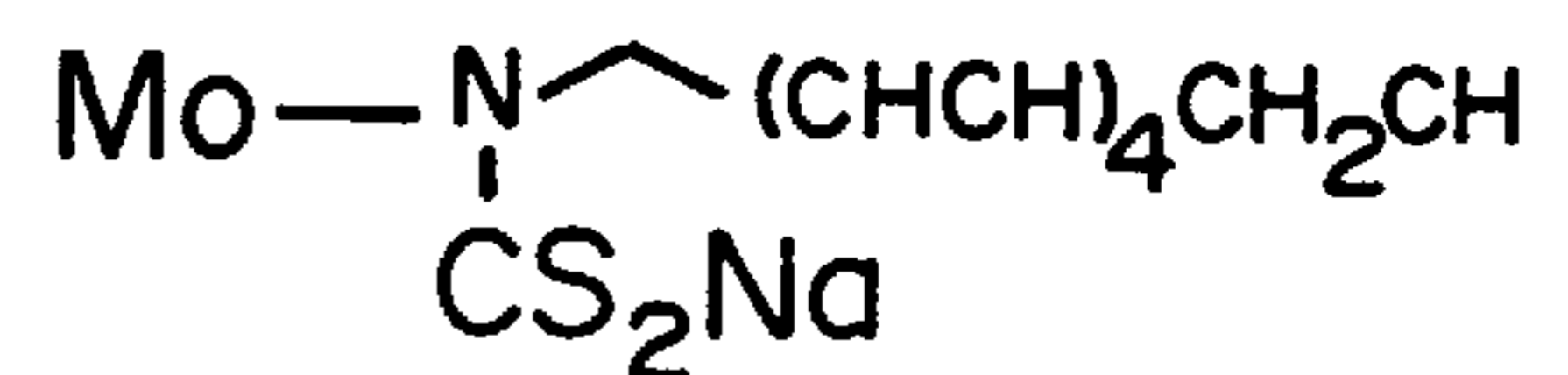
SODIUM N -METHYL-D-GLUCAMINE- N -CARBODITHIOATE
