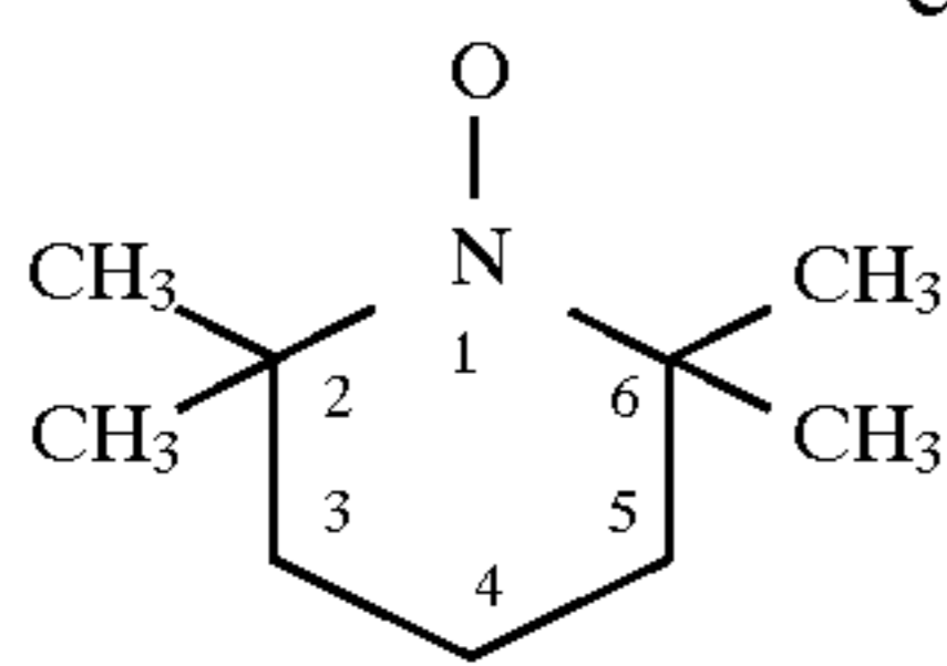
TEMPO (2,2,6,6-Tetramethyl-1- piperidinyloxy-) (2,2,6,6-Tetramethylpiperidine- N-oxyl)
