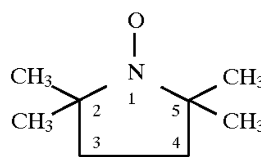
PROXYL (2,2,5,5-Tetramethyl-1-pyrrolidinyl-oxy-) (2,2,5,5-Tetramethylpyrrolidine-N-oxy)
