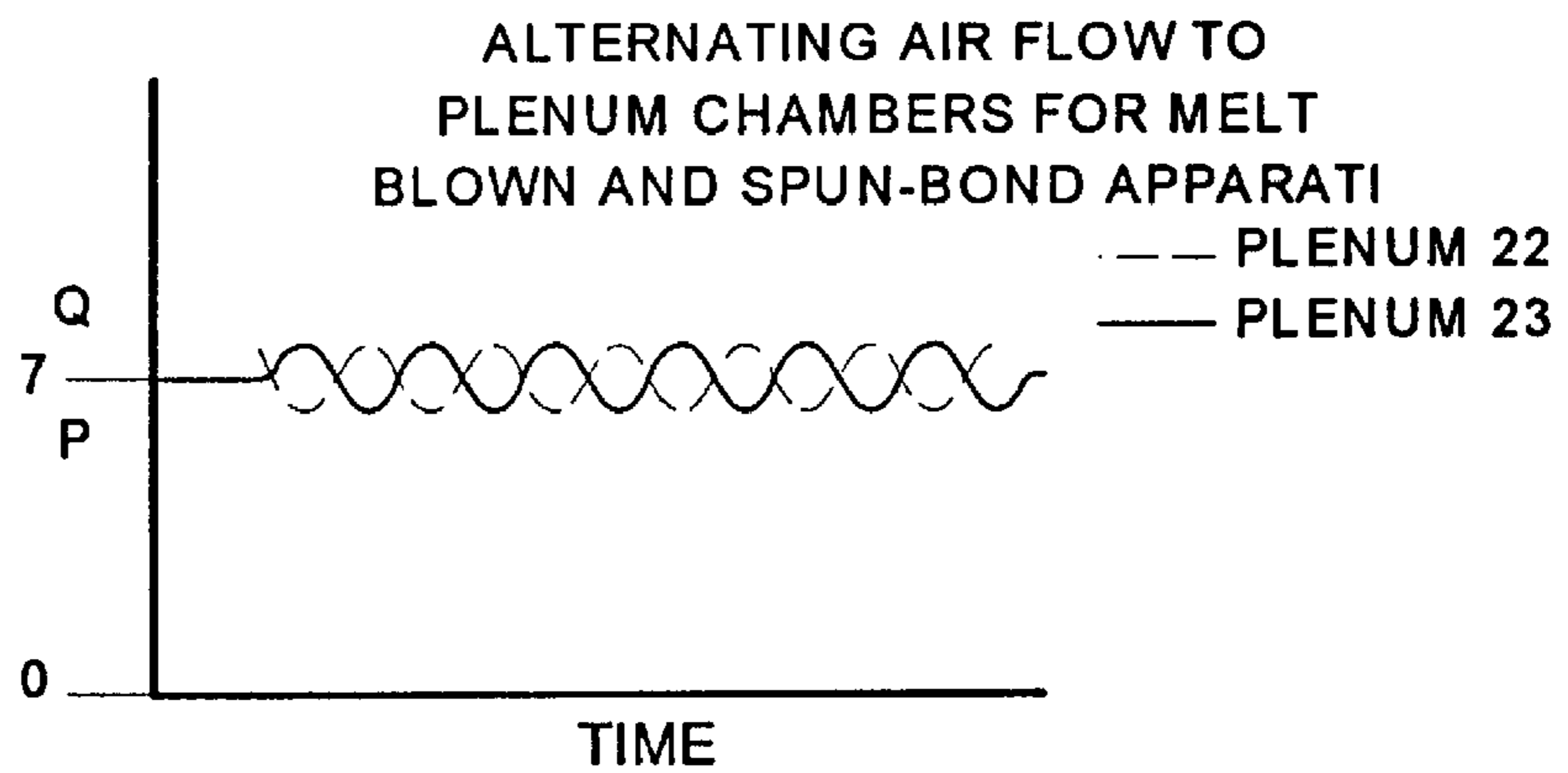
PRIOR ART FIG. 8B
