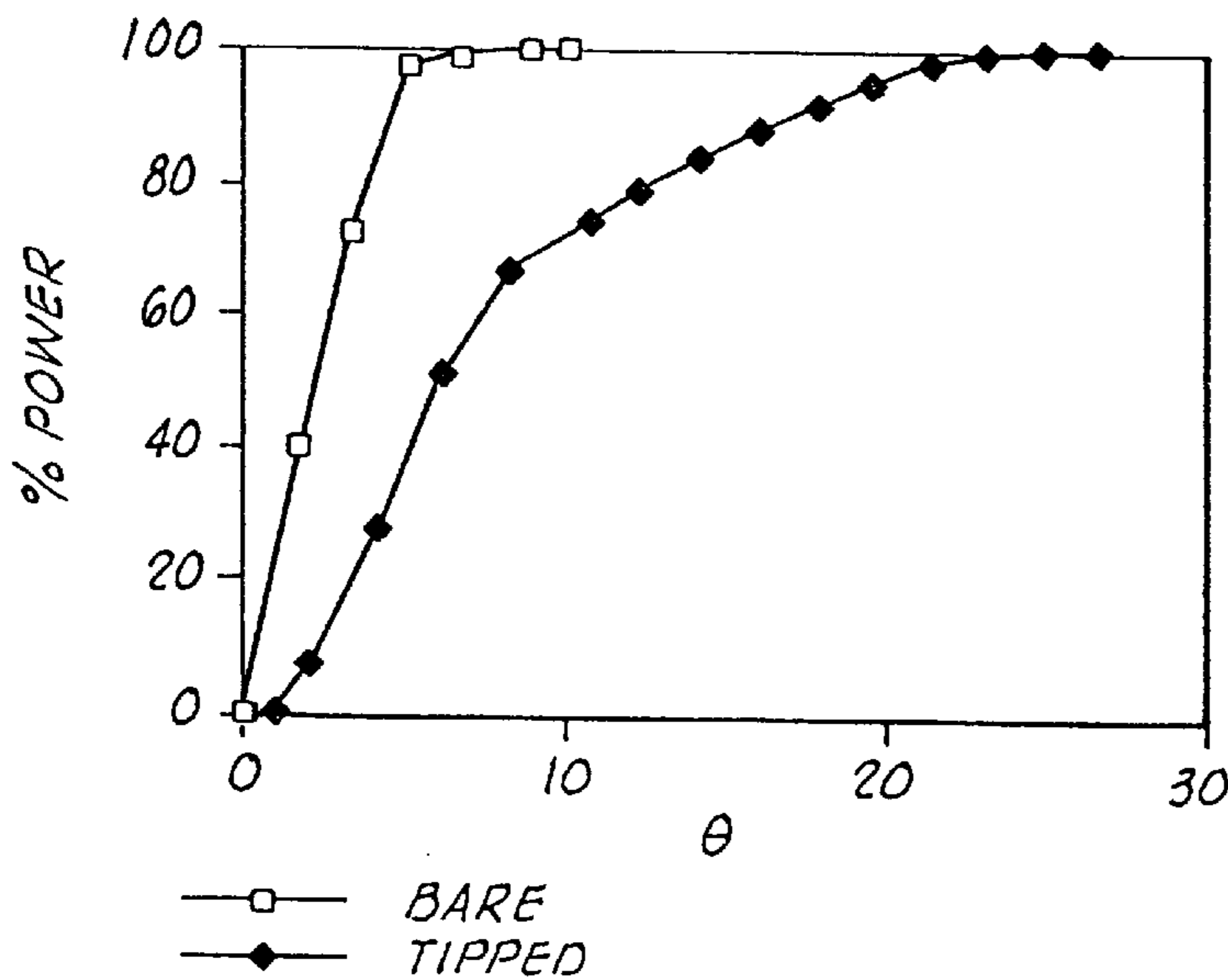
PERCENTAGE OF TOTAL EMITTED LASER POWER VERSUS INCLUDED ANGLE ( \theta ) FOR REPRESENTATIVE BARE AND TIPPED FIBERS AT 632.8 NM.
