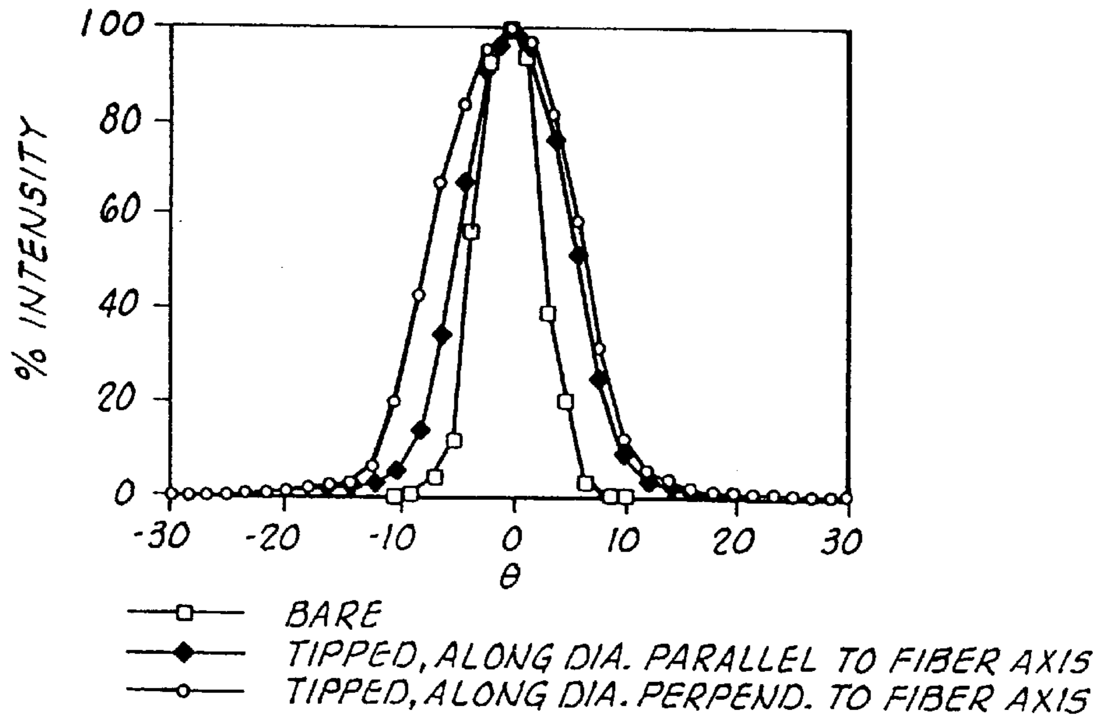
ANGULAR LIGHT INTENSITY DISTRIBUTION OF REPRESENTATIVE BARE AND TIPPED OPTICAL FIBER MEASURED AT 632.8 NM WAVELENGTH.
