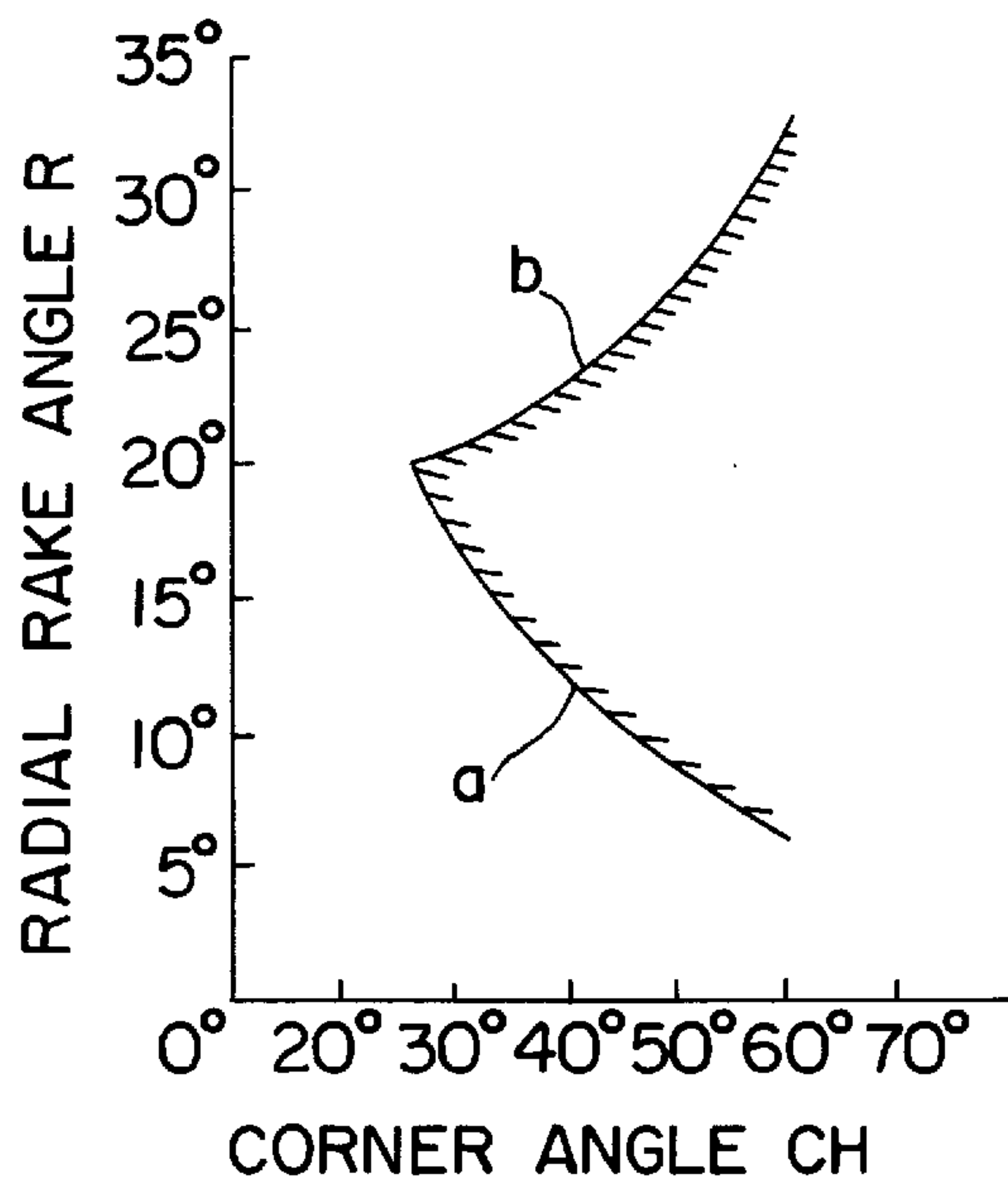
FIG. 13 PRIOR ART
