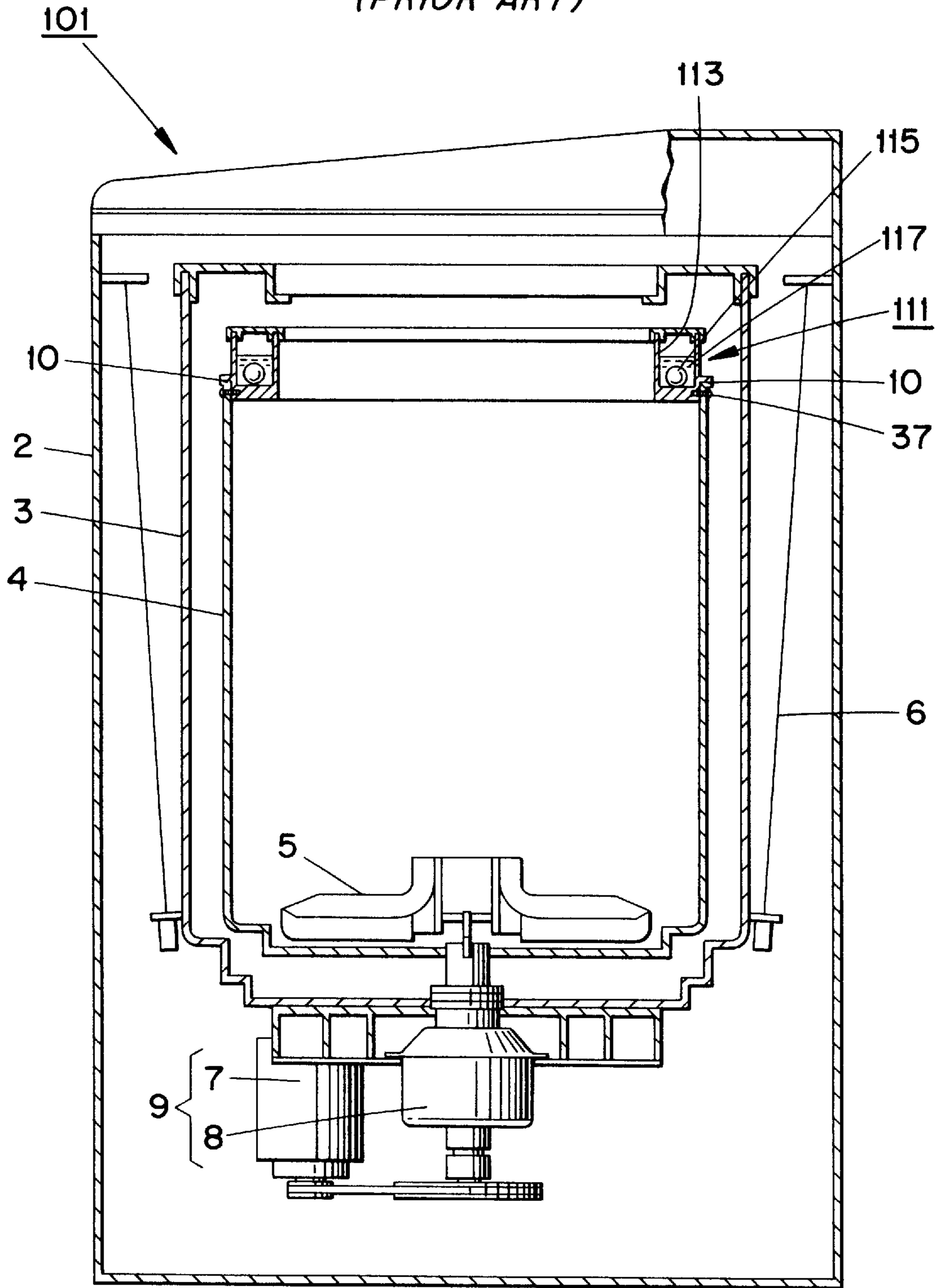
FIG. 9 (PRIOR ART)
