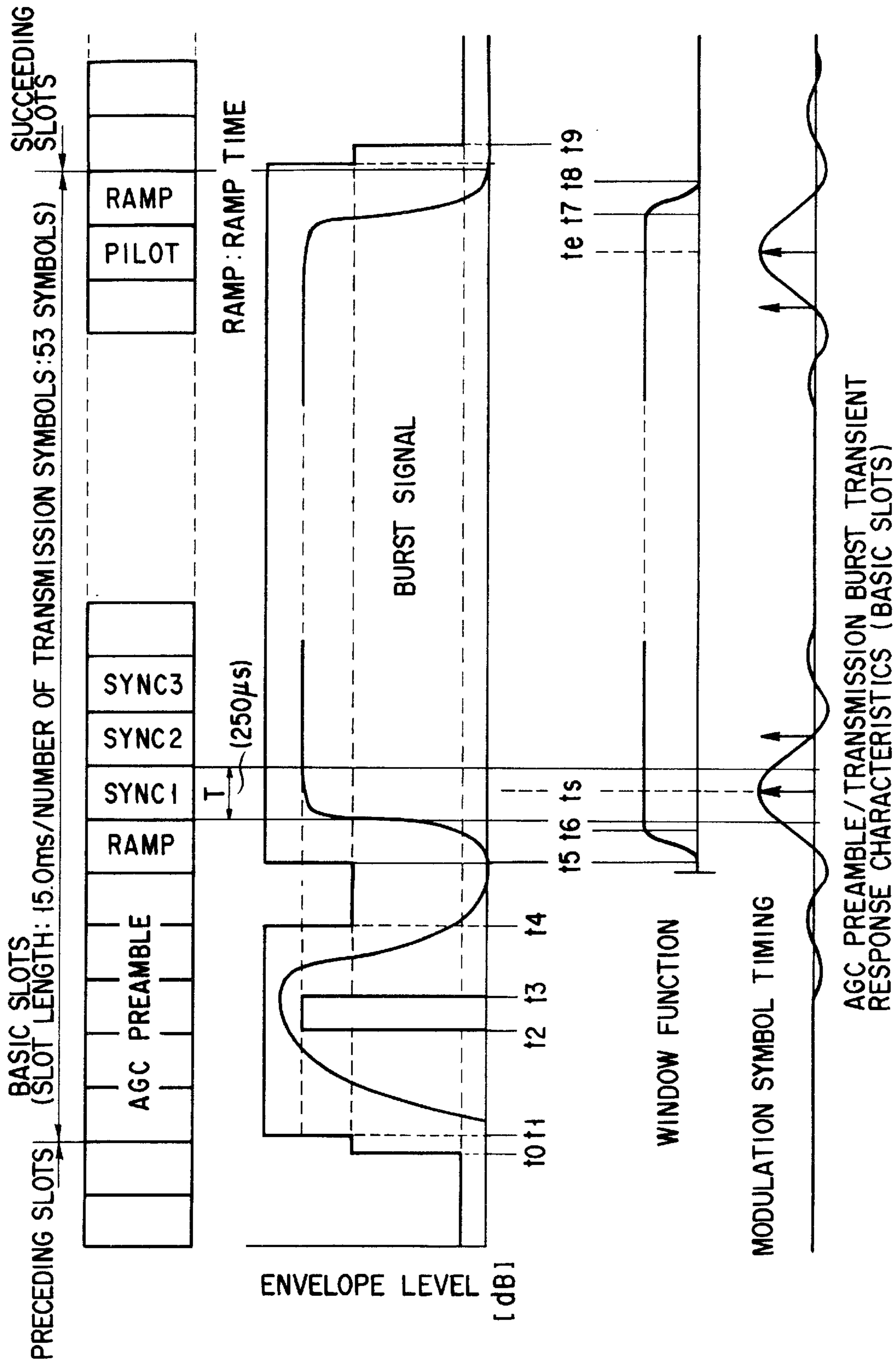
FIG. 15 (PRIOR ART)
