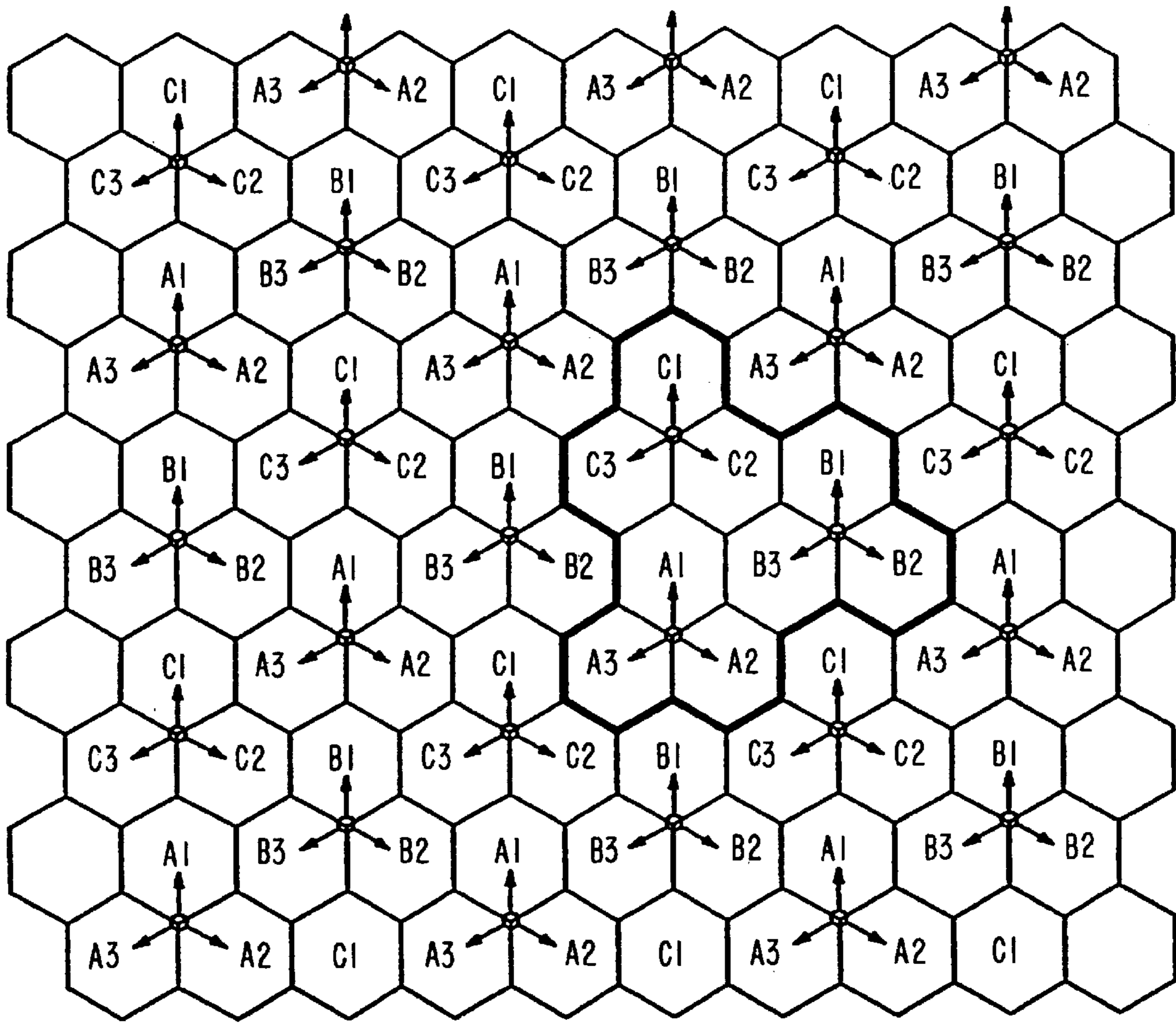
3/9 CELL PATTERN
