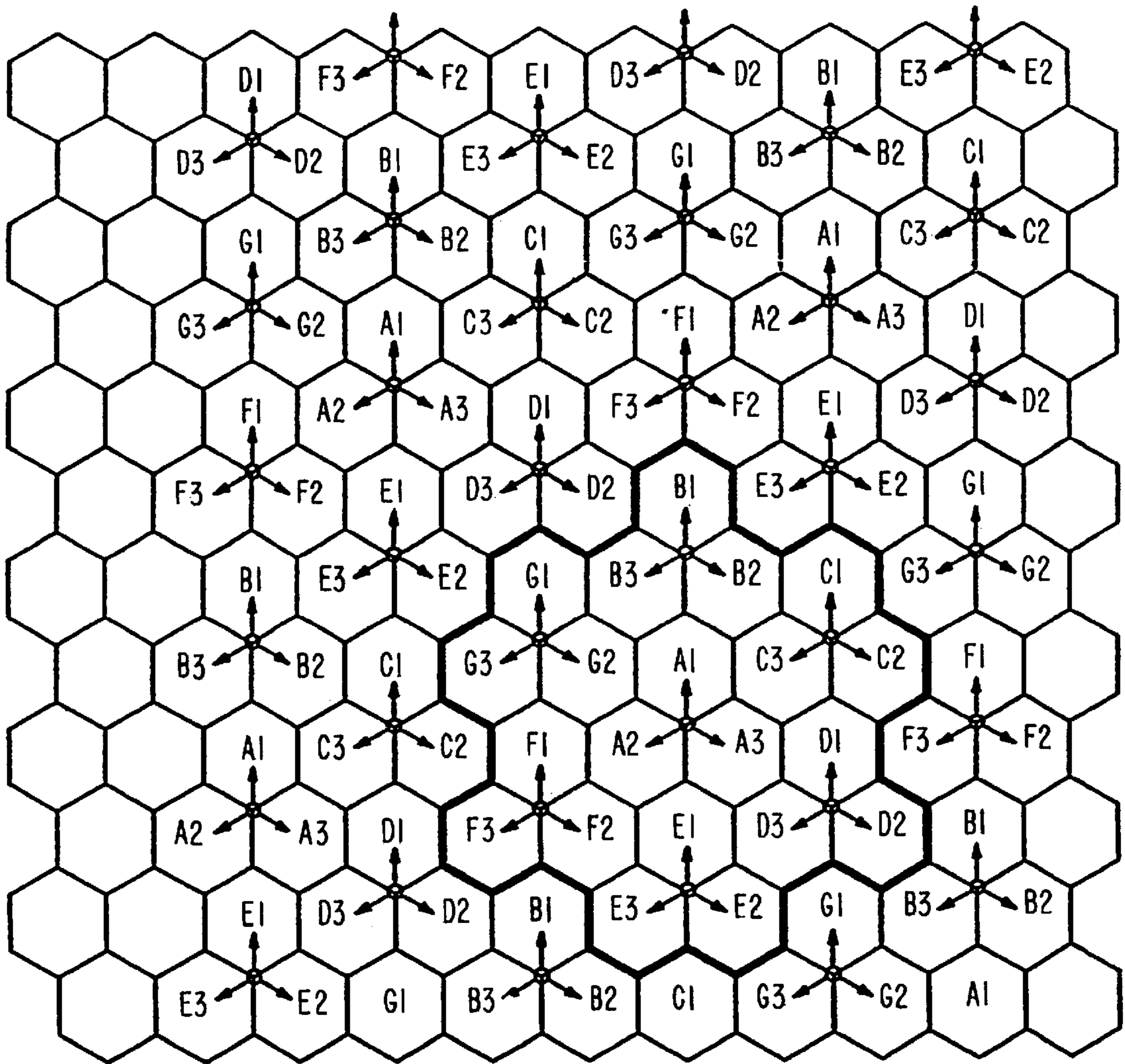
7/21 CELL PATTERN
