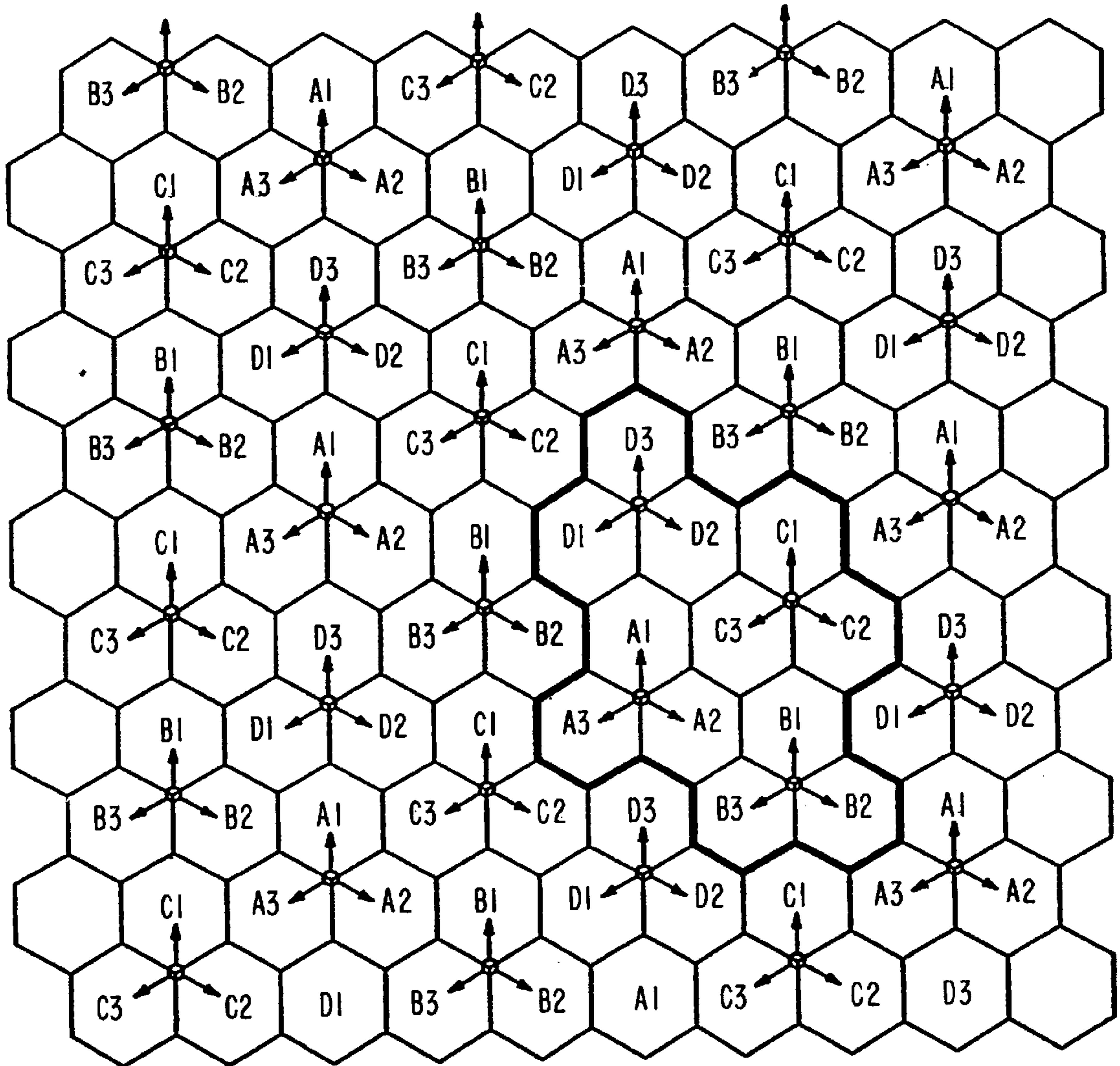
4/12 CELL PATTERN
