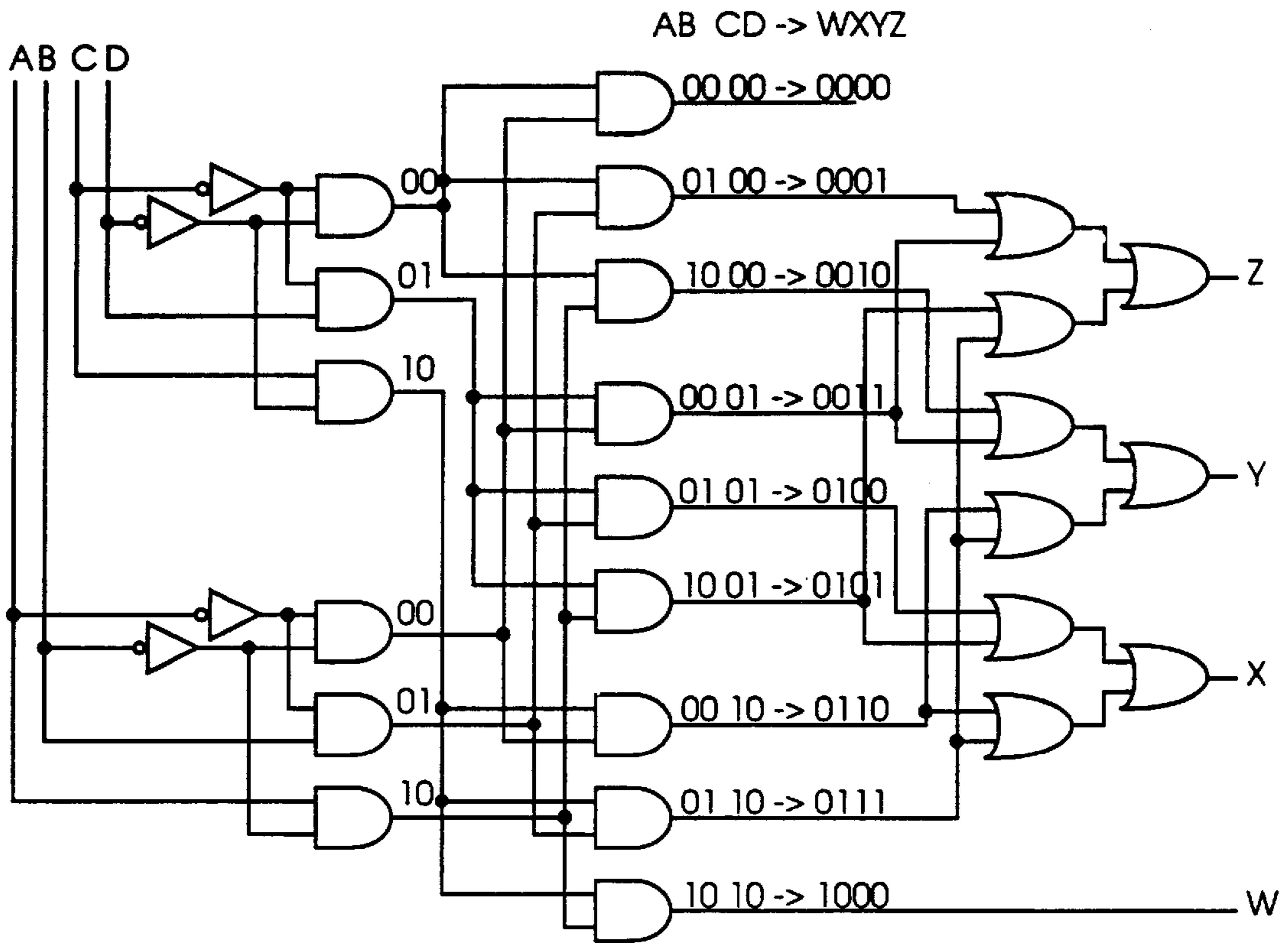
EXAMPLE BINARY REPRESENTATION
