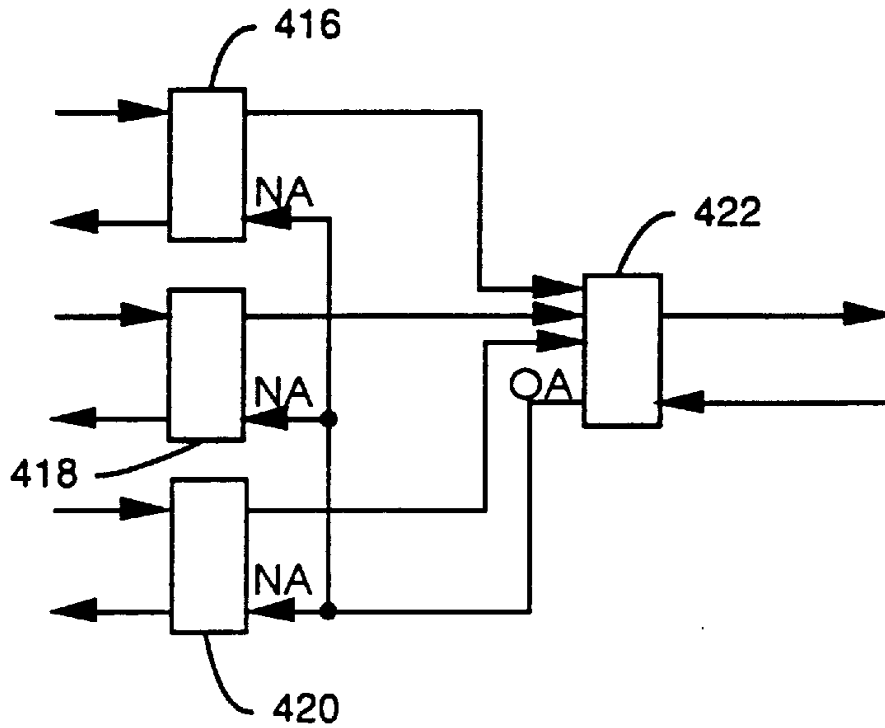
FAN IN CONFIGURATION OF BOUNDARY ELEMENTS
