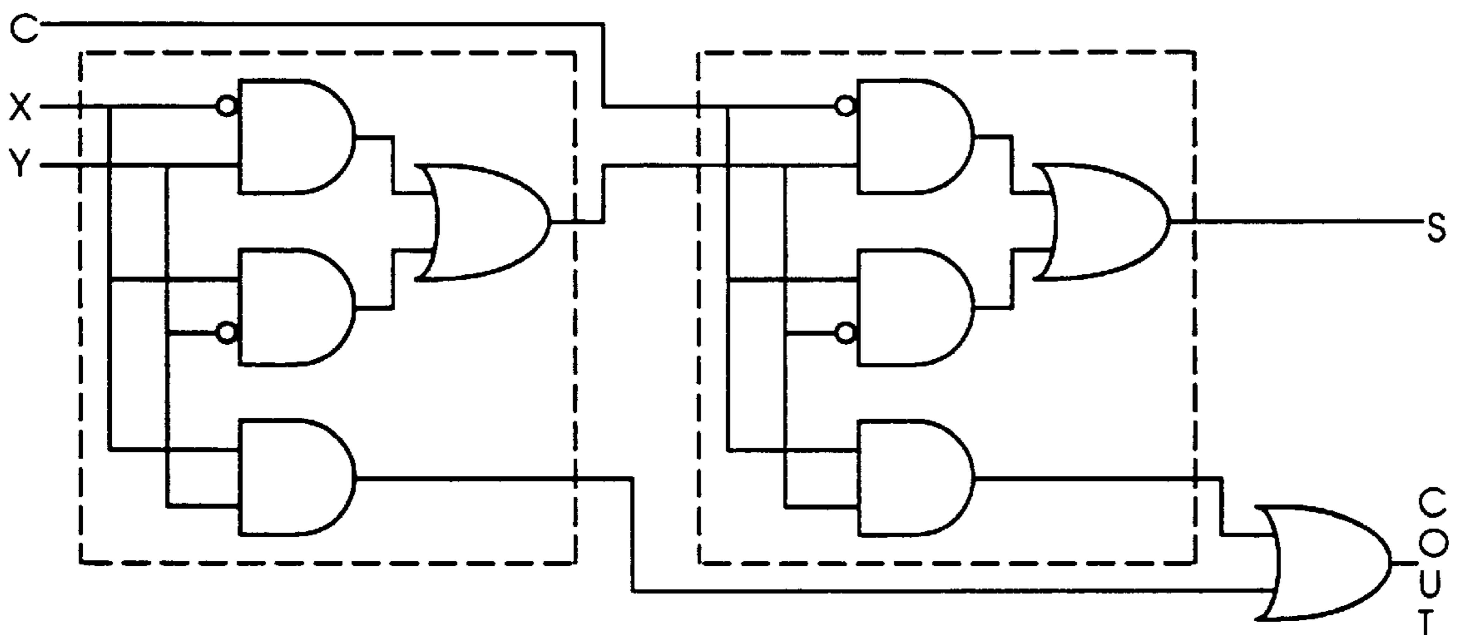
BINARY FULLADDER EXAMPLE EXPRESSION
