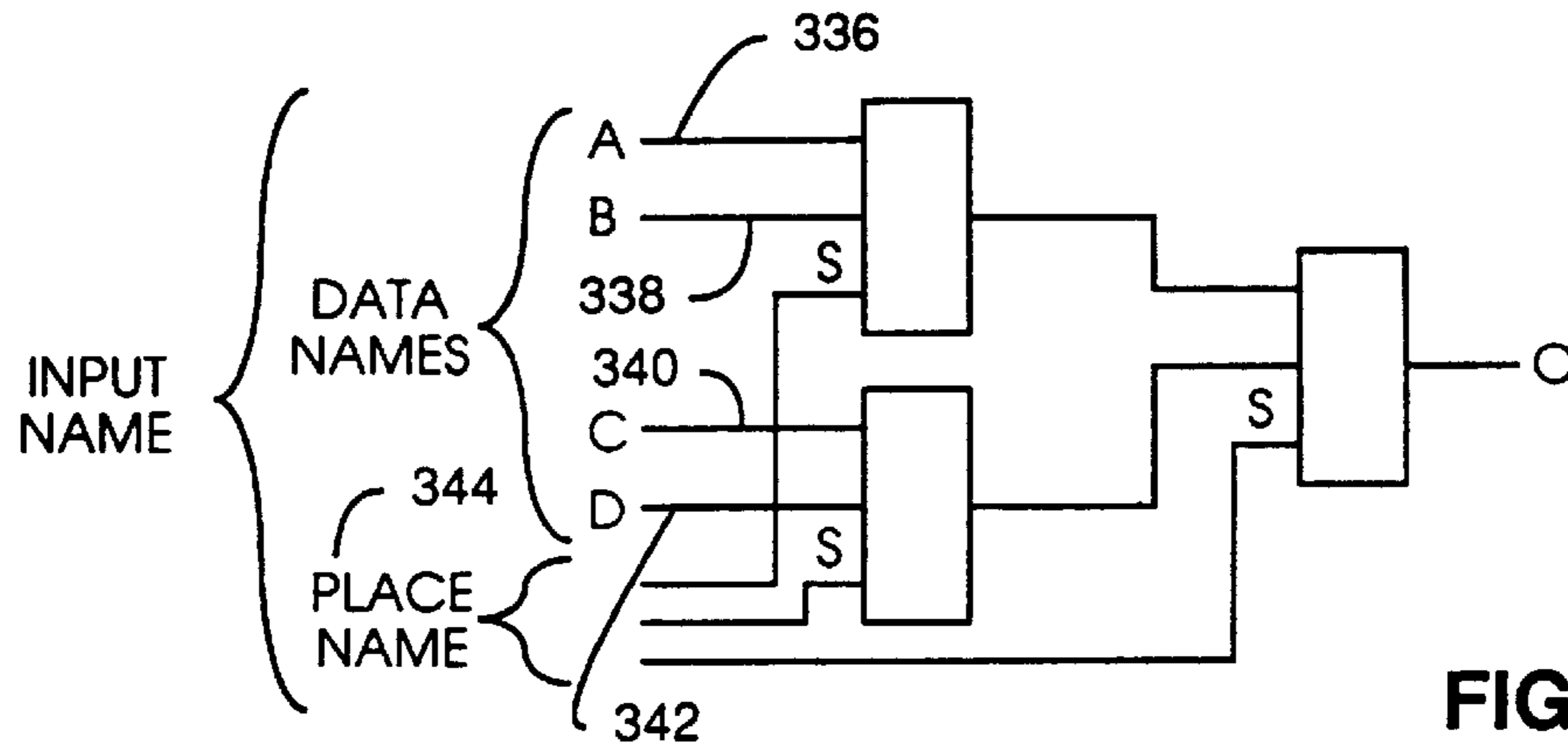
CASCADED SELECTOR TREE
