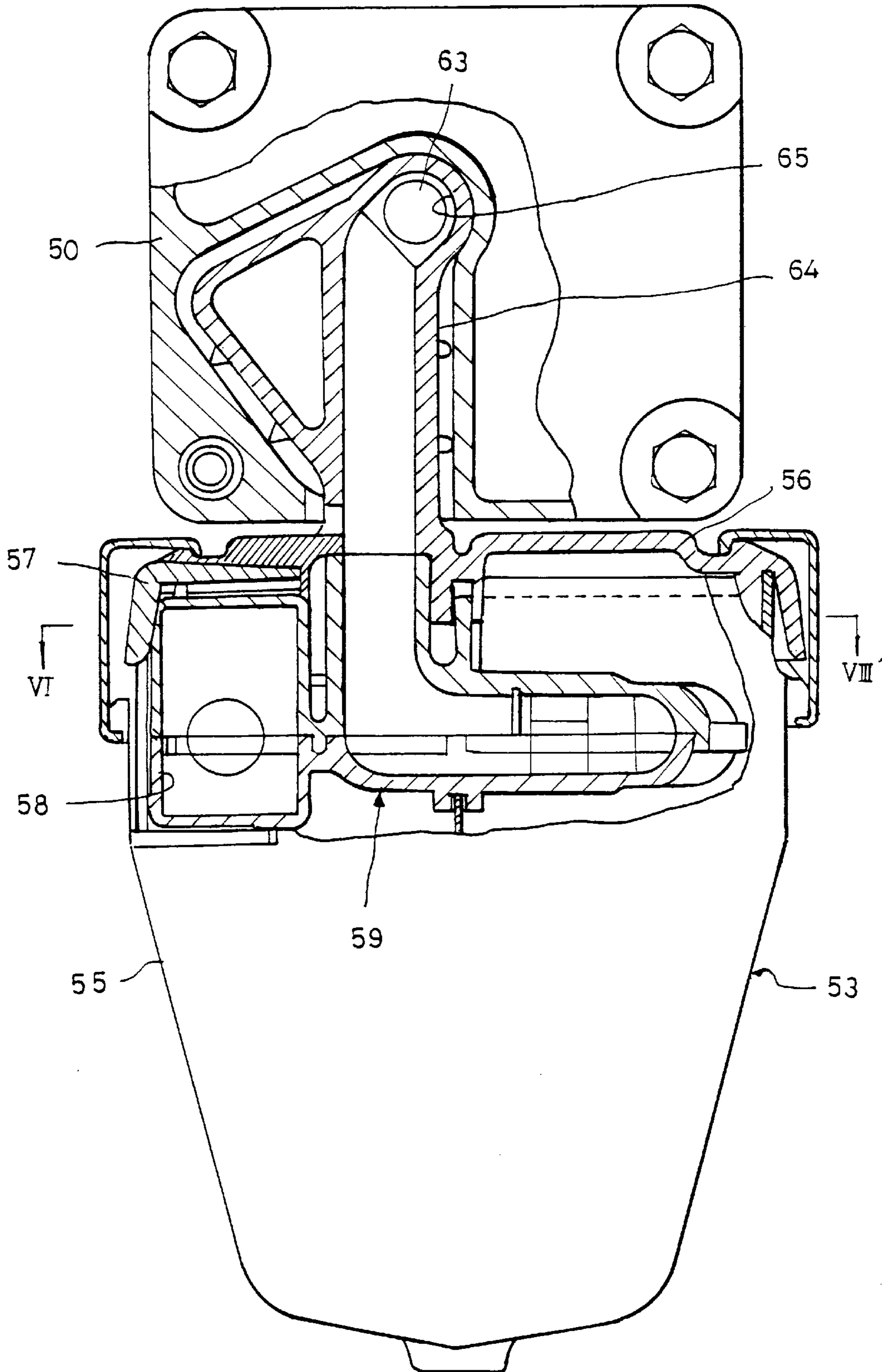
FIG. 7 CONVENTIONAL ART
