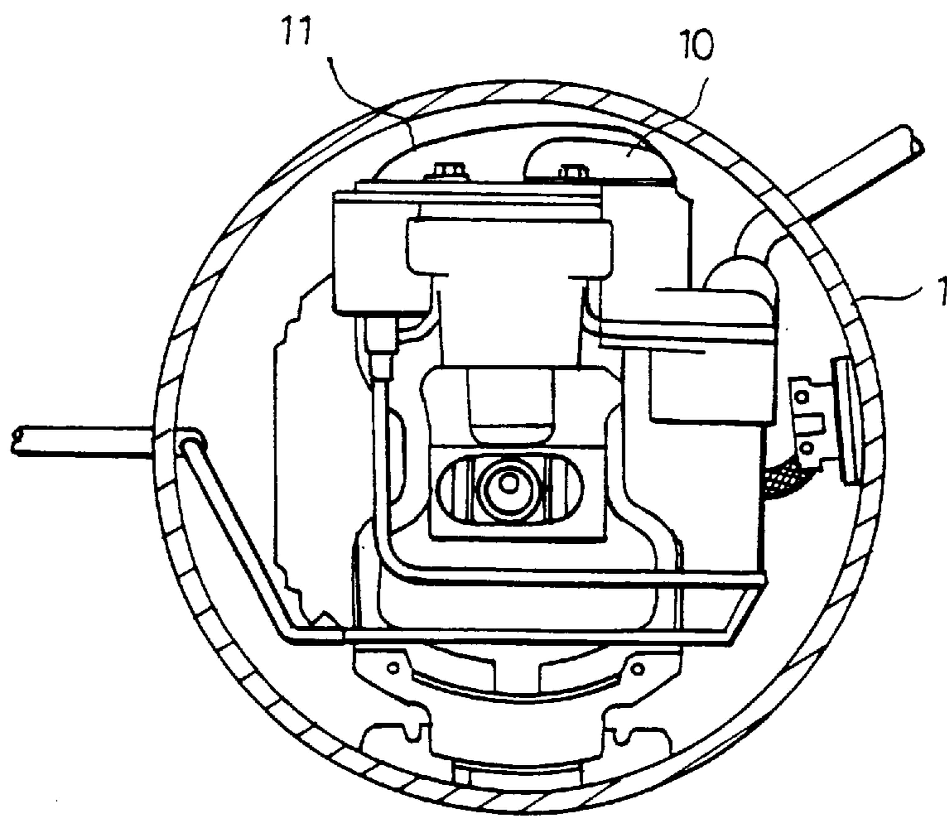
FIG. 2 CONVENTIONAL ART
