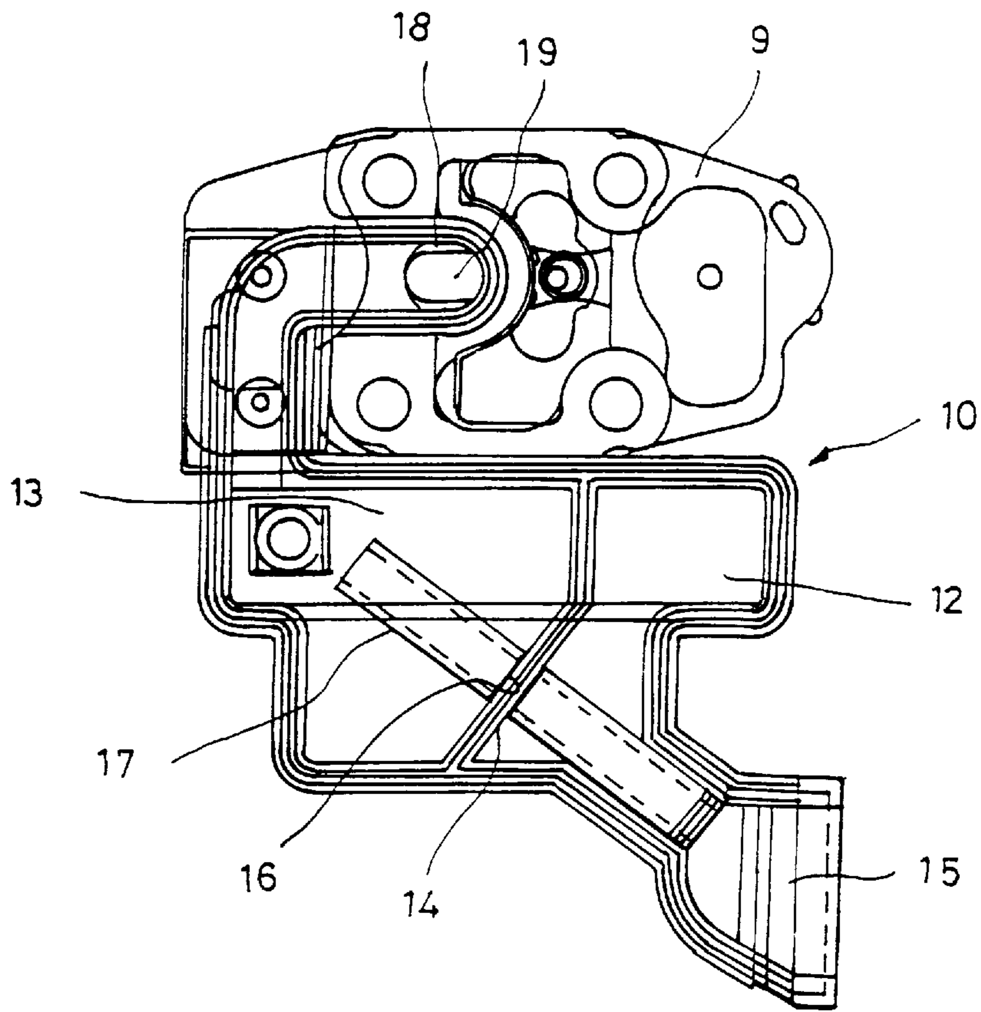
FIG. 3 CONVENTIONAL ART
