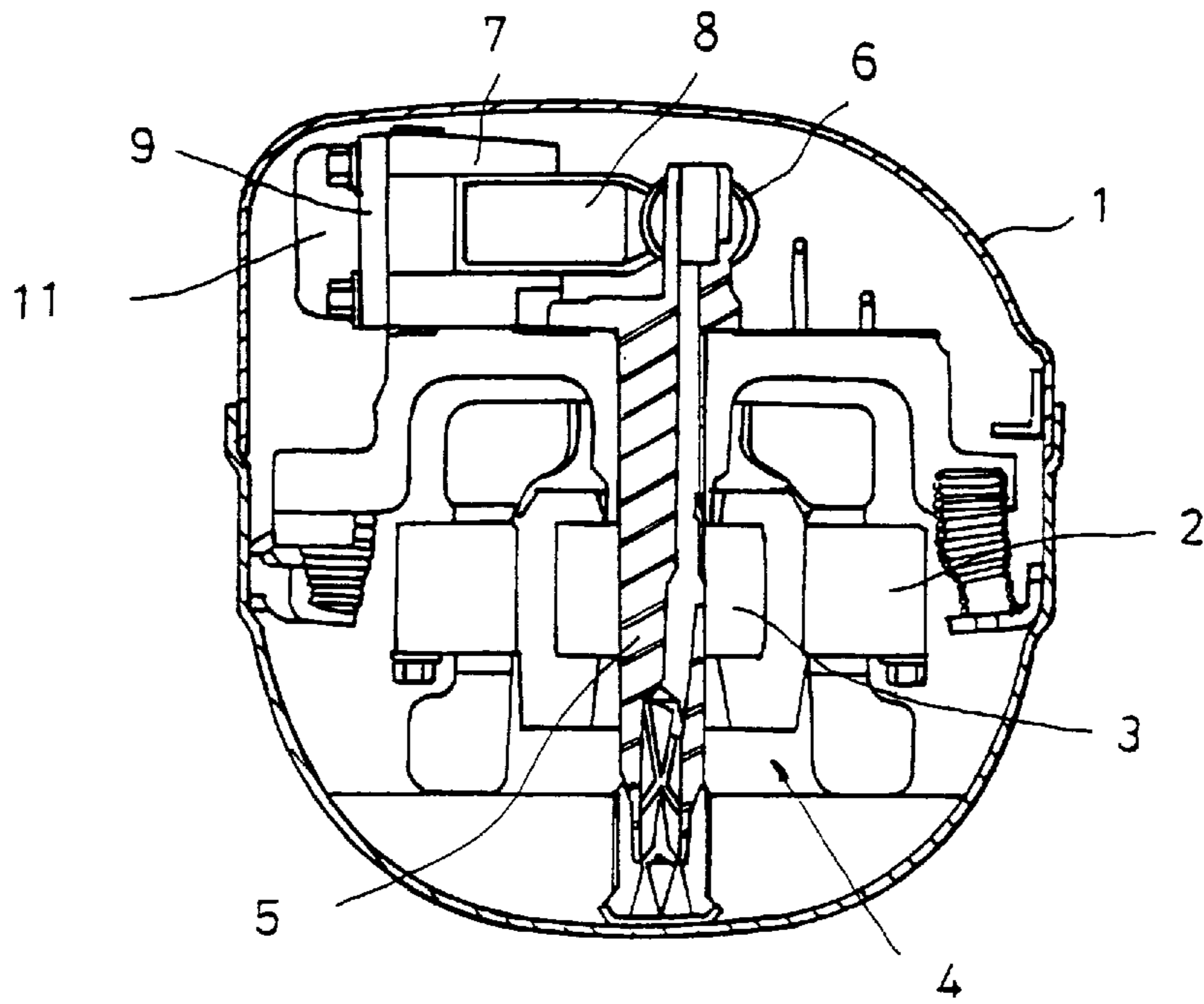
FIG. 1 CONVENTIONAL ART
