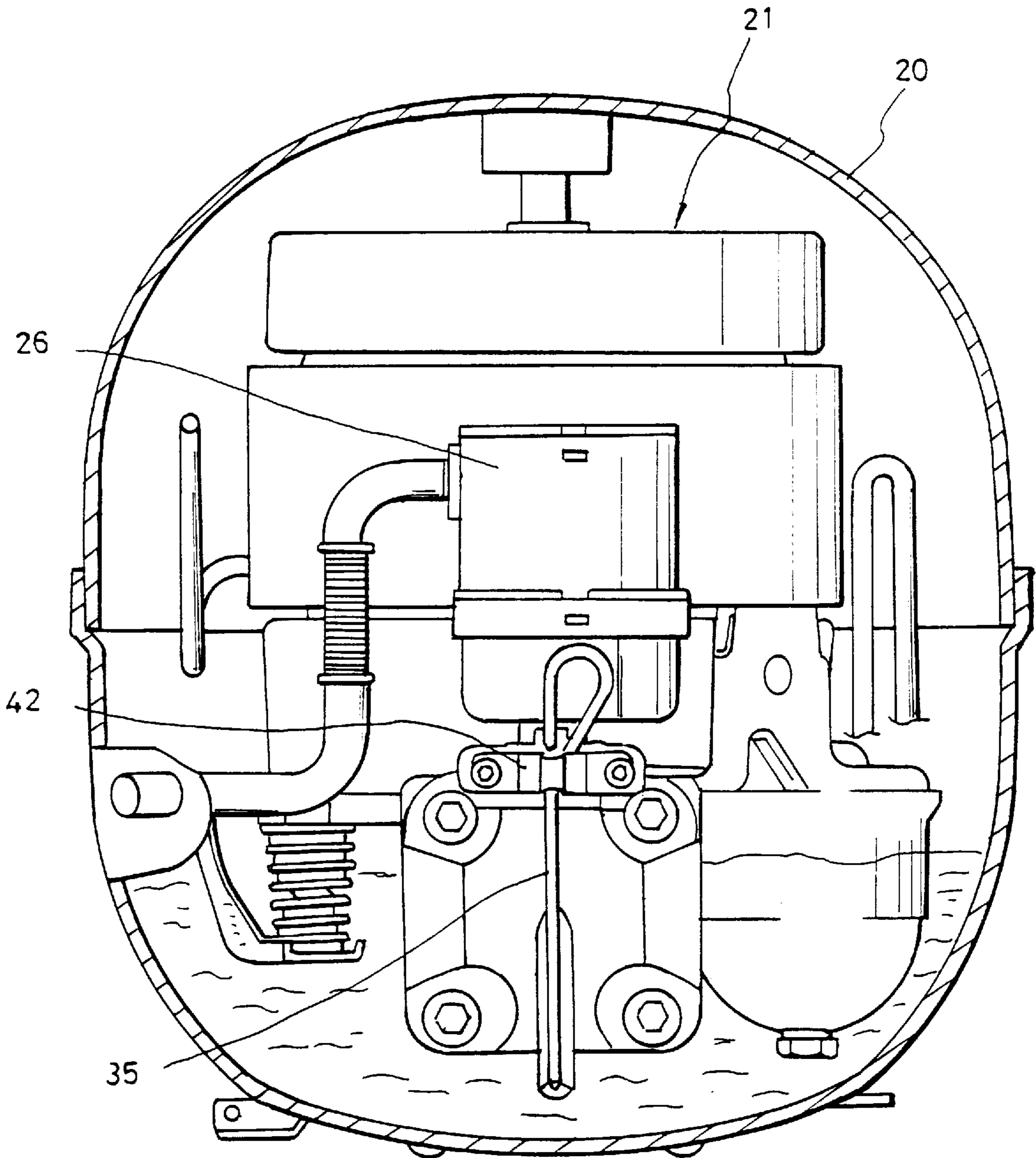
FIG. 4 CONVENTIONAL ART
