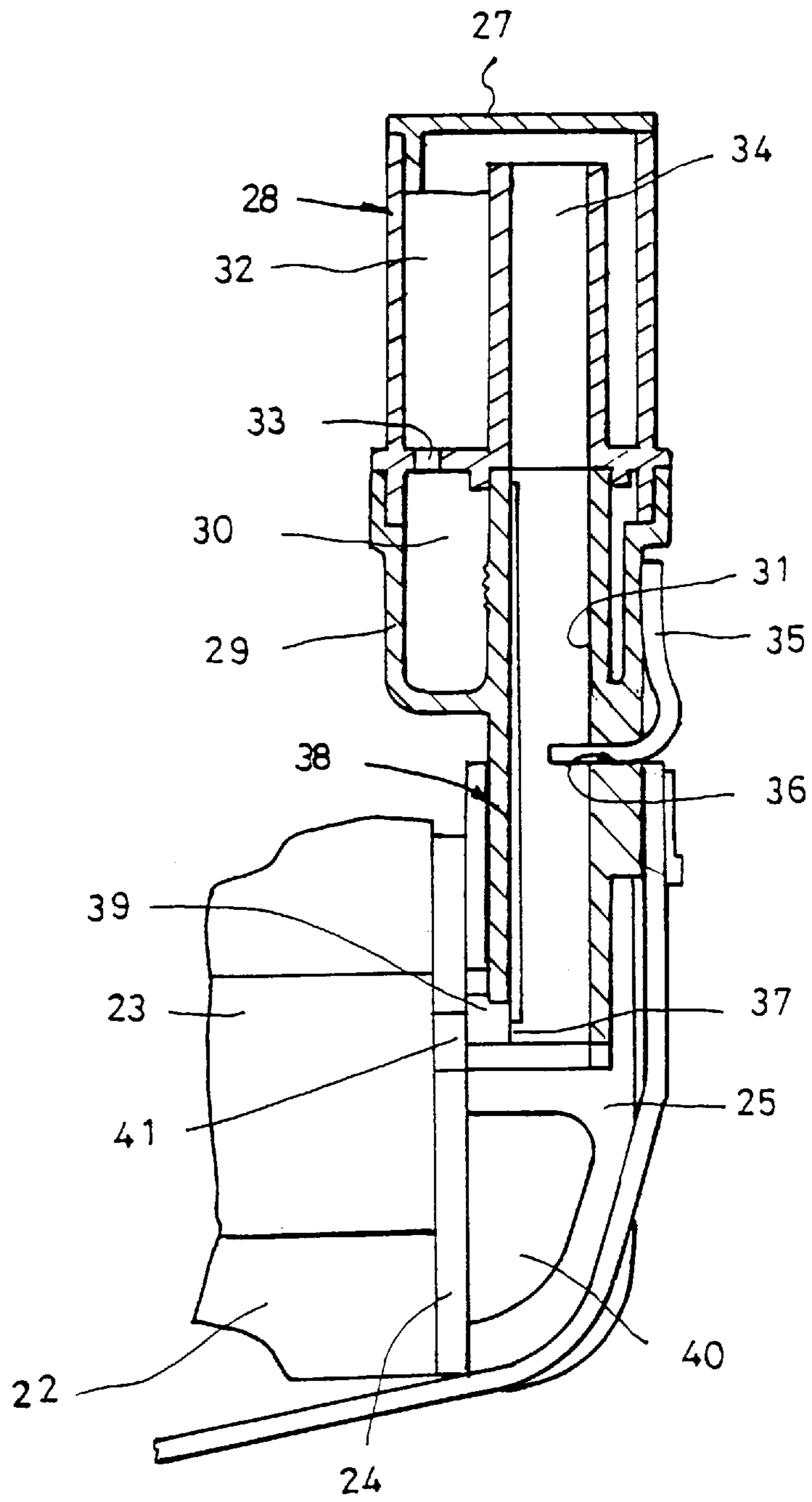
FIG. 5 CONVENTIONAL ART
