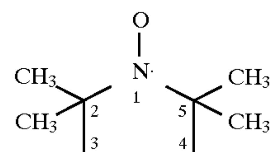
PROXYL (2,2,5,5-Tetramethyl-1-pyrrolidinyl-oxy-) (2,2,5,5-Tetramethylpyrrolidine-N-oxy)
