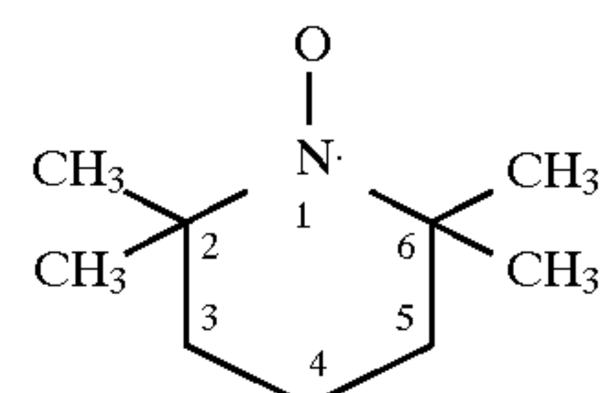
TEMPO (2,2,6,6-Tetramethyl-1-piperidinyl-oxy-) (2,2,6,6-Tetramethylpiperidine-N-oxy)
