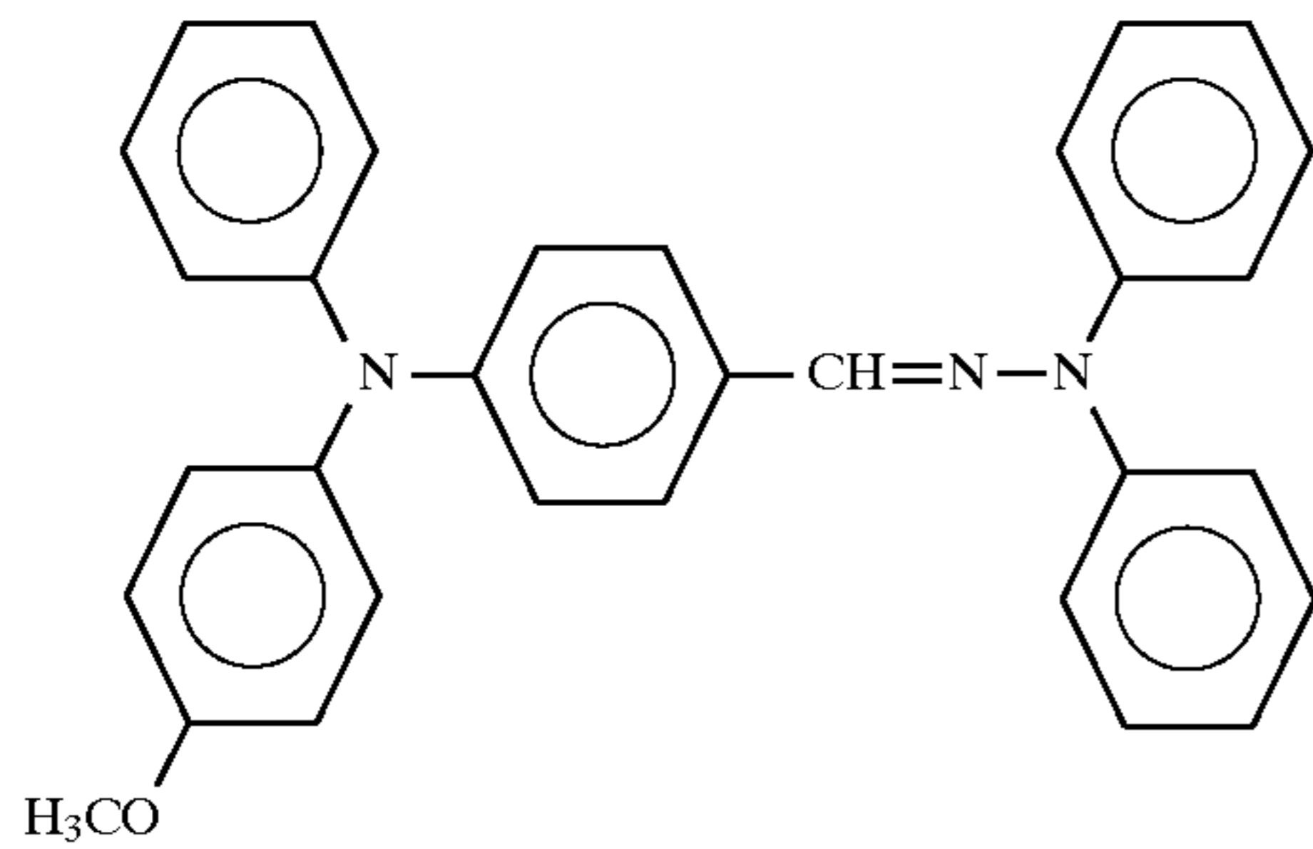
Comparative Example 4
