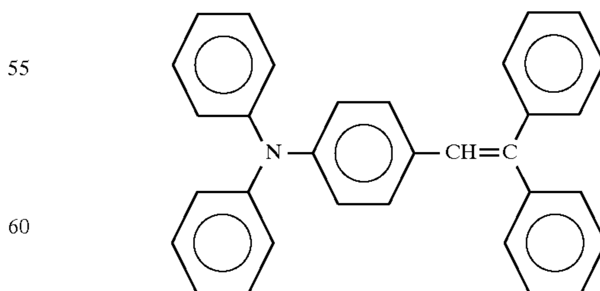
Comparative Compound 7
