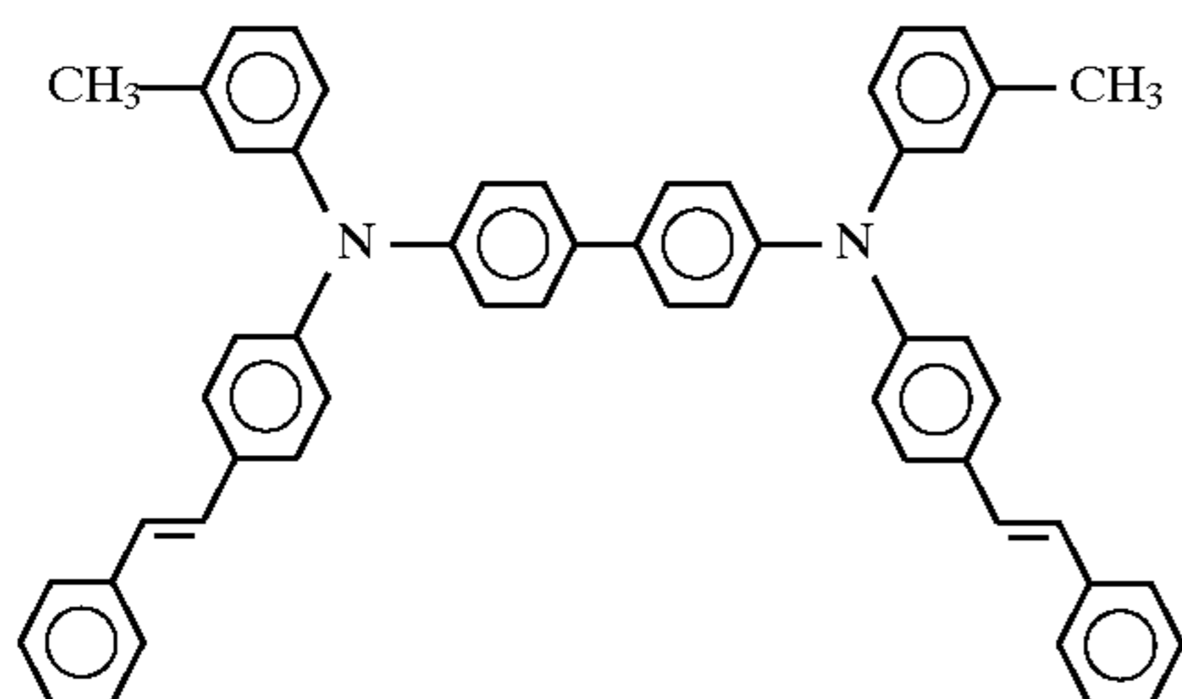
Comparative Compound 4
