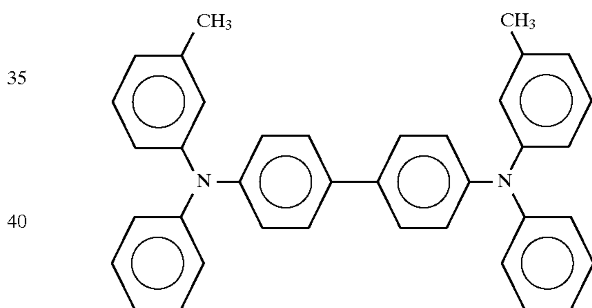
Comparative Compound 6
