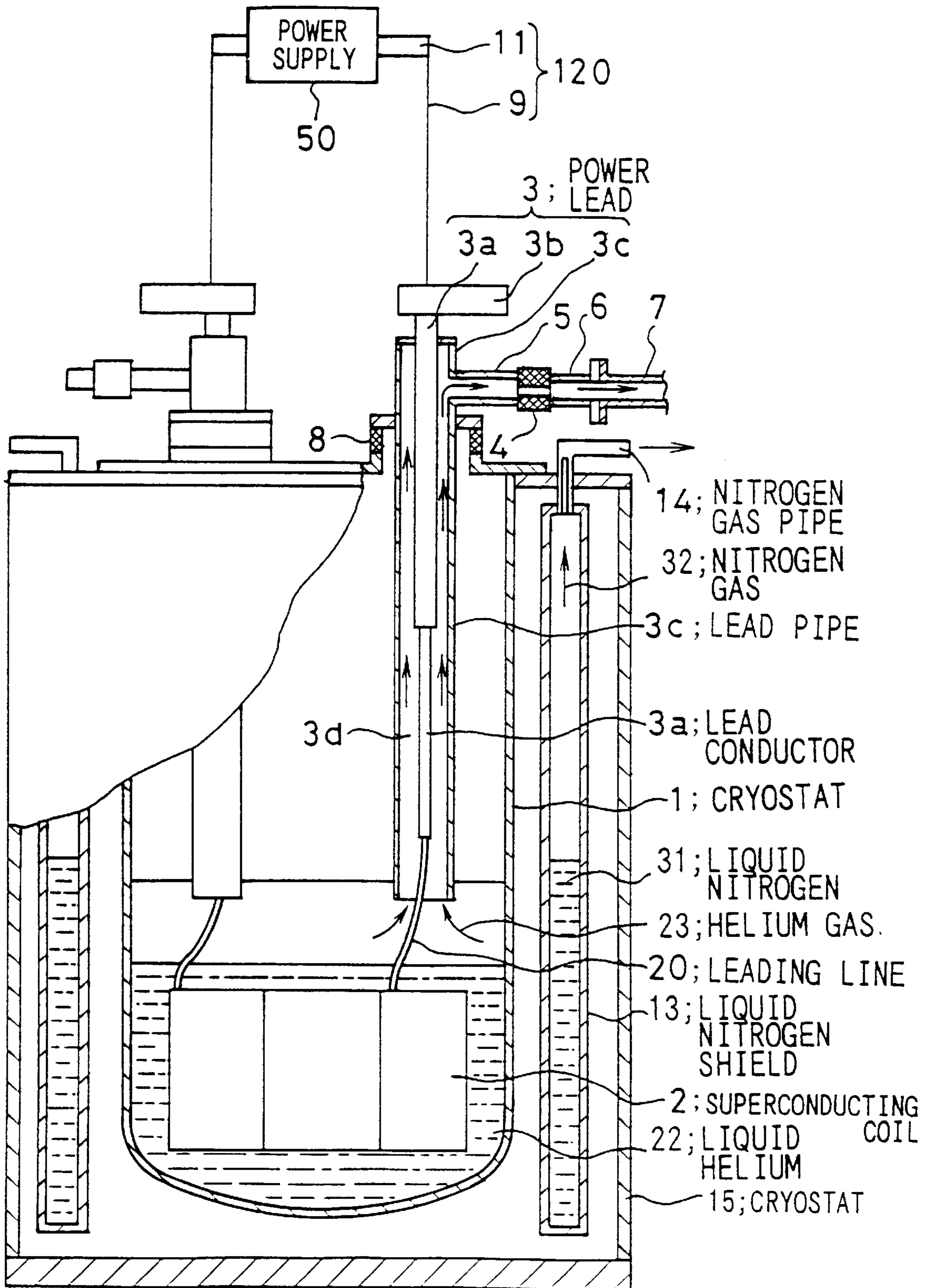
FIG. 16 PRIOR ART
