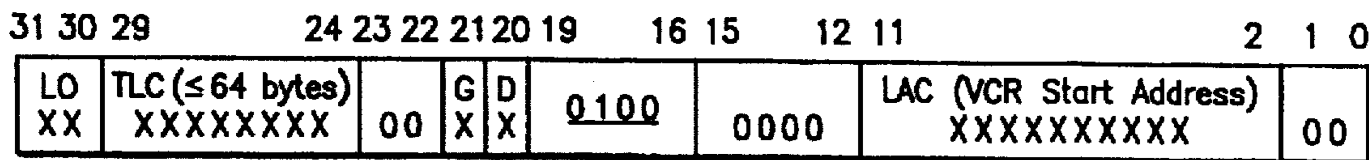
Effective Address Field Settings for Write to DMA Control Registers/Counters
