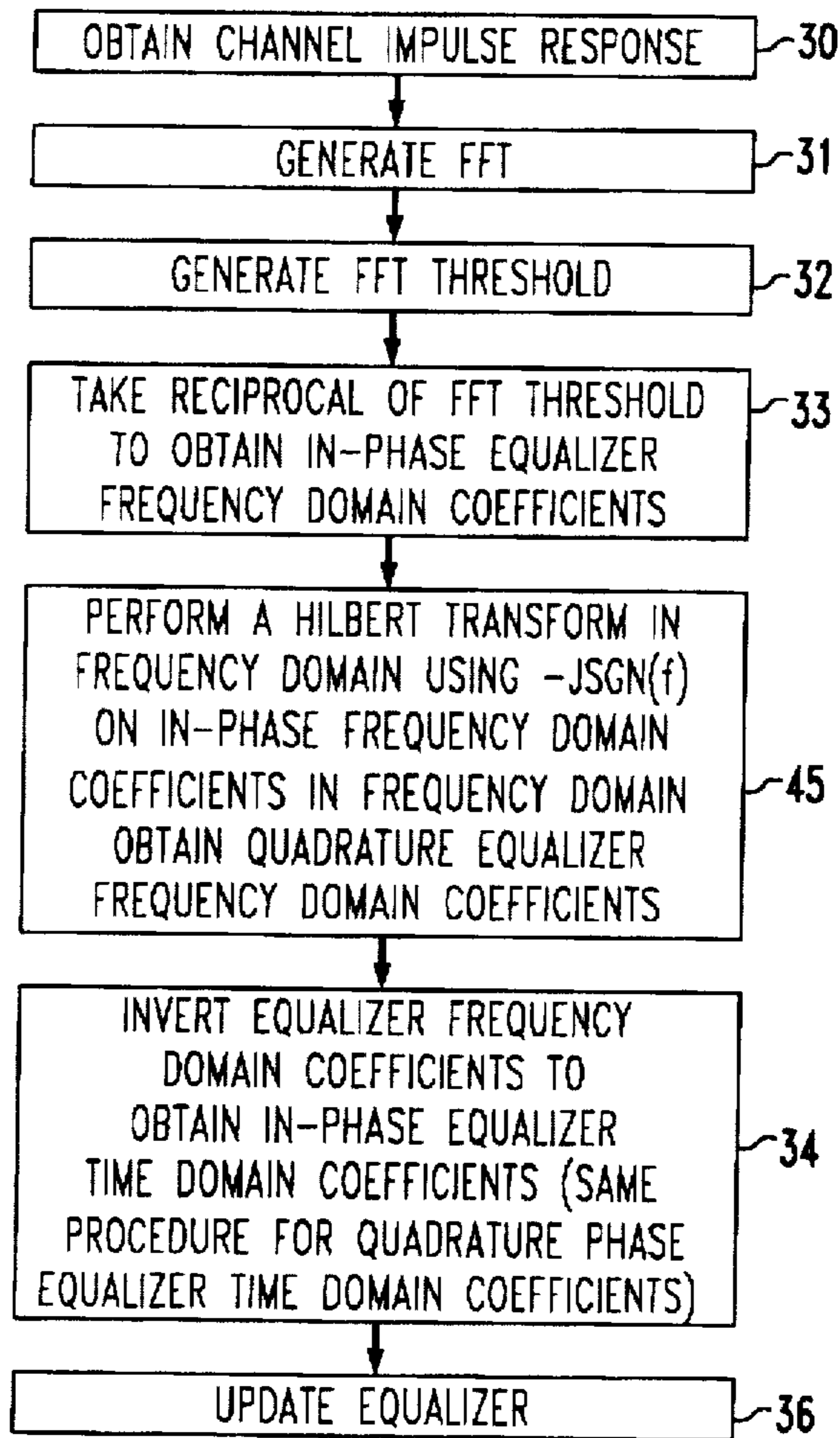
FIG. 16 CHANNEL SOUNDING PROCESS
