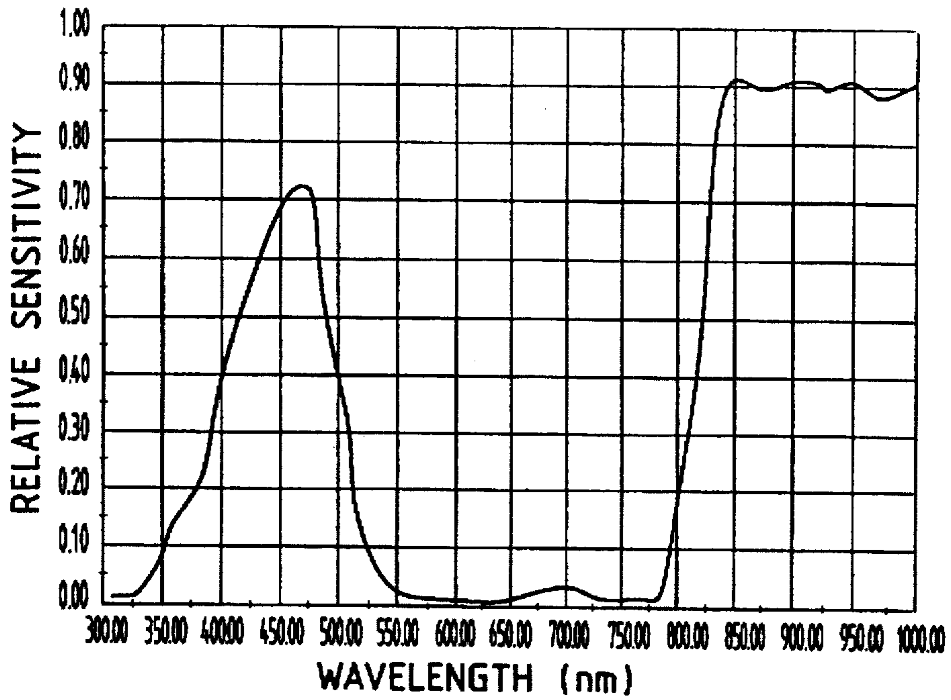
B-FILTER SPECTRUM PROPERTY
