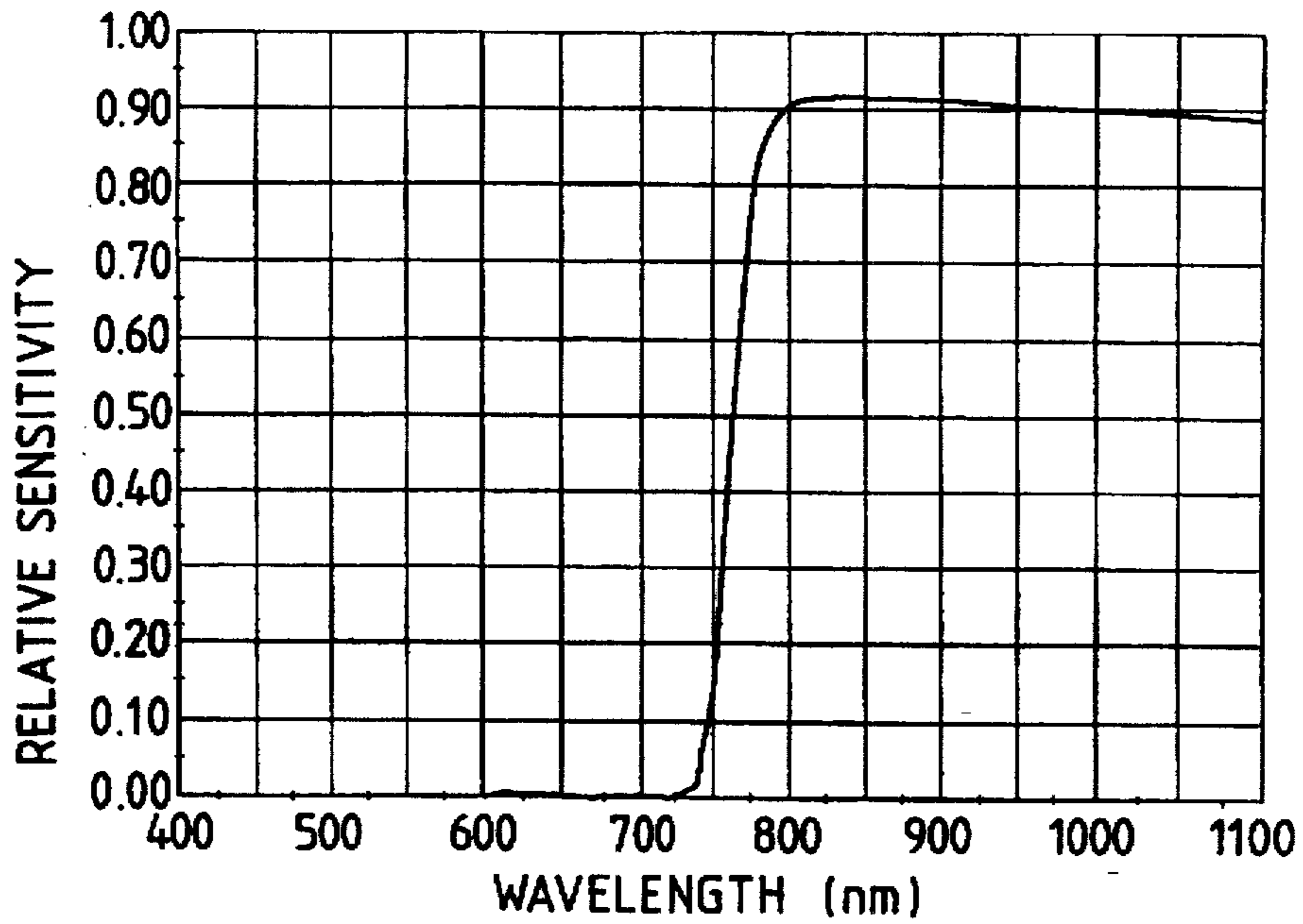
VISIBLE LIGHT CUT FILTER SPECTRUM PROPERTY
