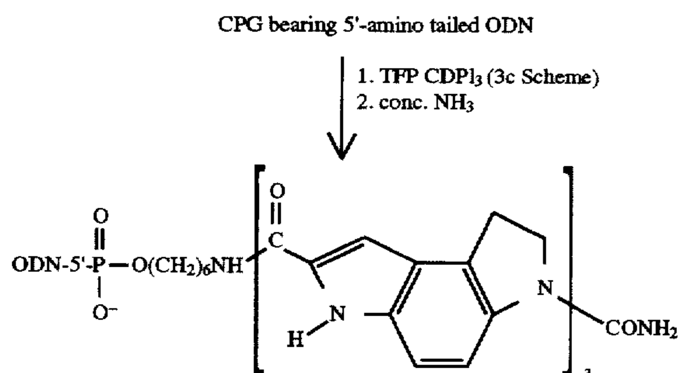
Reaction Scheme 4
