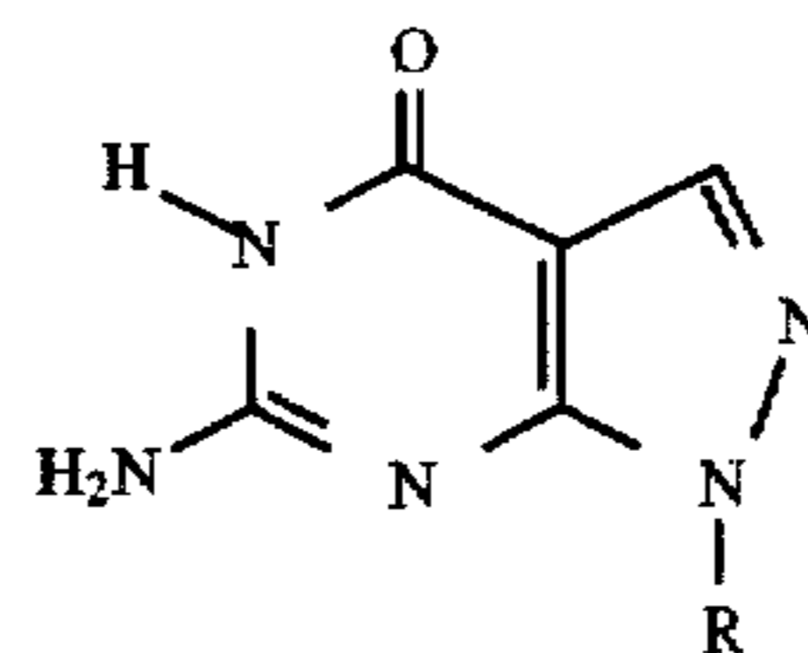
6-amino-4-hydroxypyrazolo-[3,4-d]pyrimidine 2-deoxyriboside R = 2-deoxy-β-D-ribofuranosyl
