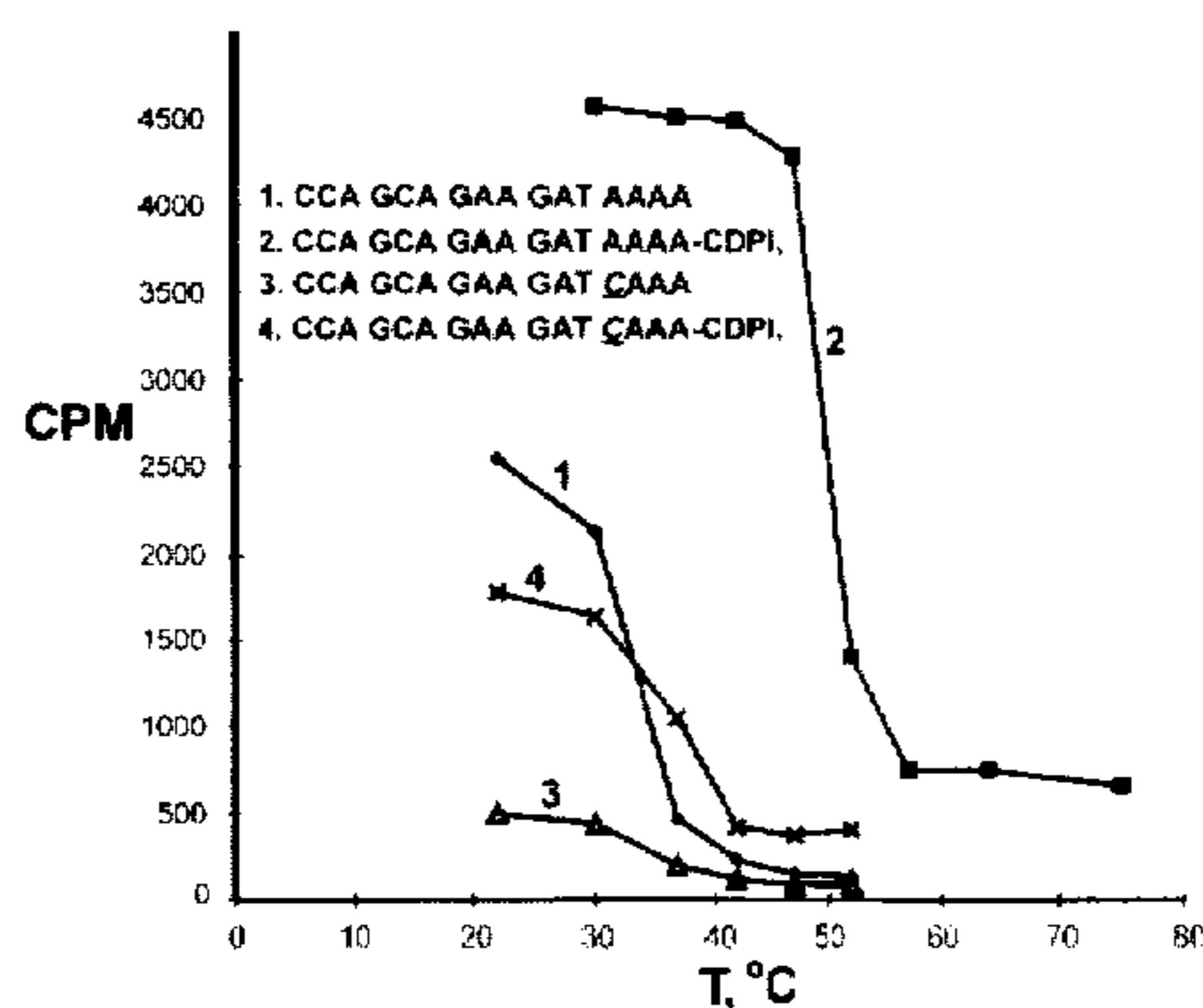
Figure 1: Slot blot hybridization of unmodified ODN or 3'-ODN-CDPI conjugates to M13mp19 (+) strand DNA. Underlined nucleotides represent mismatches with the targeted plasmid sequence.
