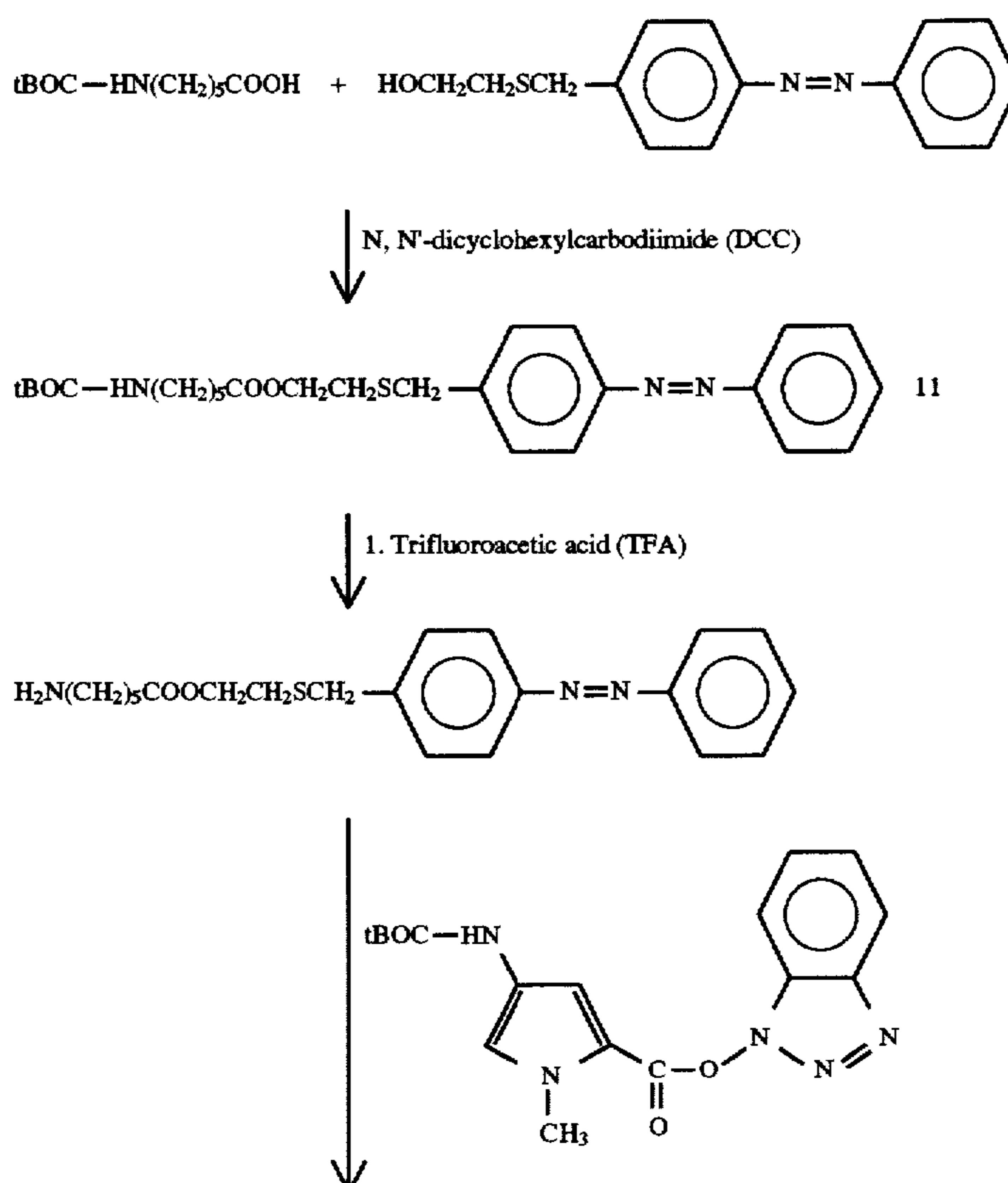
Reaction Scheme 2
