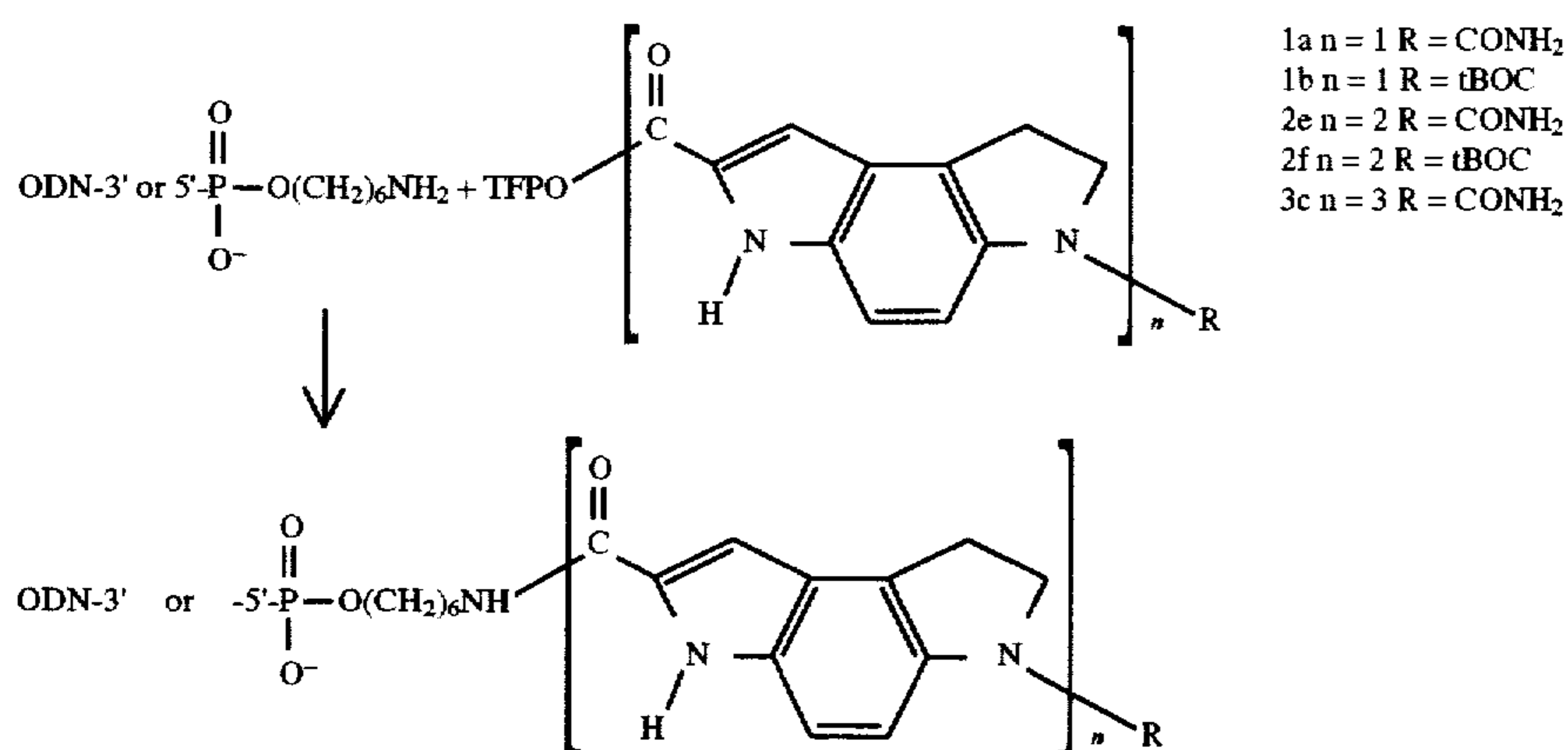
Reaction Scheme 3
