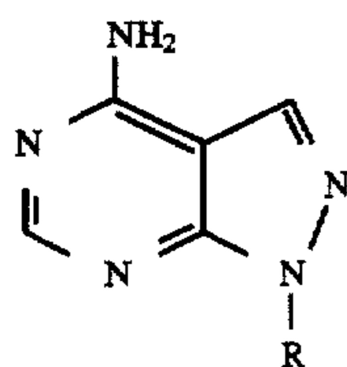
4-aminopyrazolo[3,4-d]pyrimidine 2-deoxyriboside
