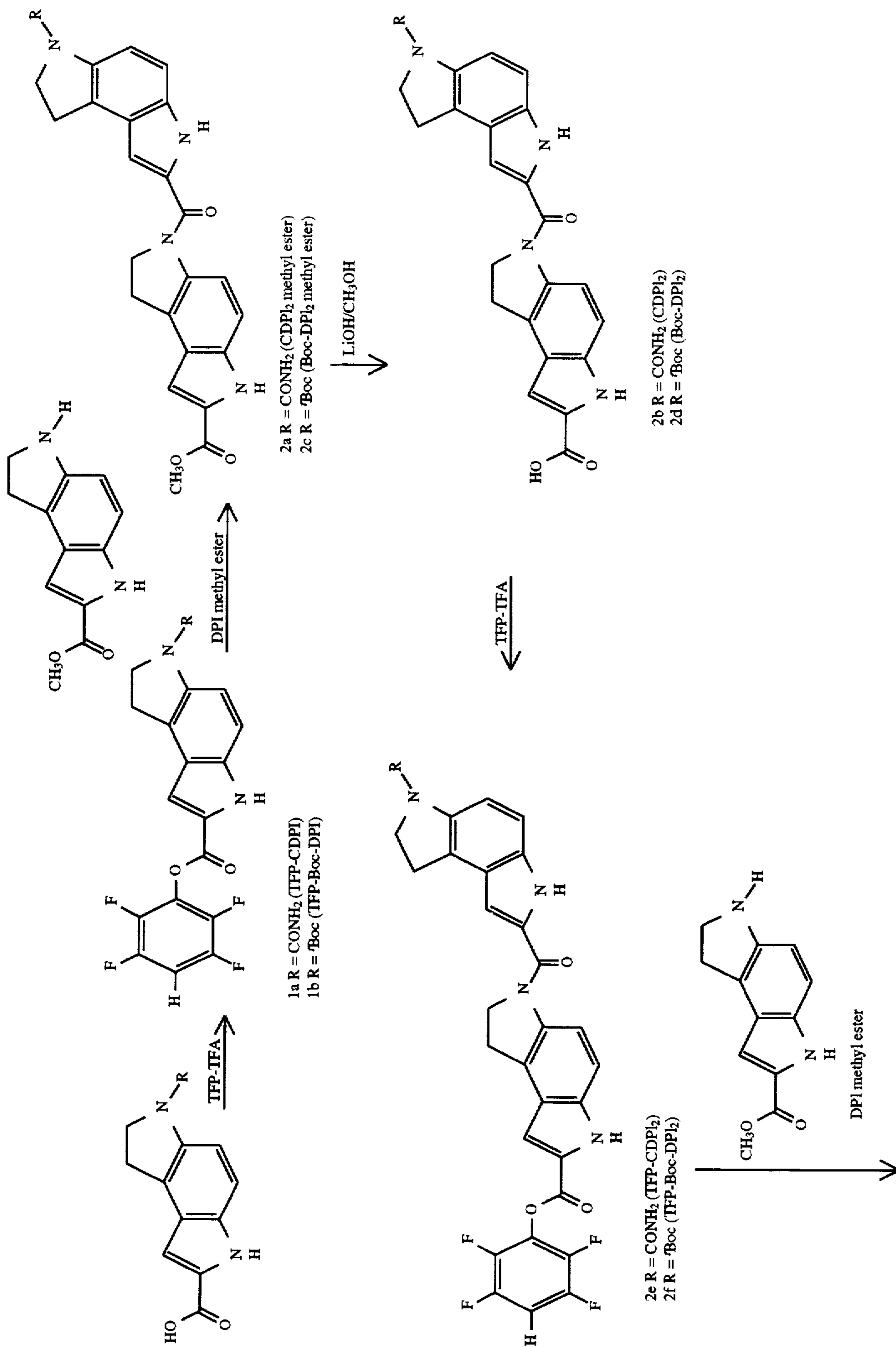
Reaction Scheme 1
