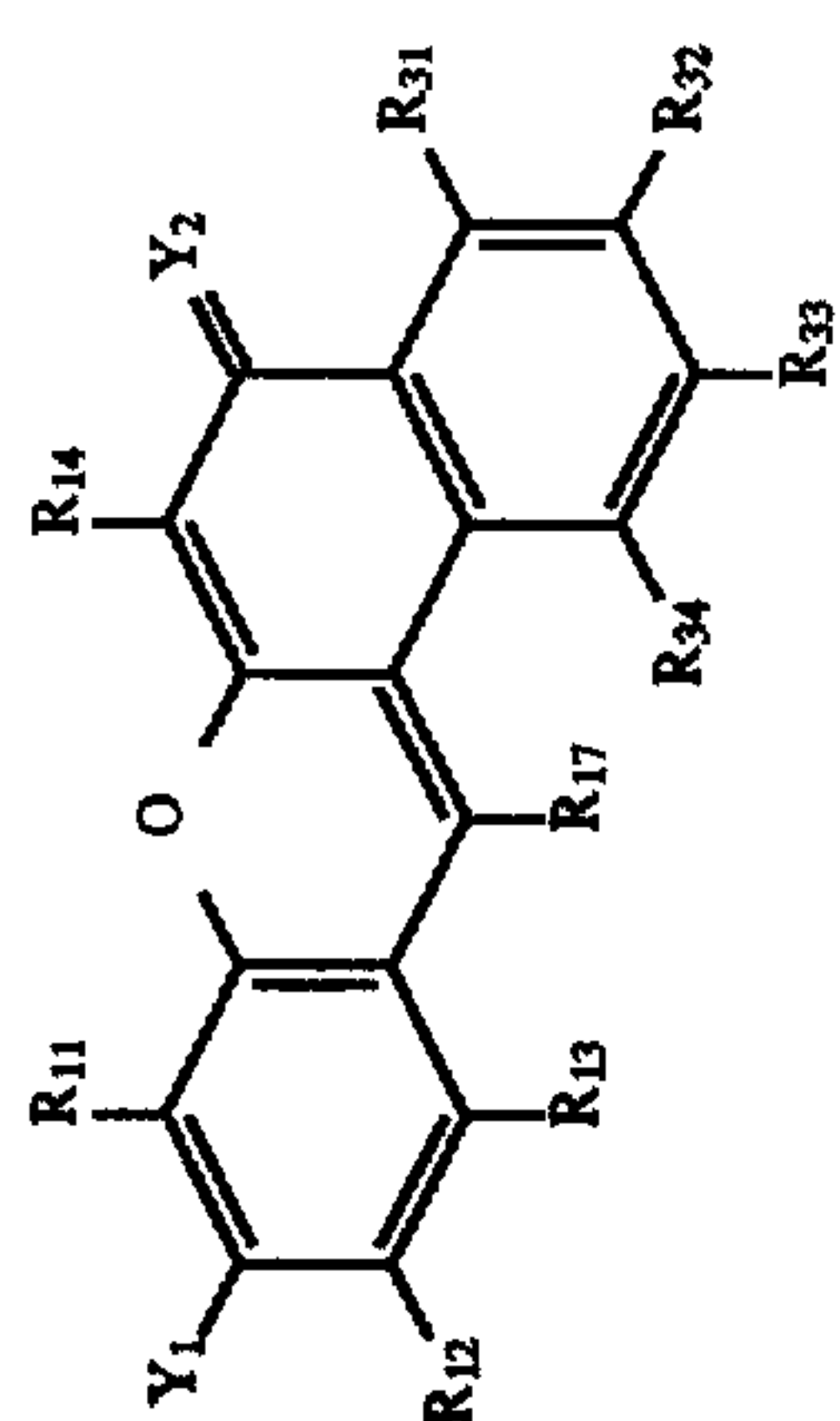
ASYMMETRIC BENZOXANTHENE DYES
