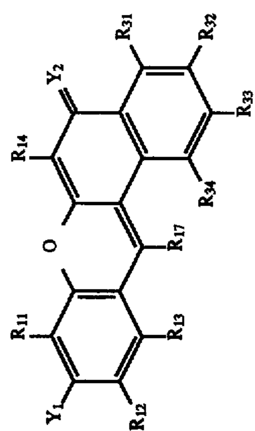
ASYMMETRIC BENZOXANTHENE DYES
