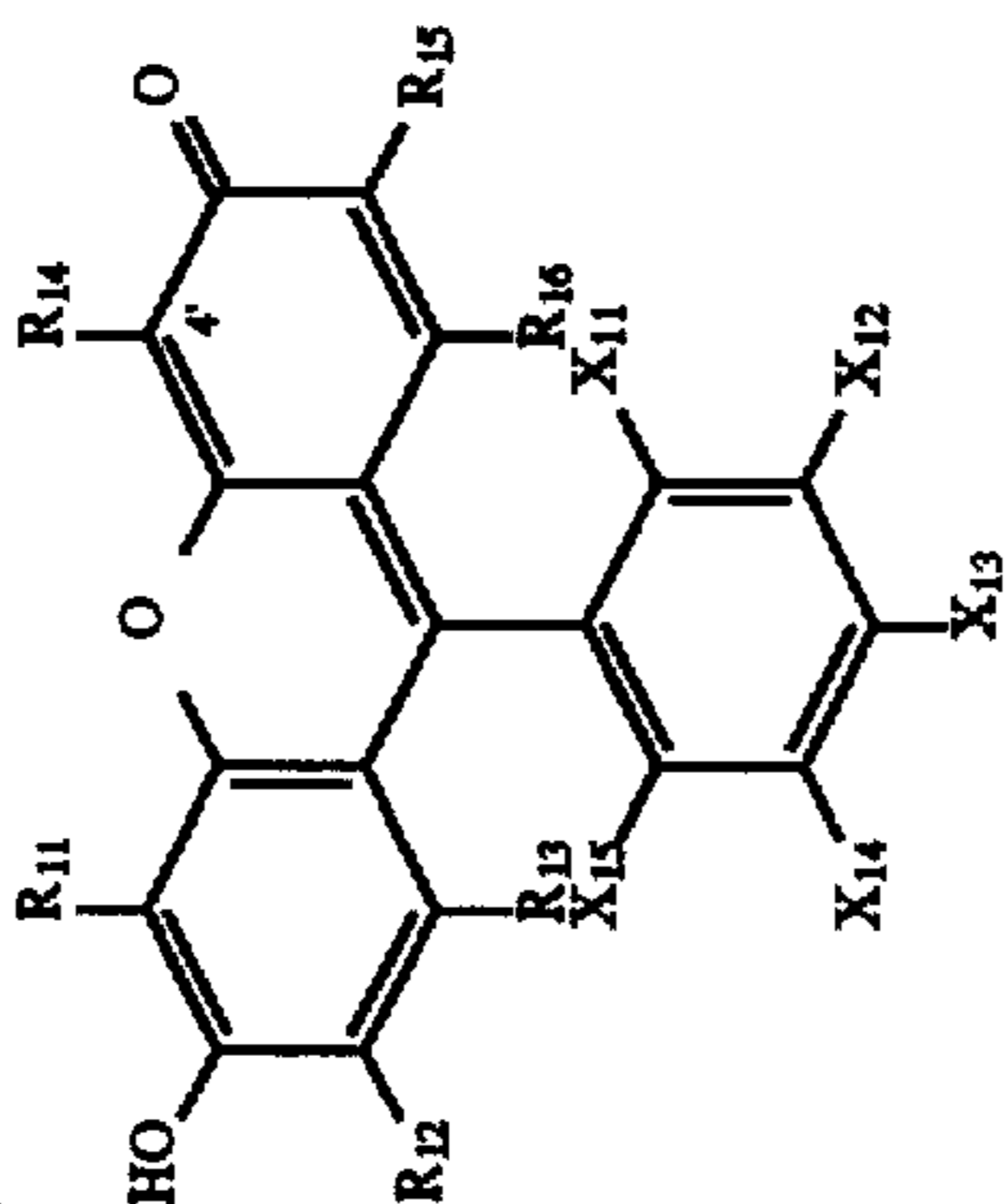
FLUORESCHEIN
