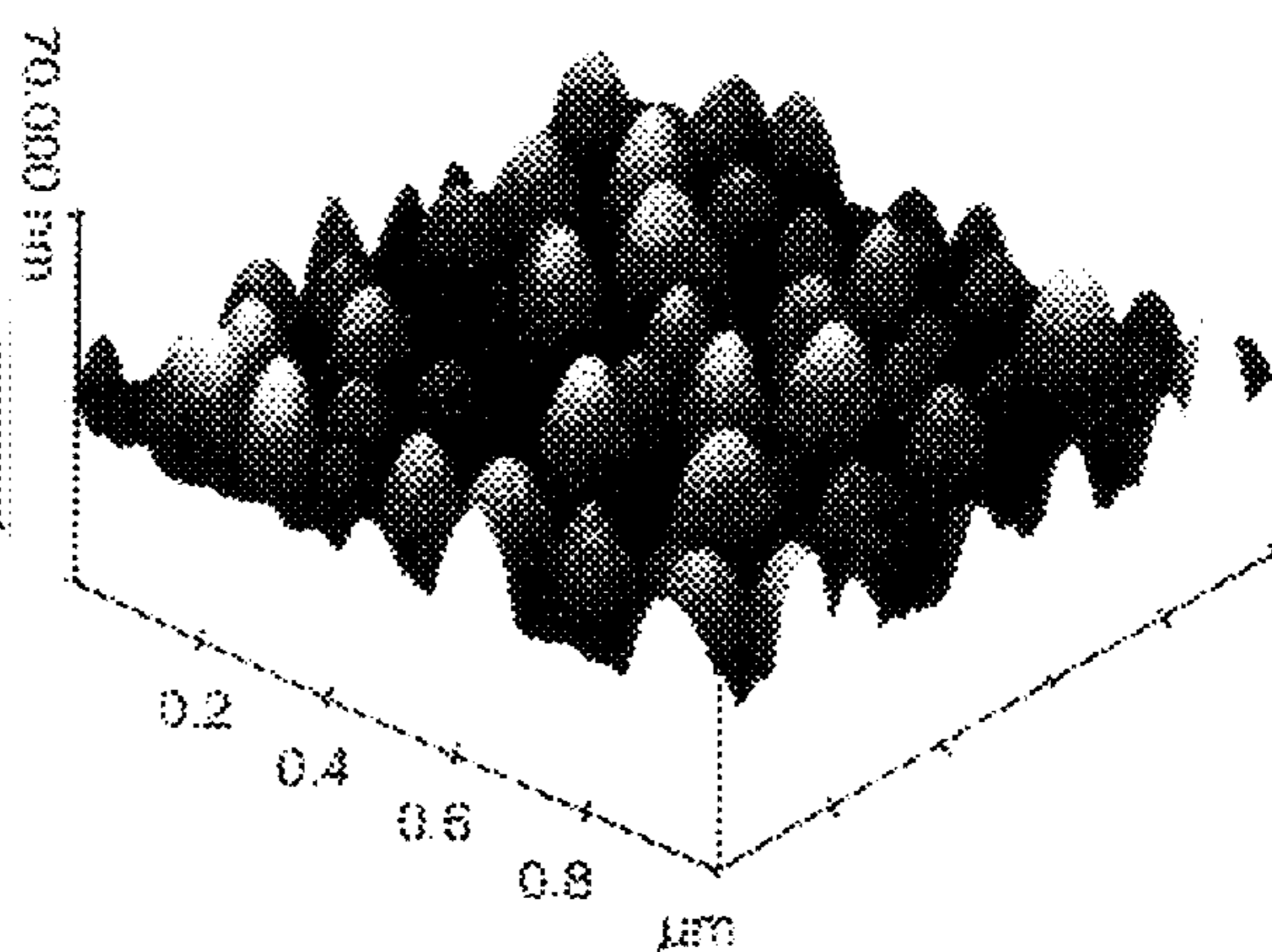
NiAl, 100nm/ MgO, 20nm/ glass
