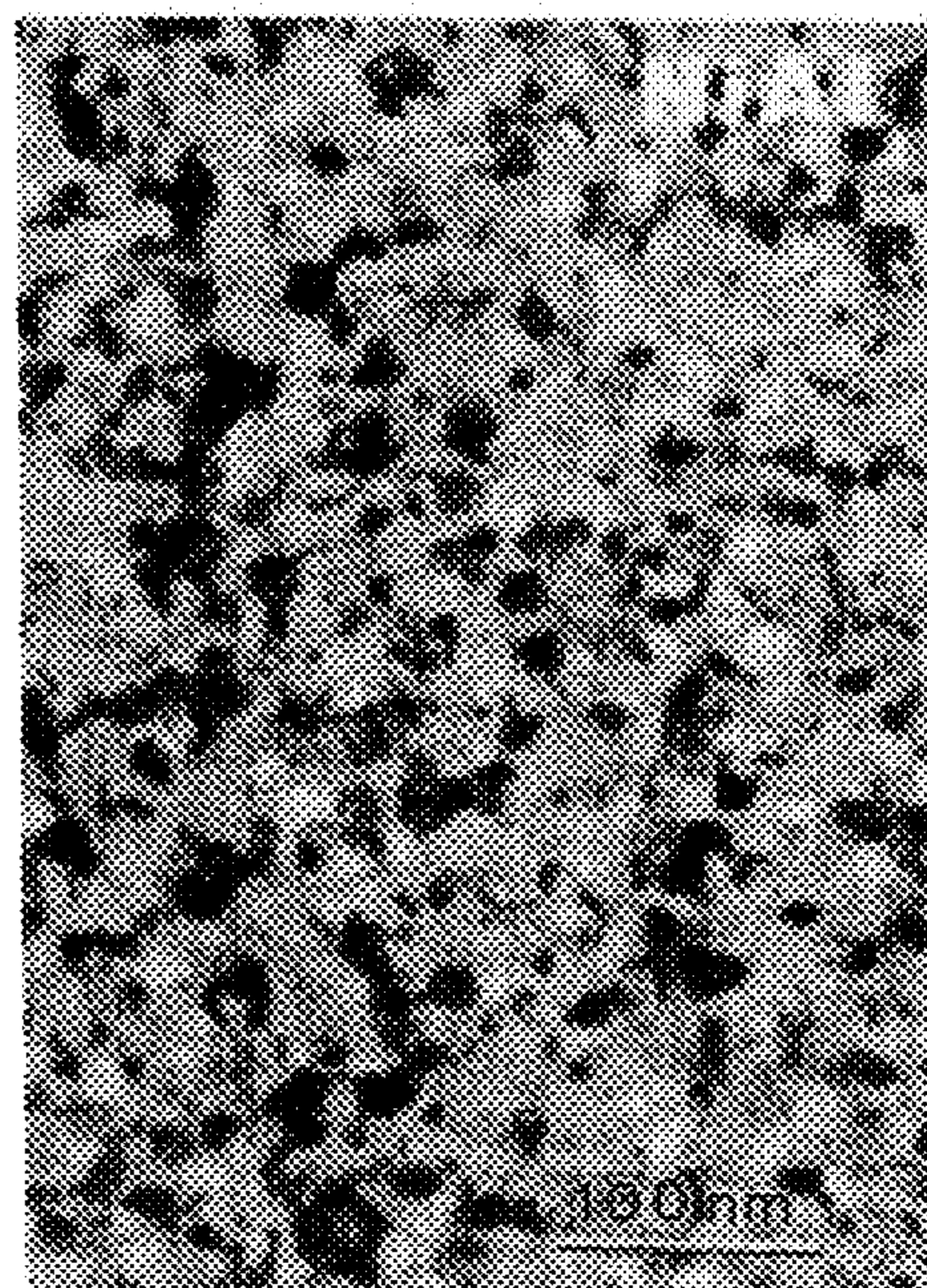
FIG. 3(a) NiAl
