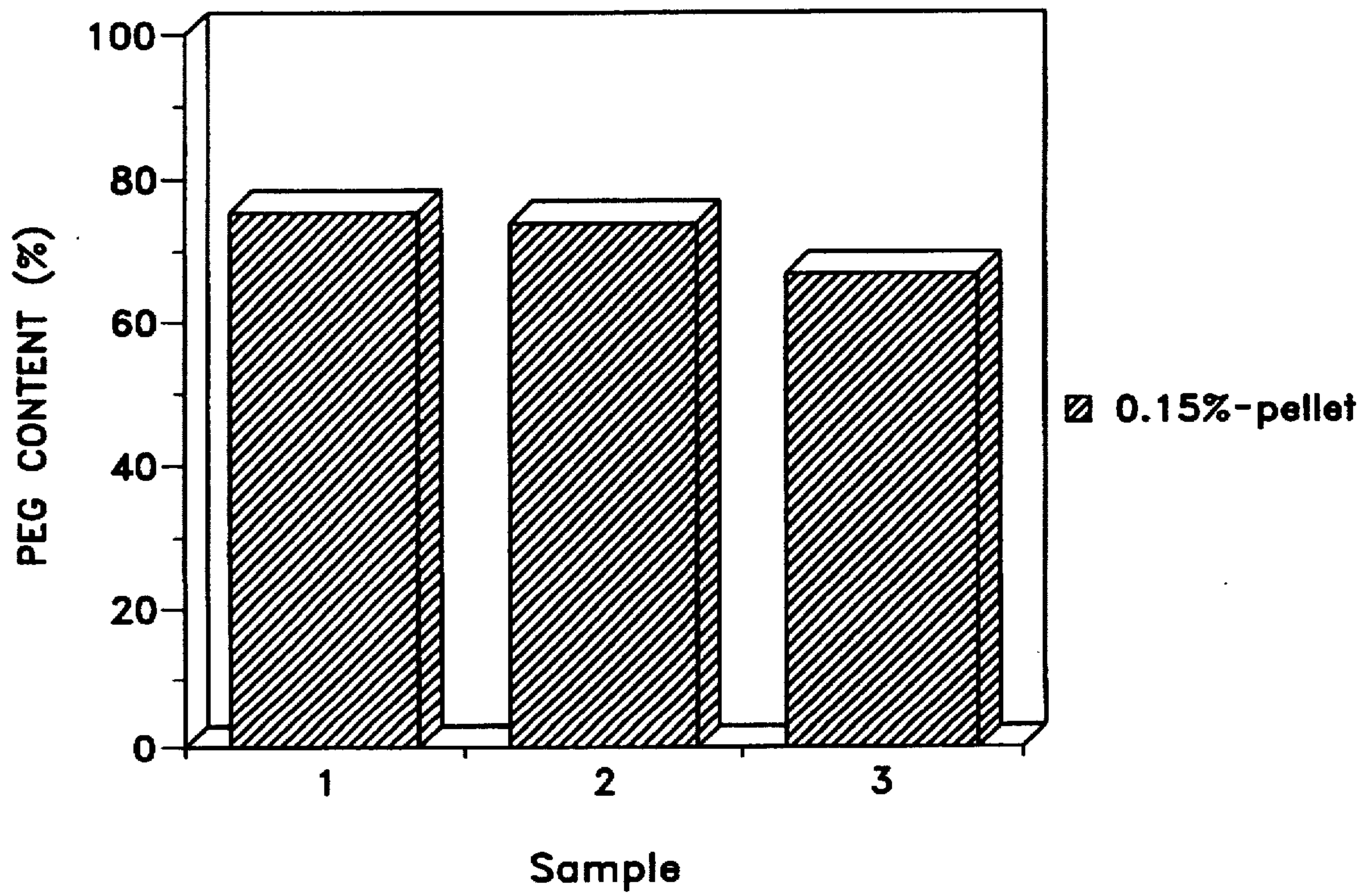
Figure 1: PEG Content in gel prepared from 0.15% w/v SPEG
