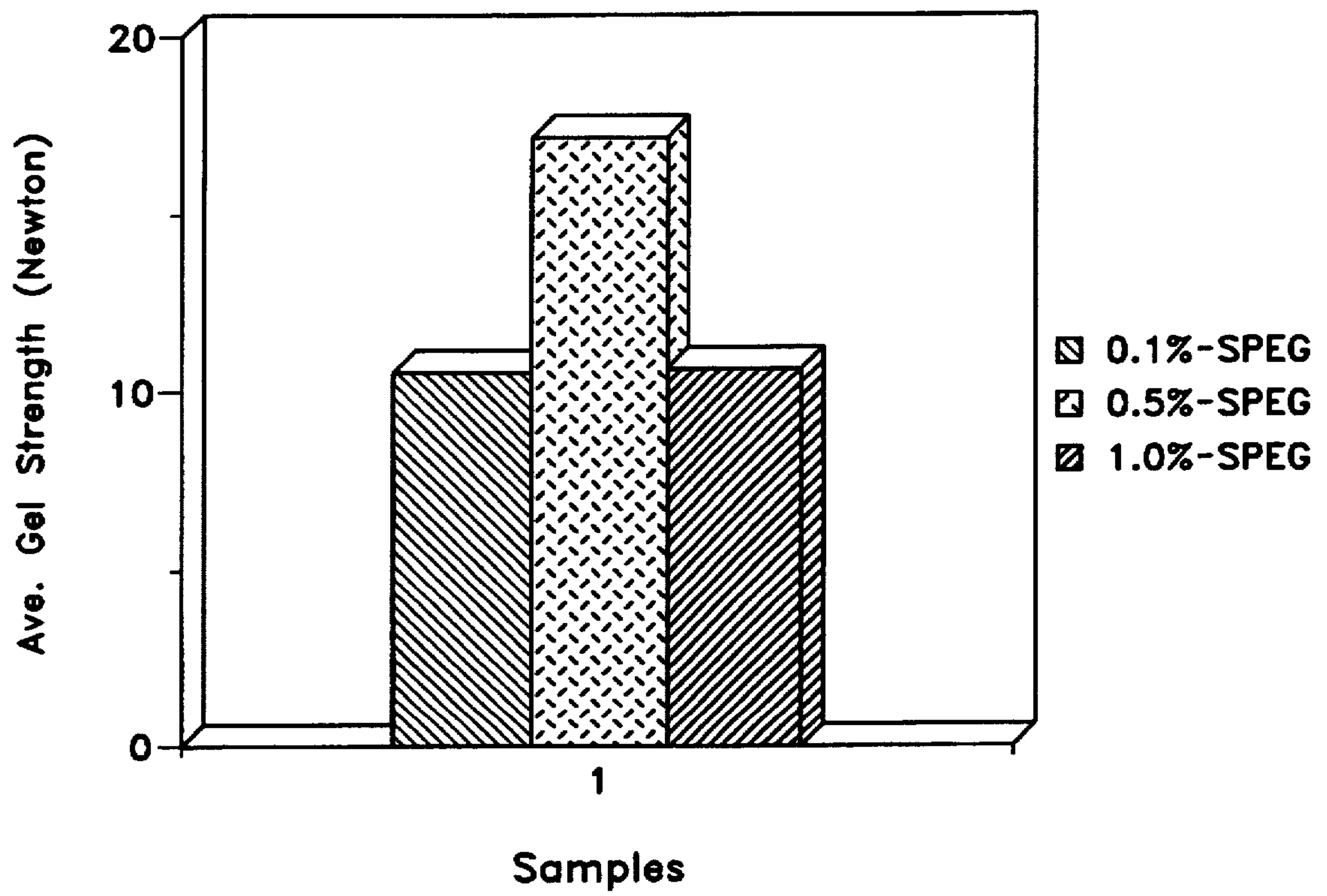
Figure 7: Gel Strength vs. %Conc. of D-SGPEG (n=4)
