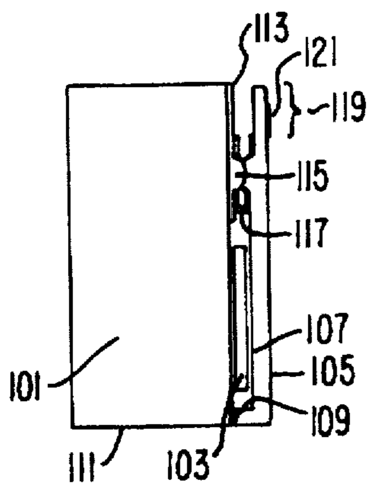
FIG. 1. PRIOR ART
