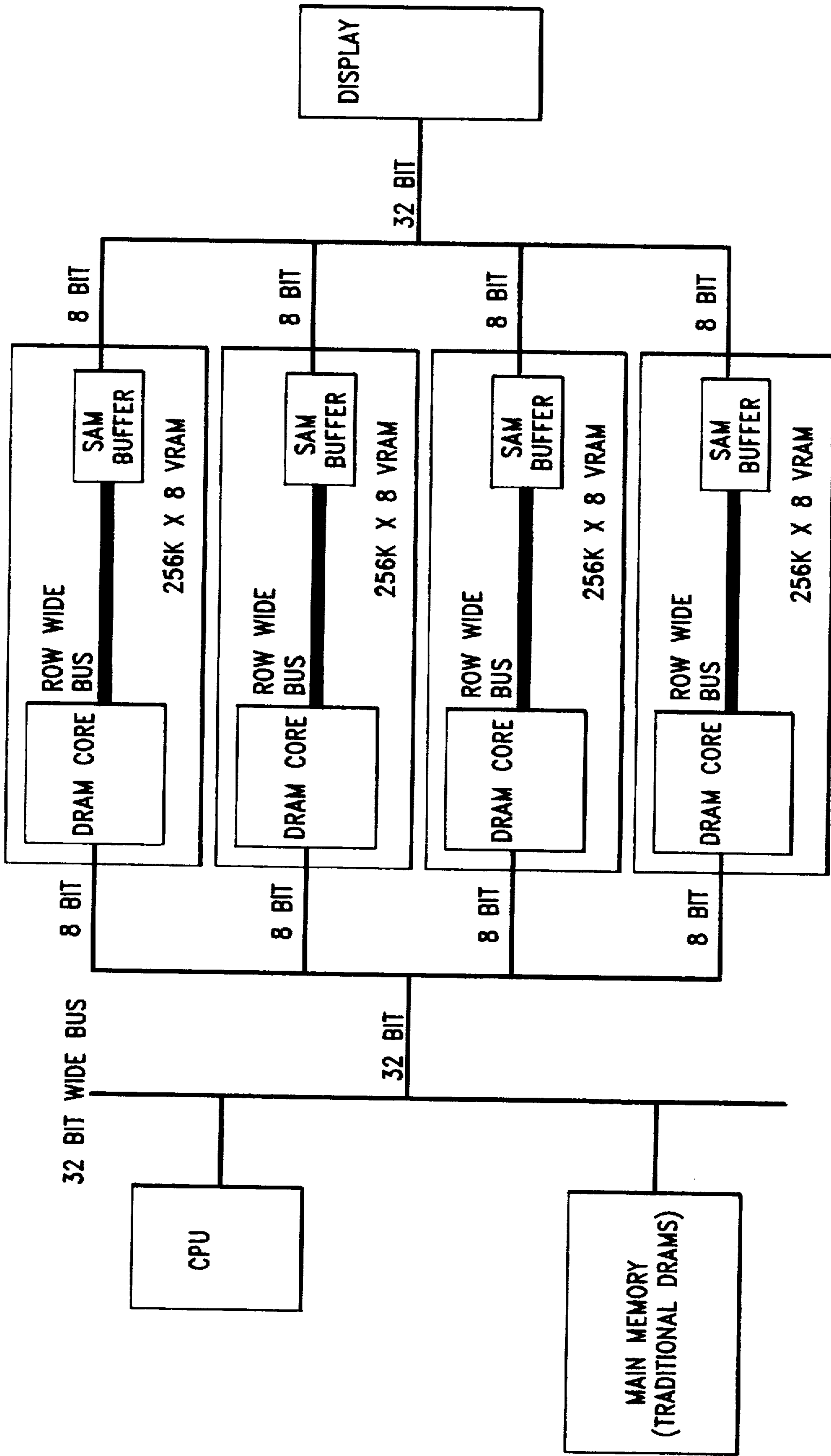
FIG. 6 (PRIOR ART)
