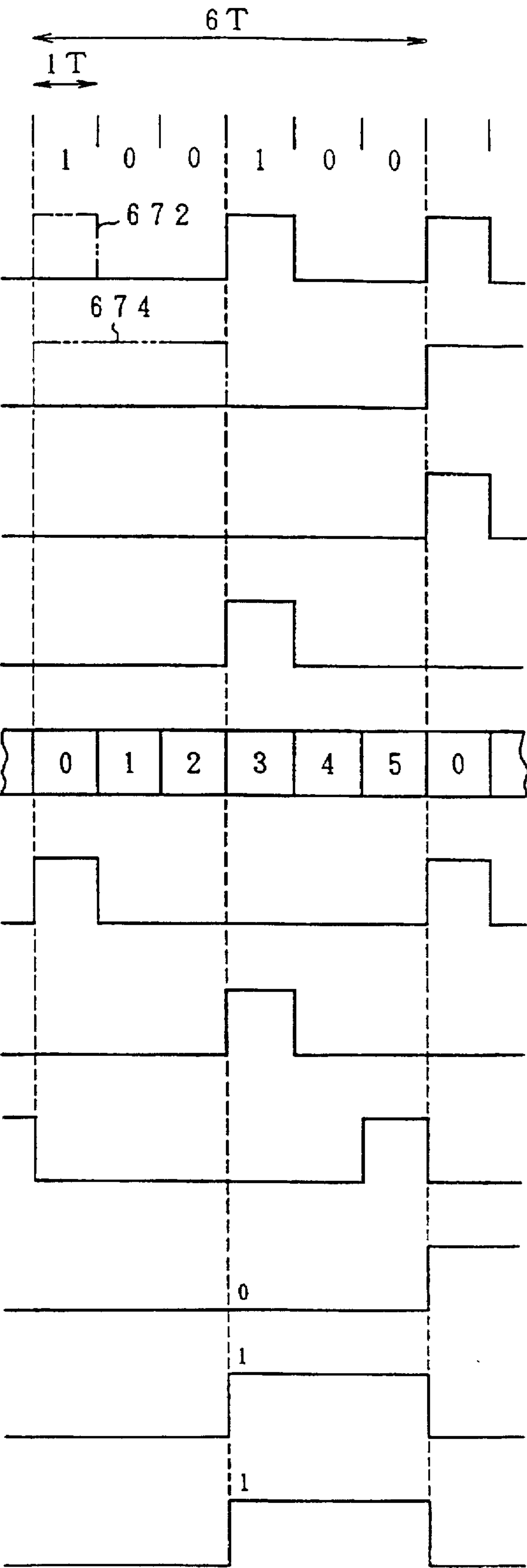
FIG. 65C POLARITY SIGNAL E4
