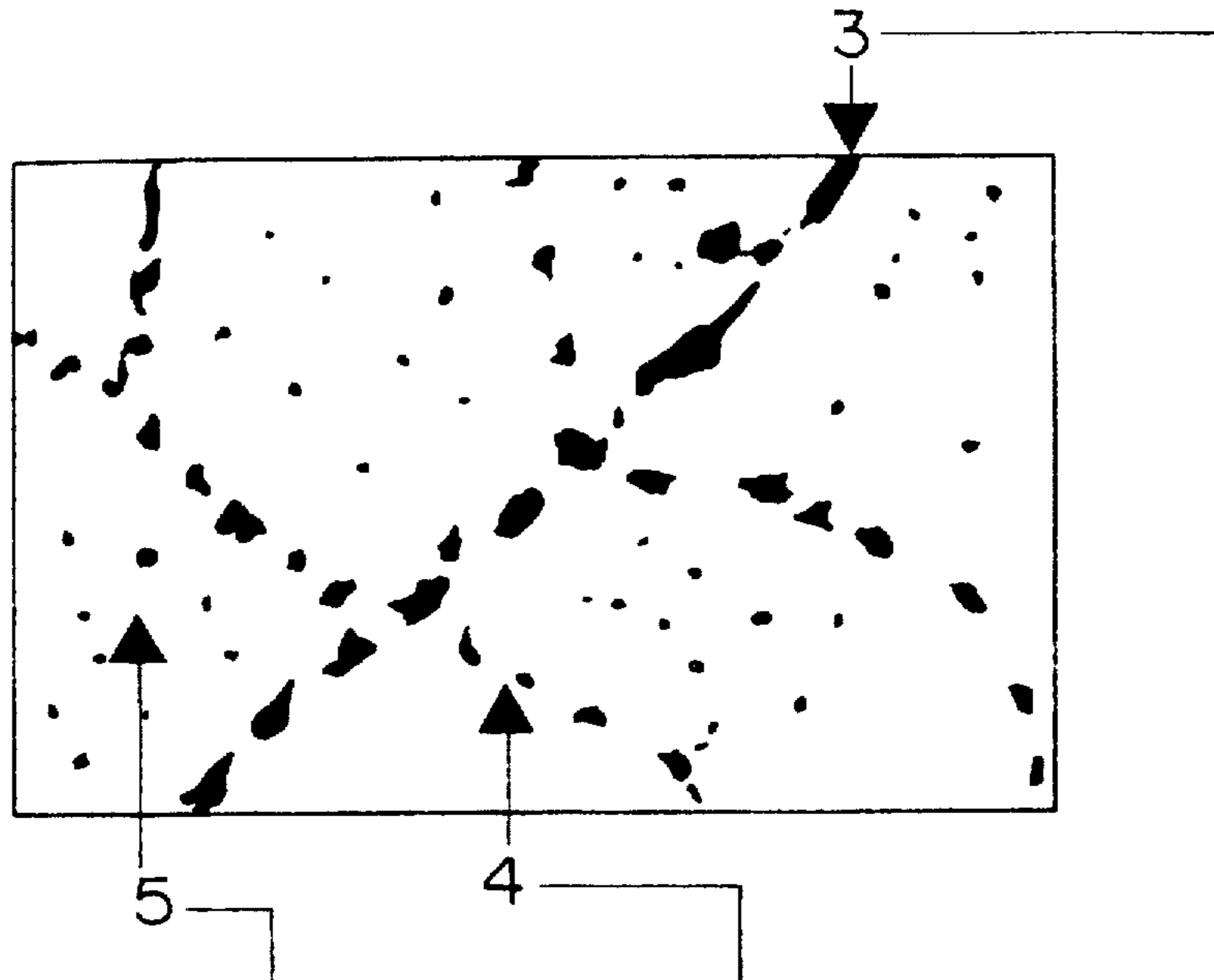
TYPE OF WHOLE METALLOGRAPHIC STRUCTURE: TEMPERED MARTENSITE STRUCTURE
