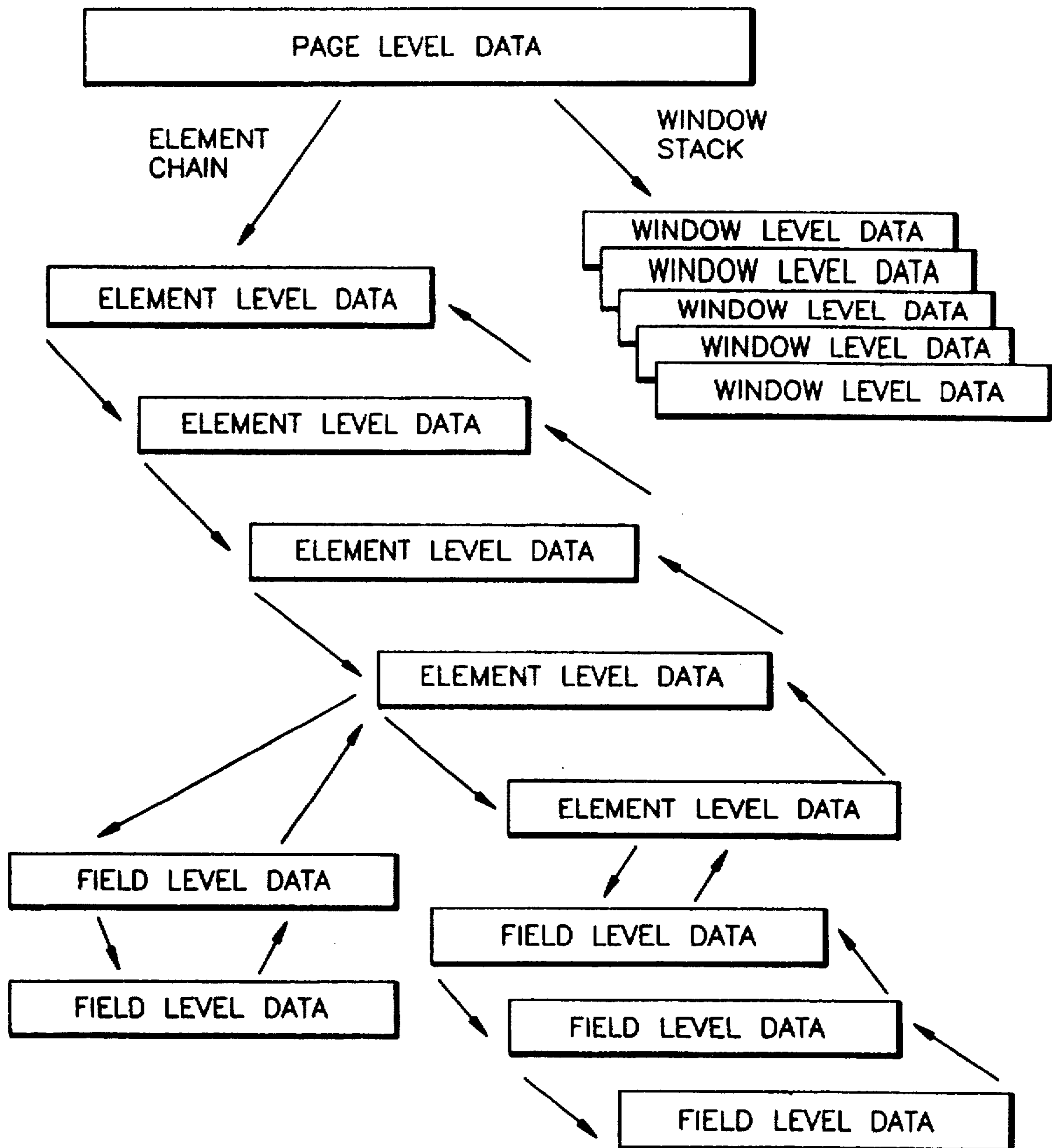
FIG. 10 PAGE PROCESSING TABLE (ppt)
