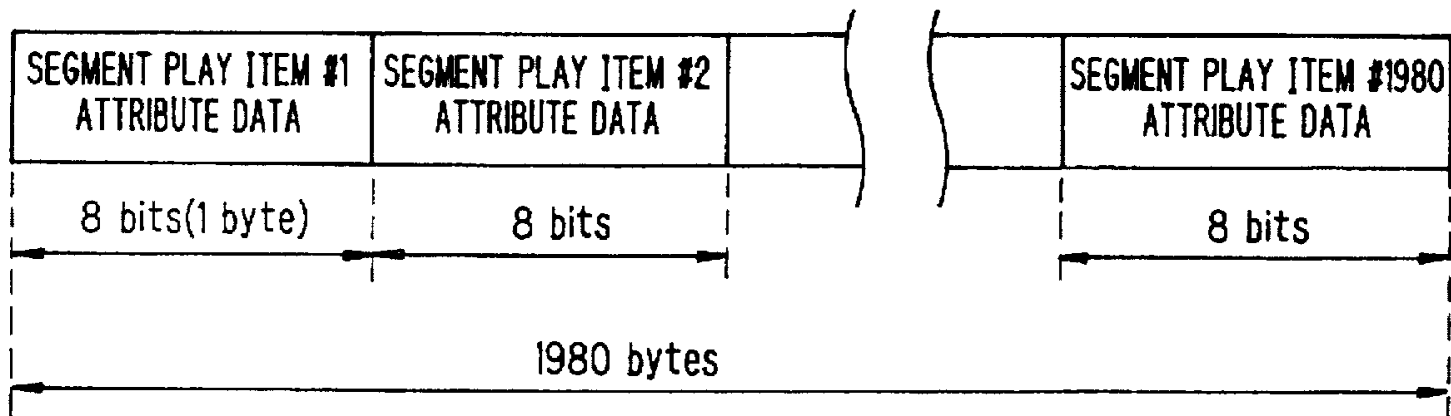
SEGMENT PLAY ITEM CONTENT TABLE
