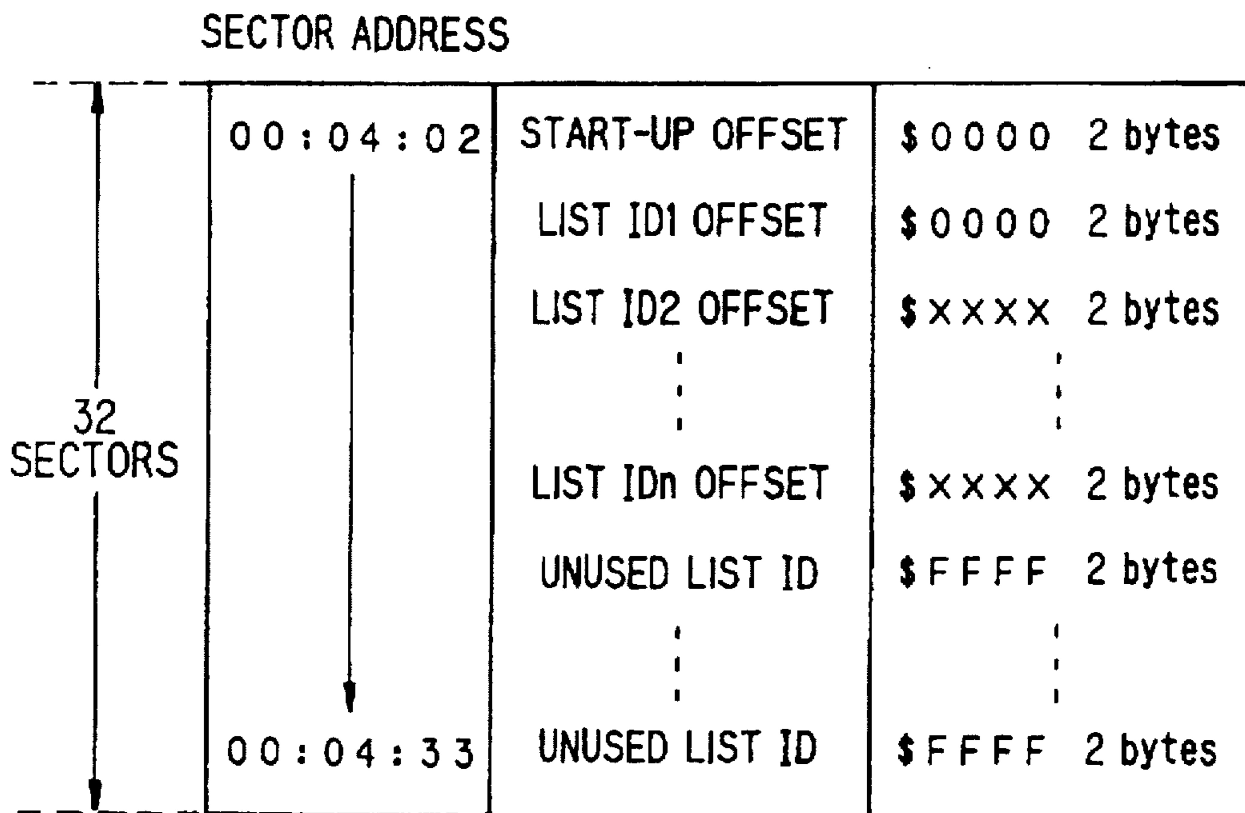
LIST ID OFFSET TABLE ( LIST ID NUMBER = n )
