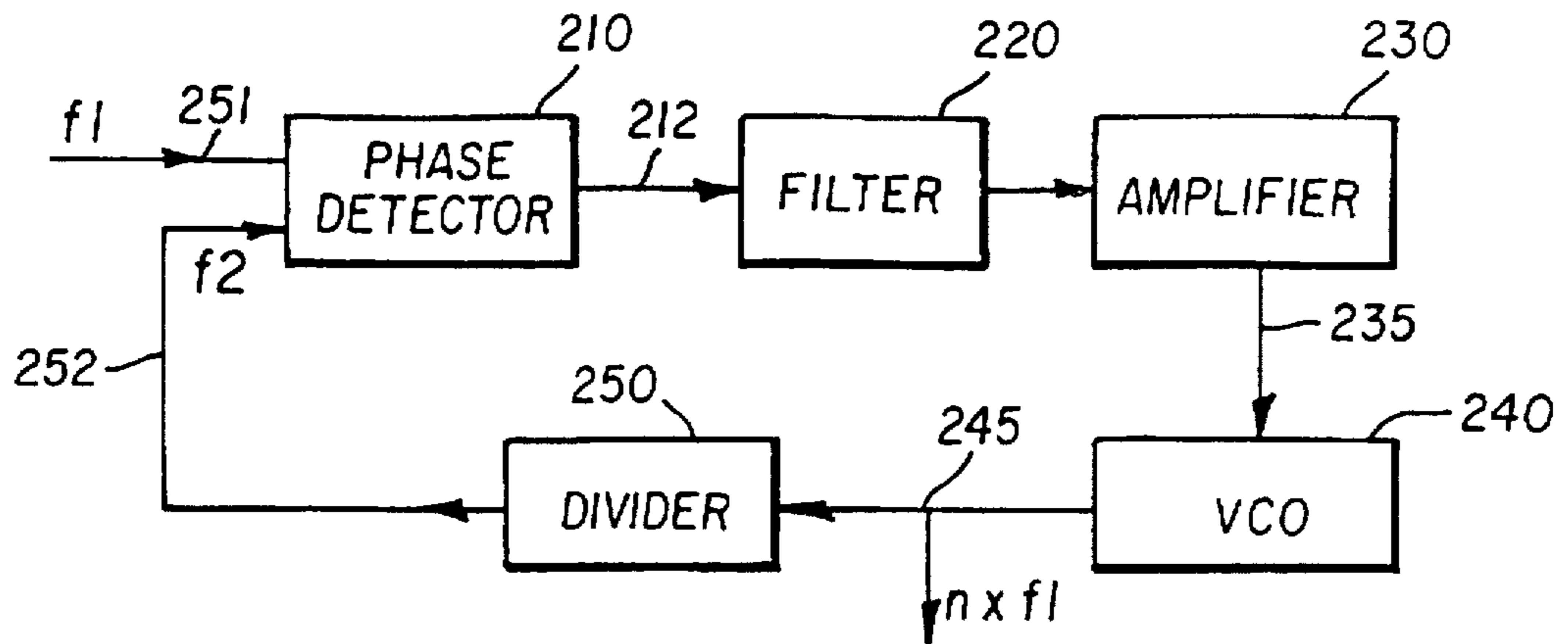
FIG. 2 (prior art)
