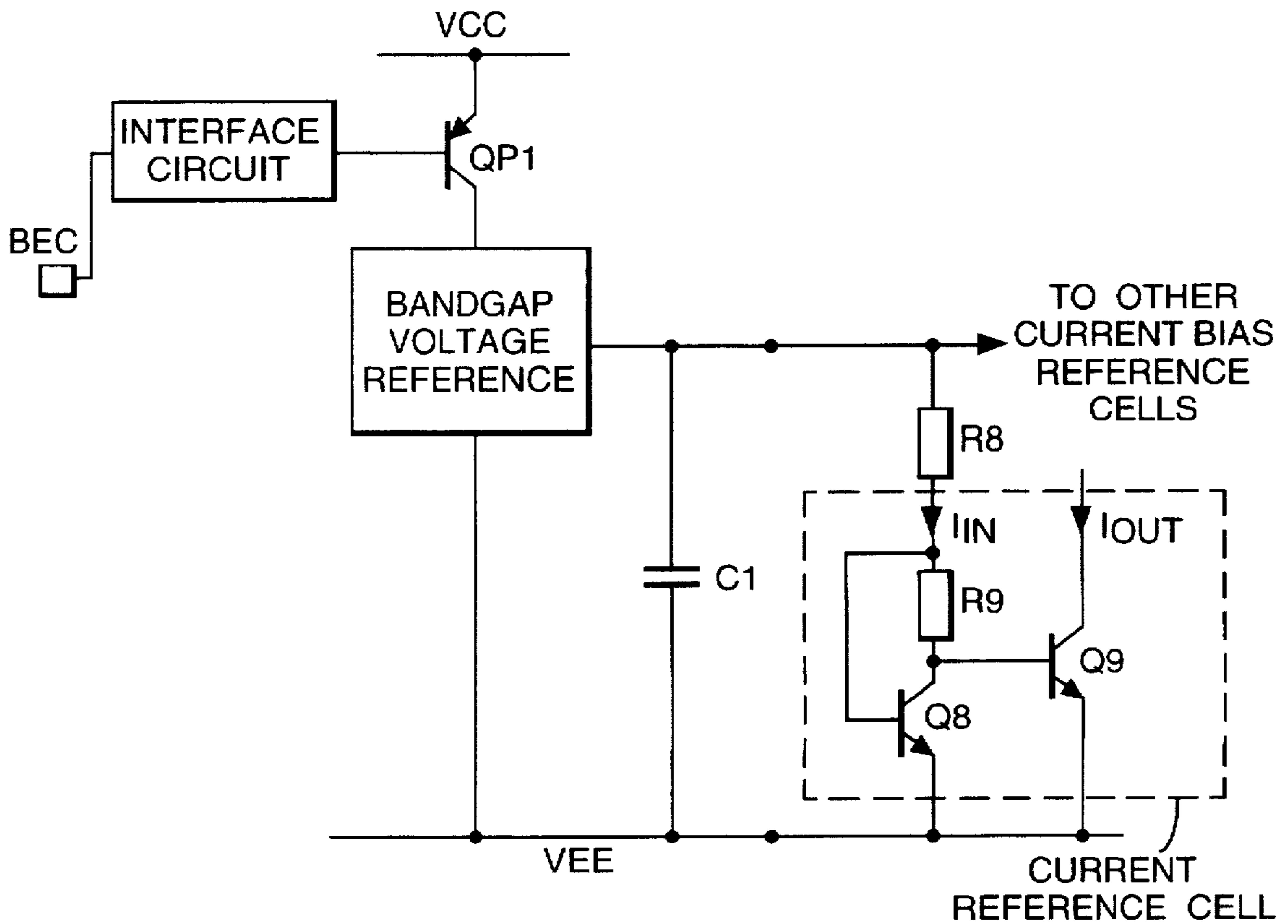
Fig.2. PRIOR ART
