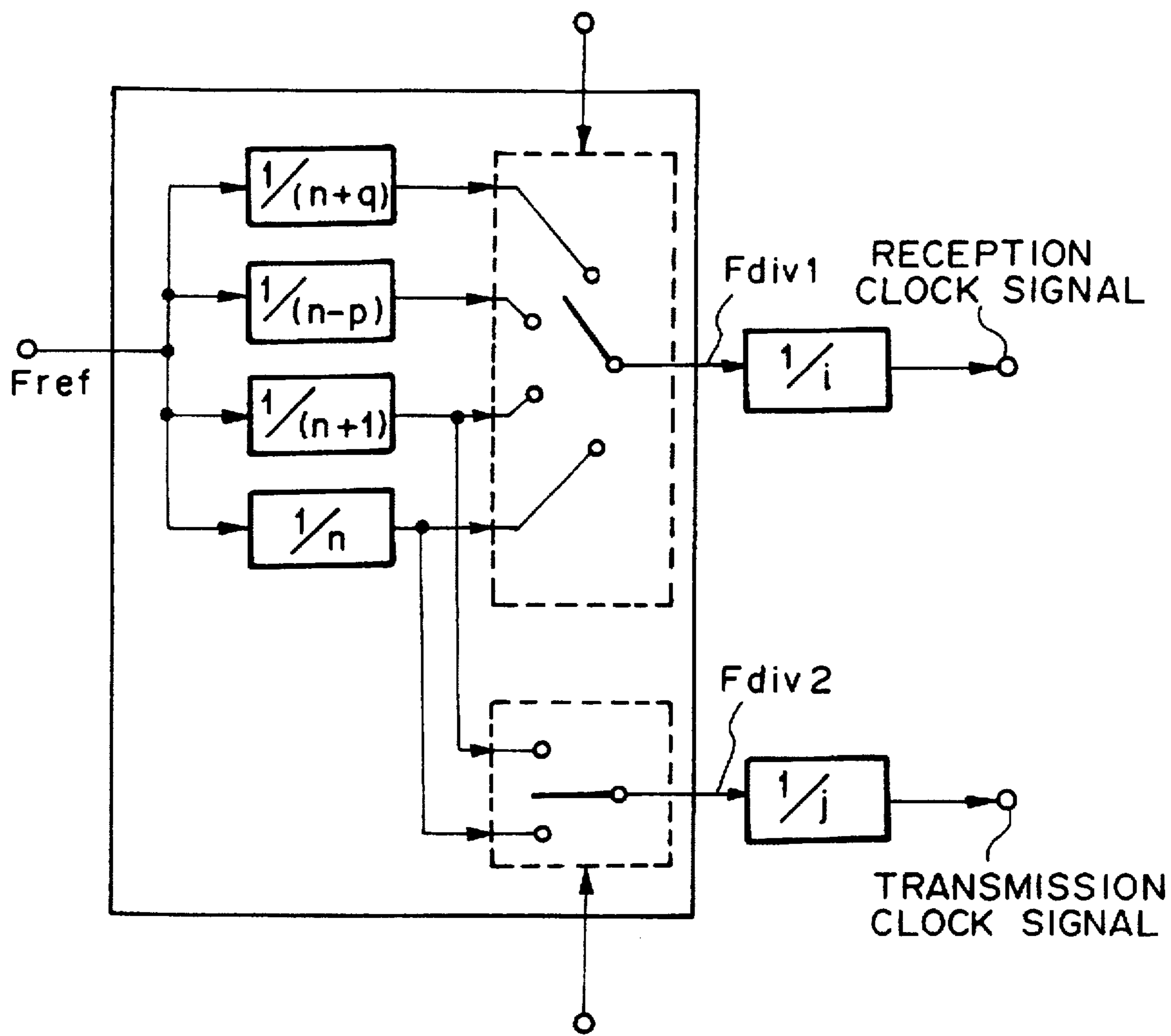
OUTPUT SIGNAL OF FREQUENCY DIVIDING CONTROLLER 9
