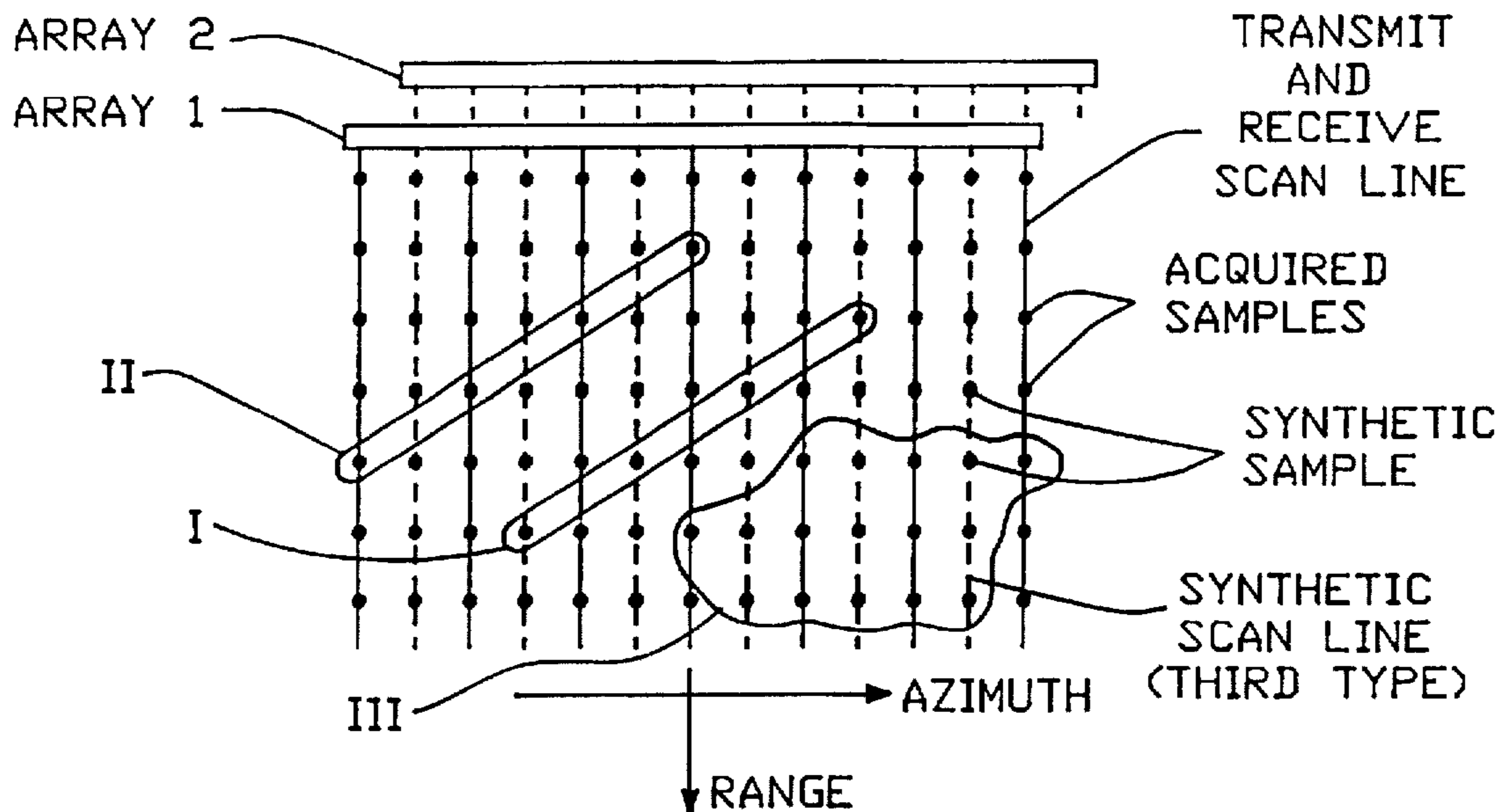
LINEAR SCAN FORMAT (CARTESIAN COORDINATE SAMPLING)
