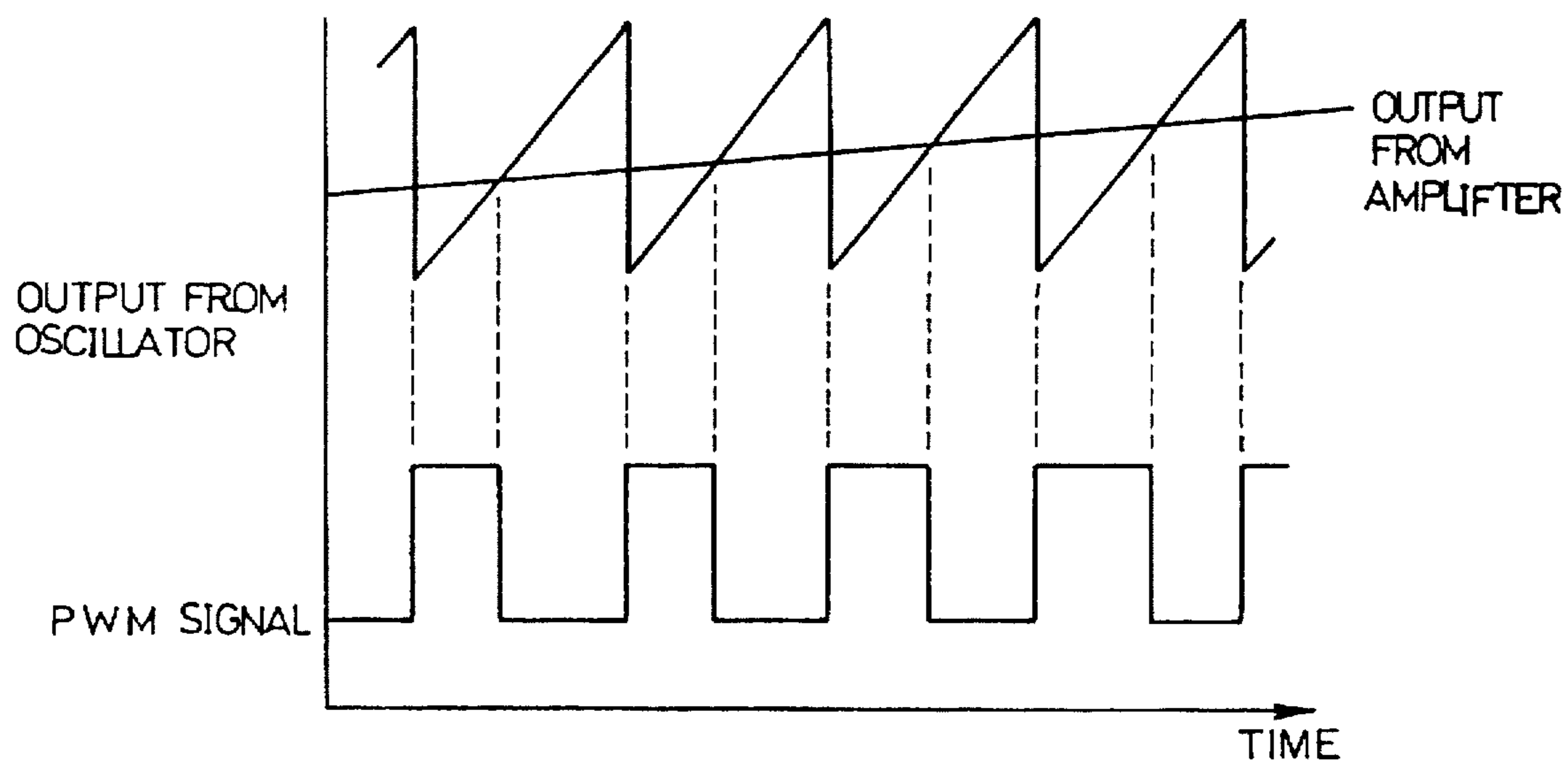
FIG.52 PRIOR ART
