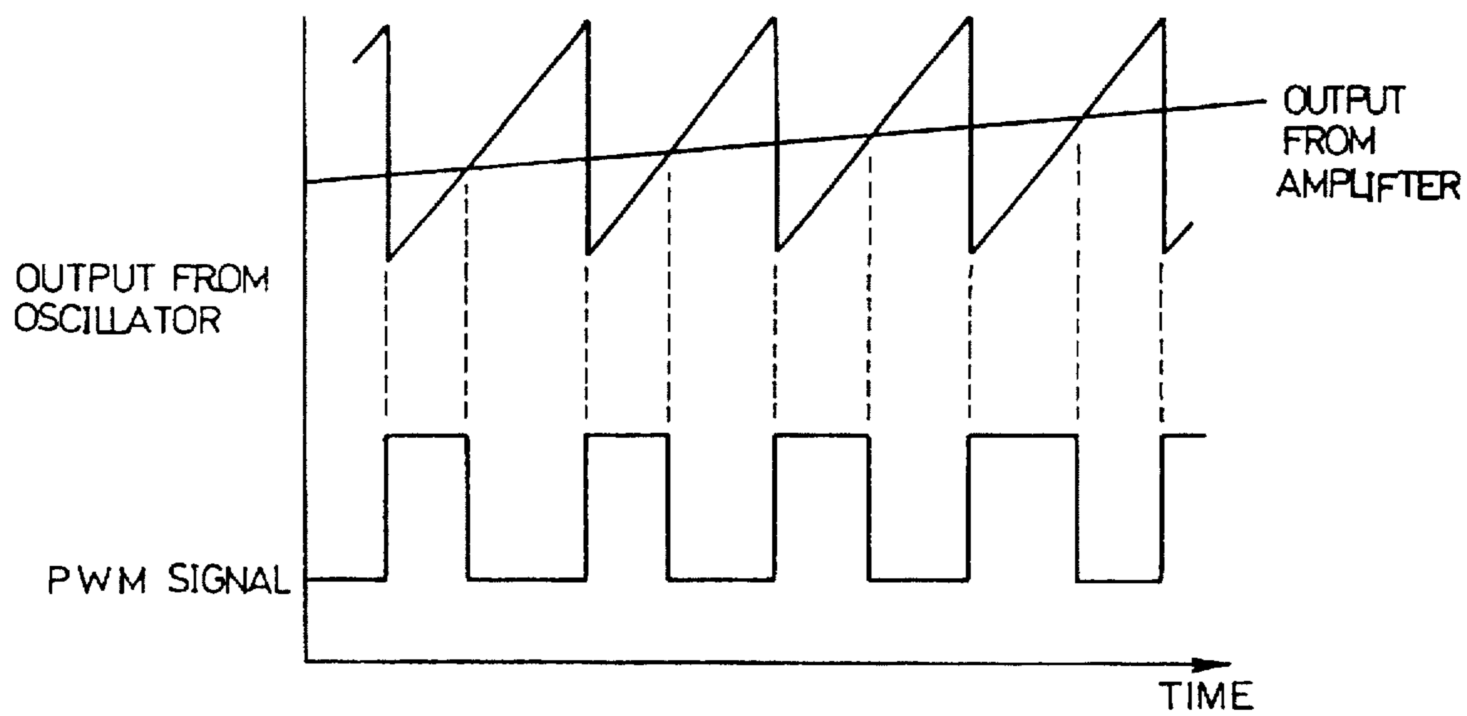
FIG.52 PRIOR ART
