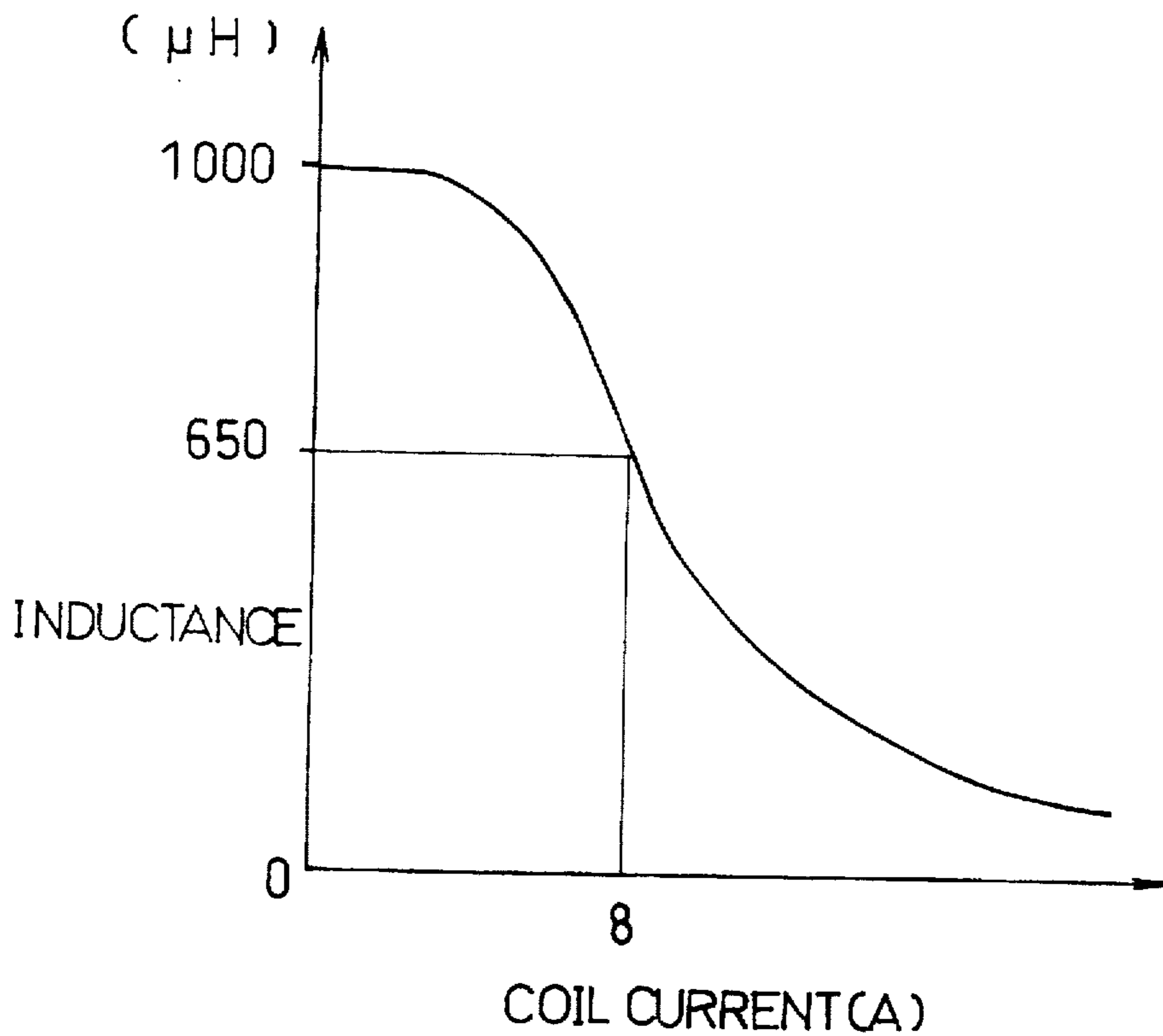
FIG.59 PRIOR ART
