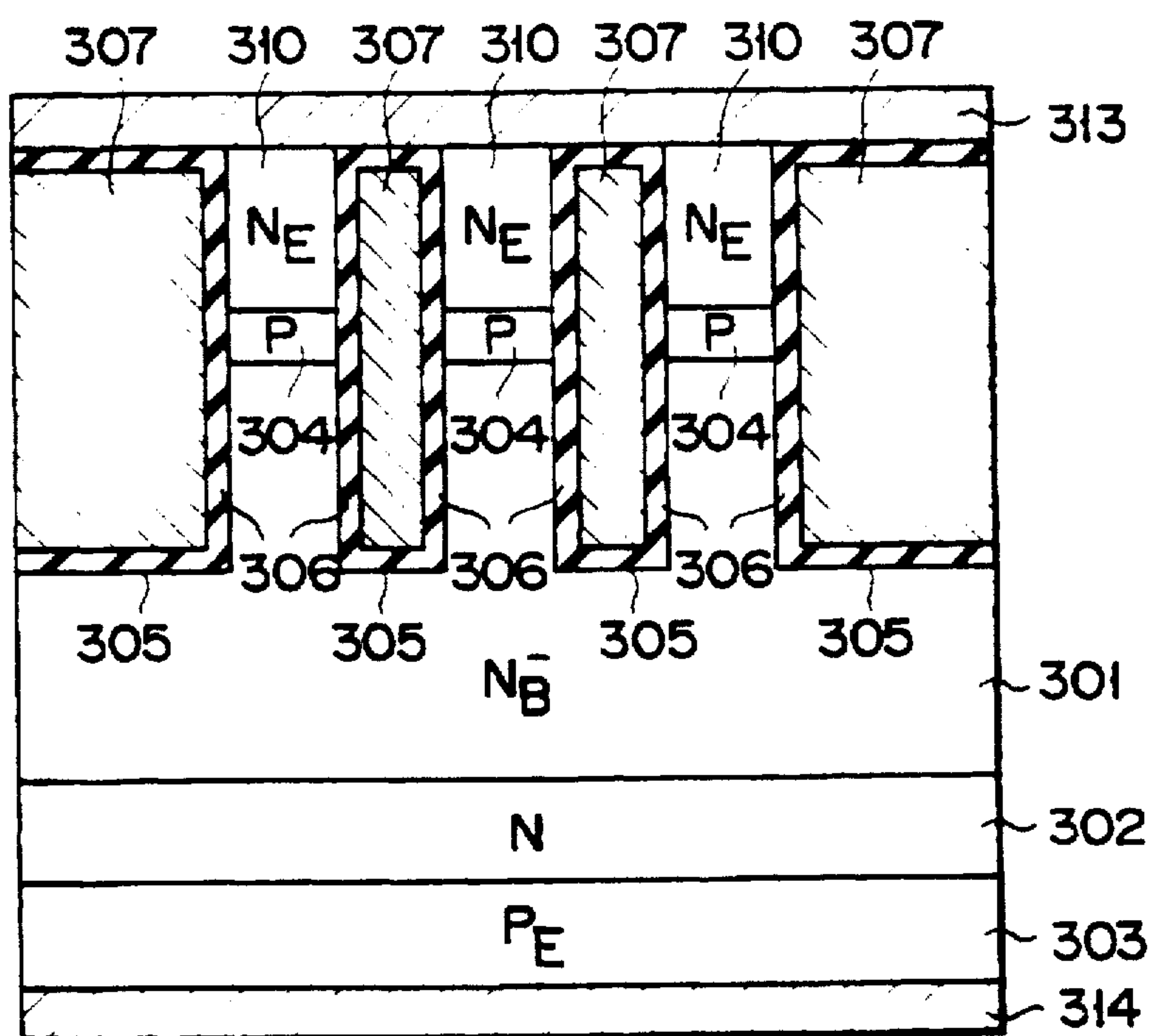
A-A' CROSS SECTION
