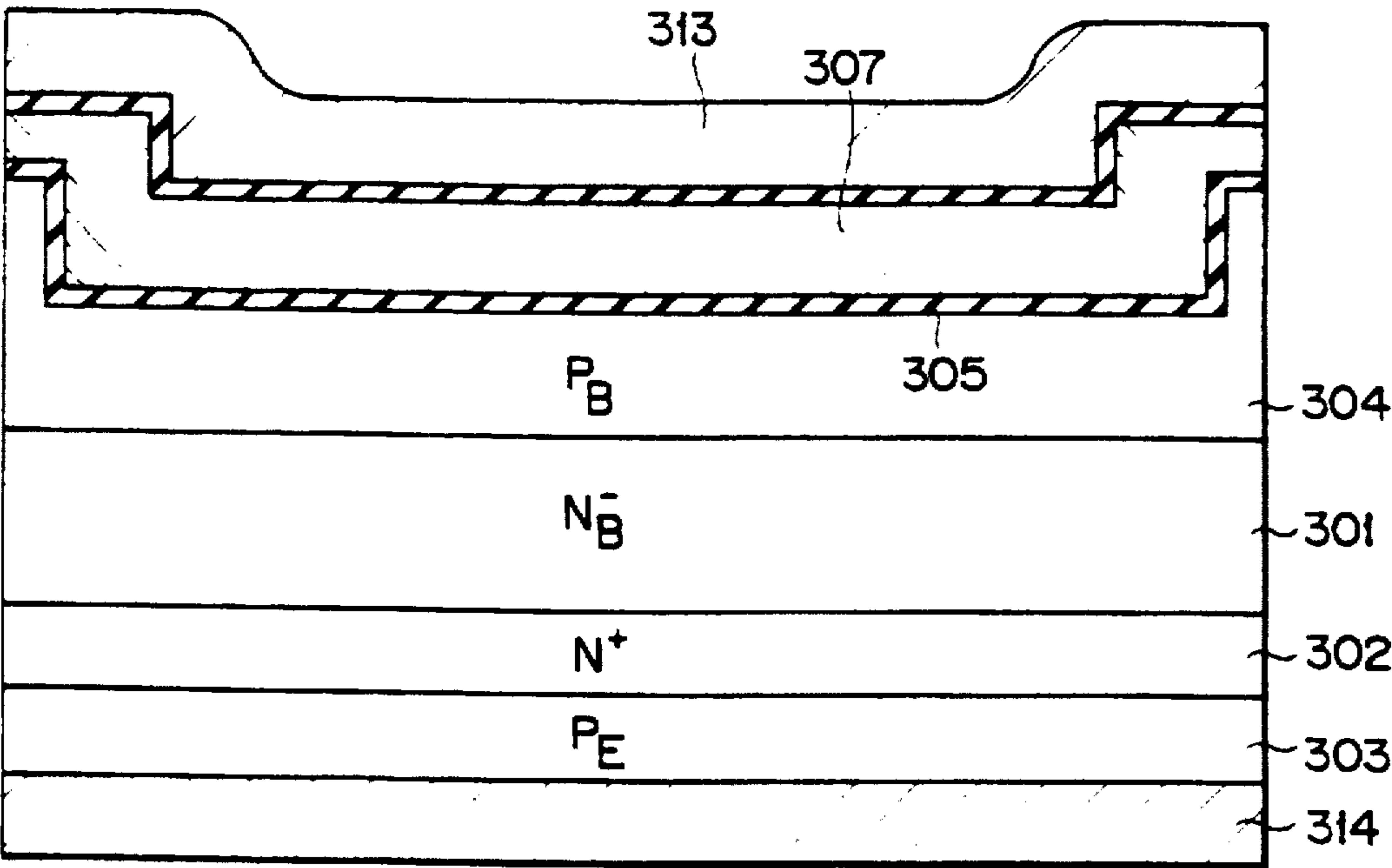
D-D' CROSS SECTION
