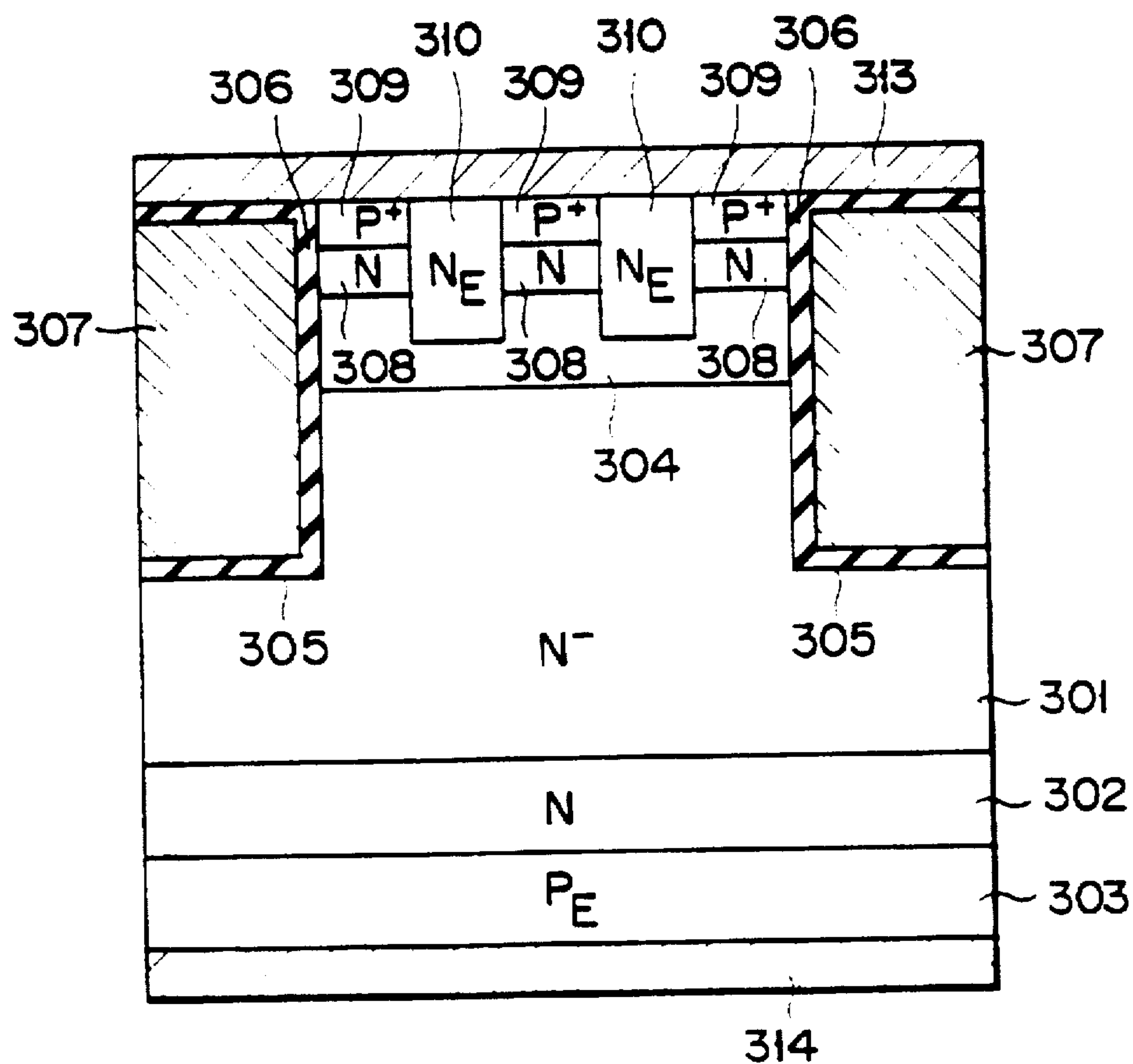
B-B' CROSS SECTION
