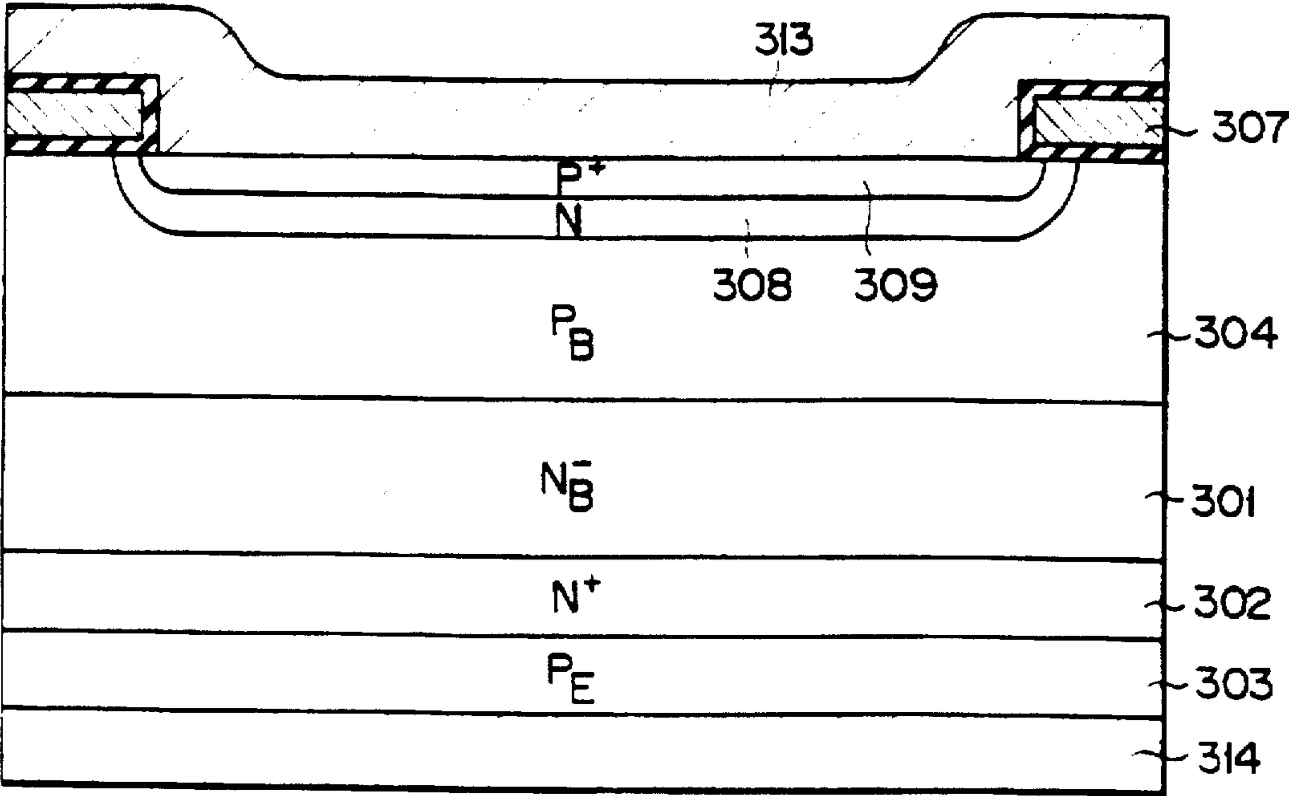
C-C' CROSS SECTION
