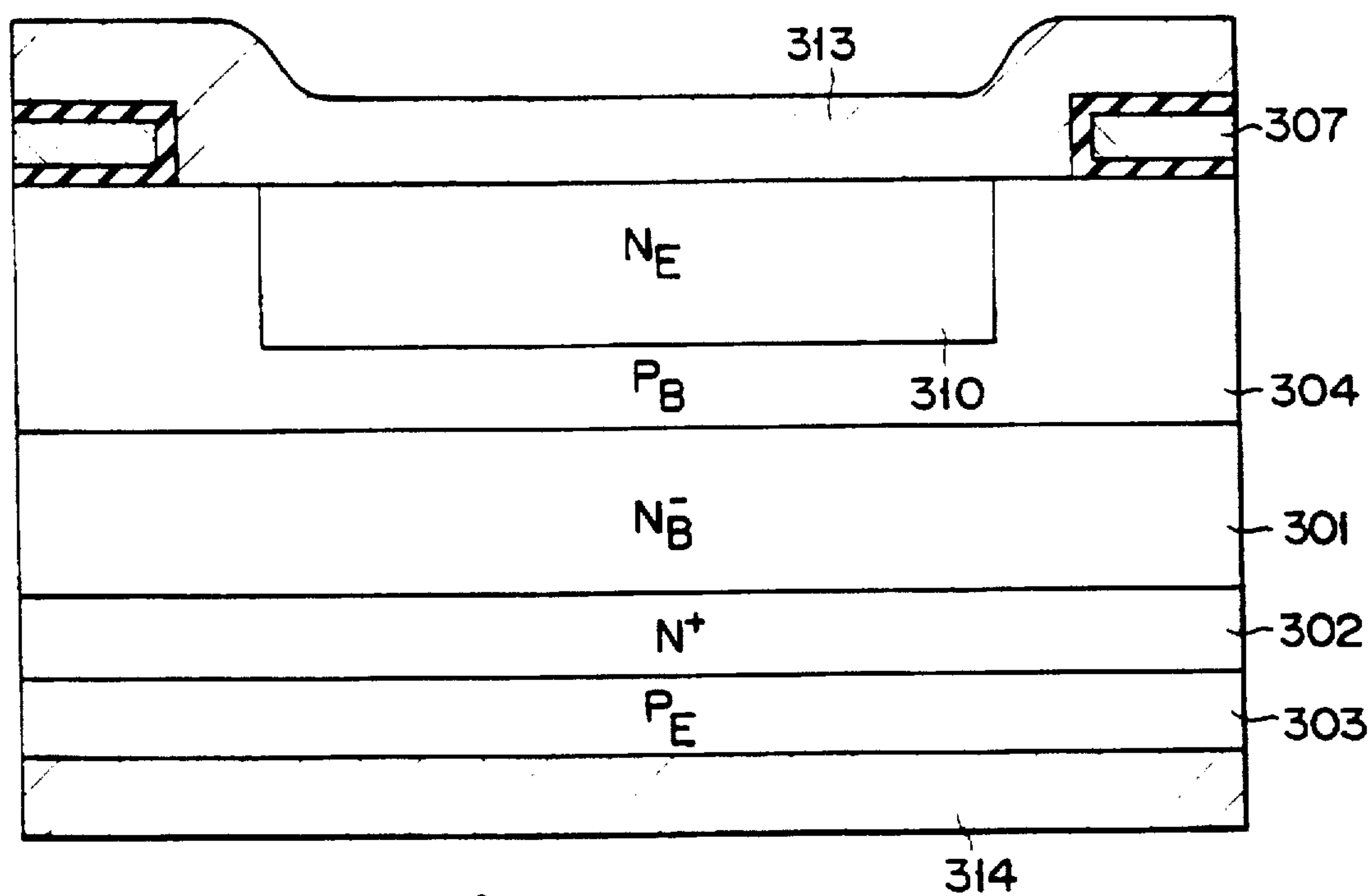
B-B' CROSS SECTION
