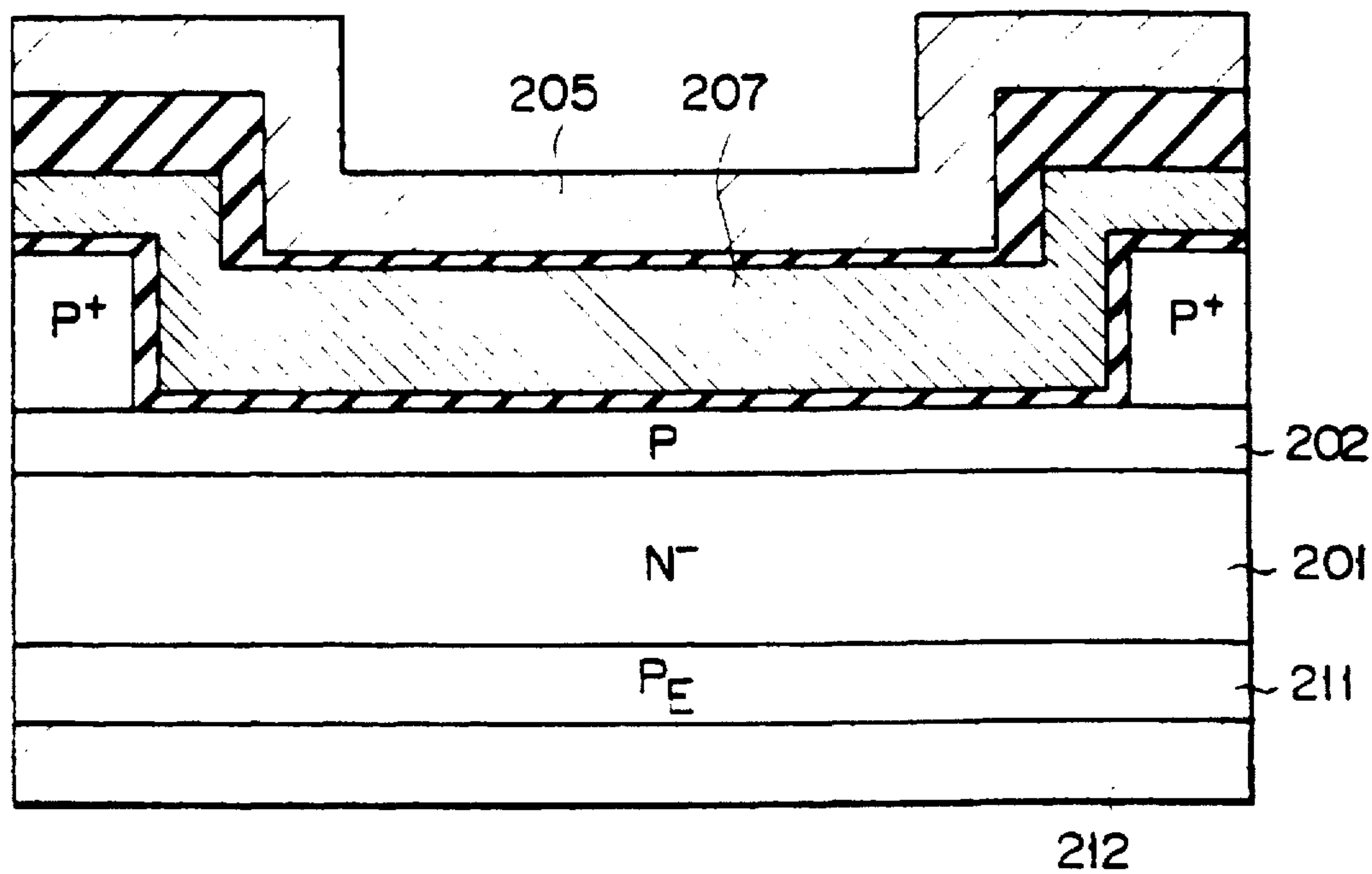
C-C' CROSS SECTION
