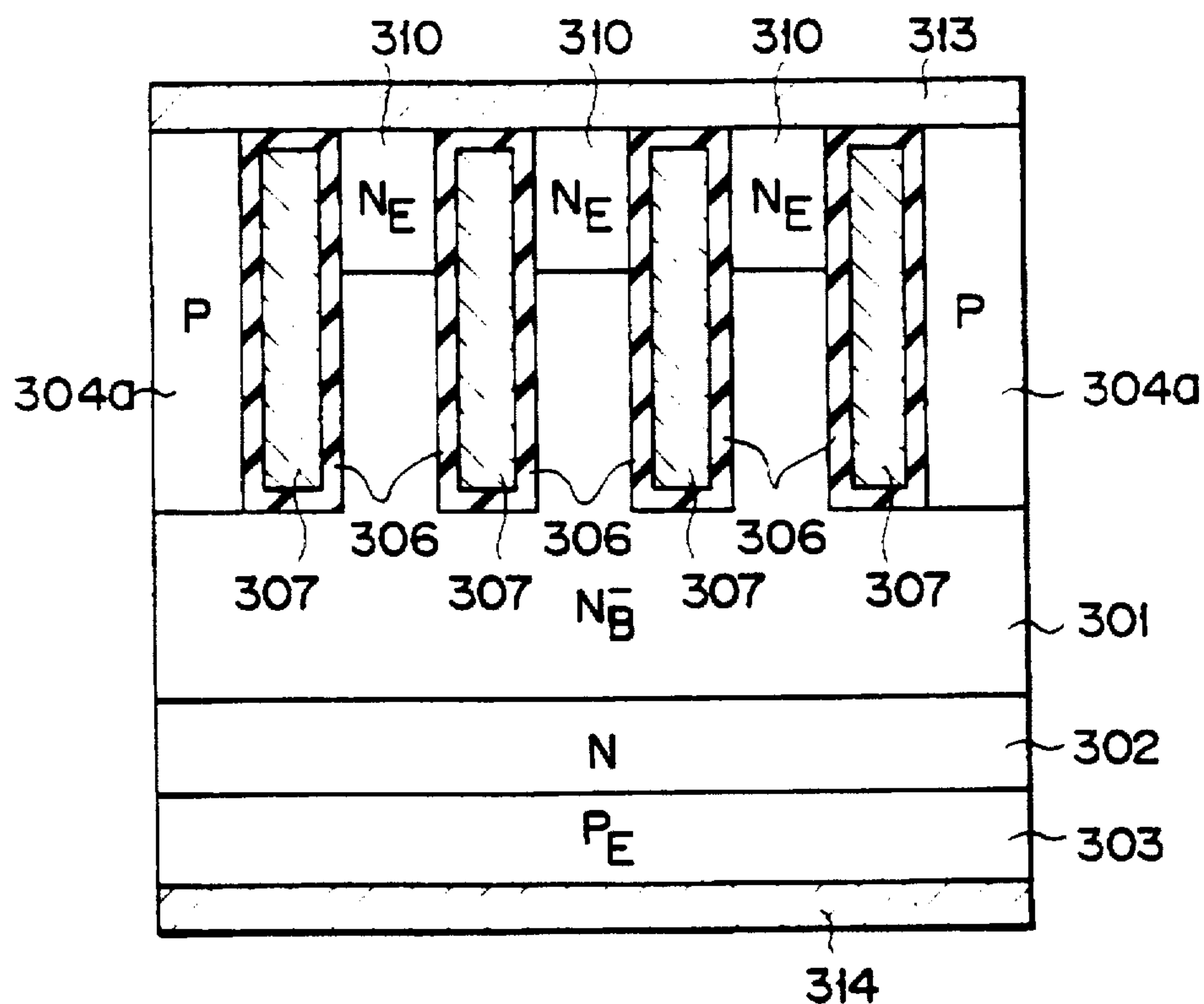
A-A' CROSS SECTION
