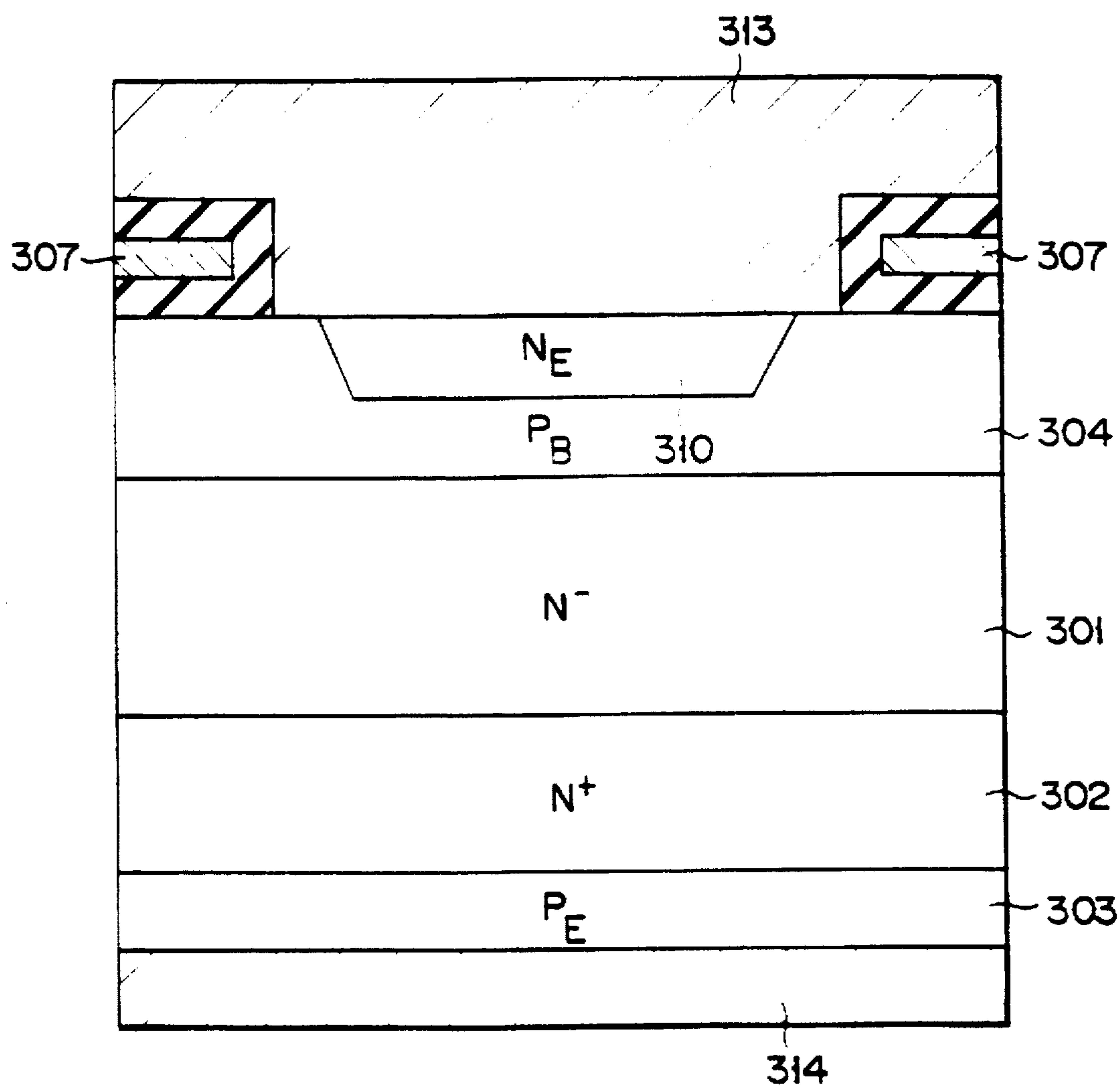
B-B' CROSS SECTION
