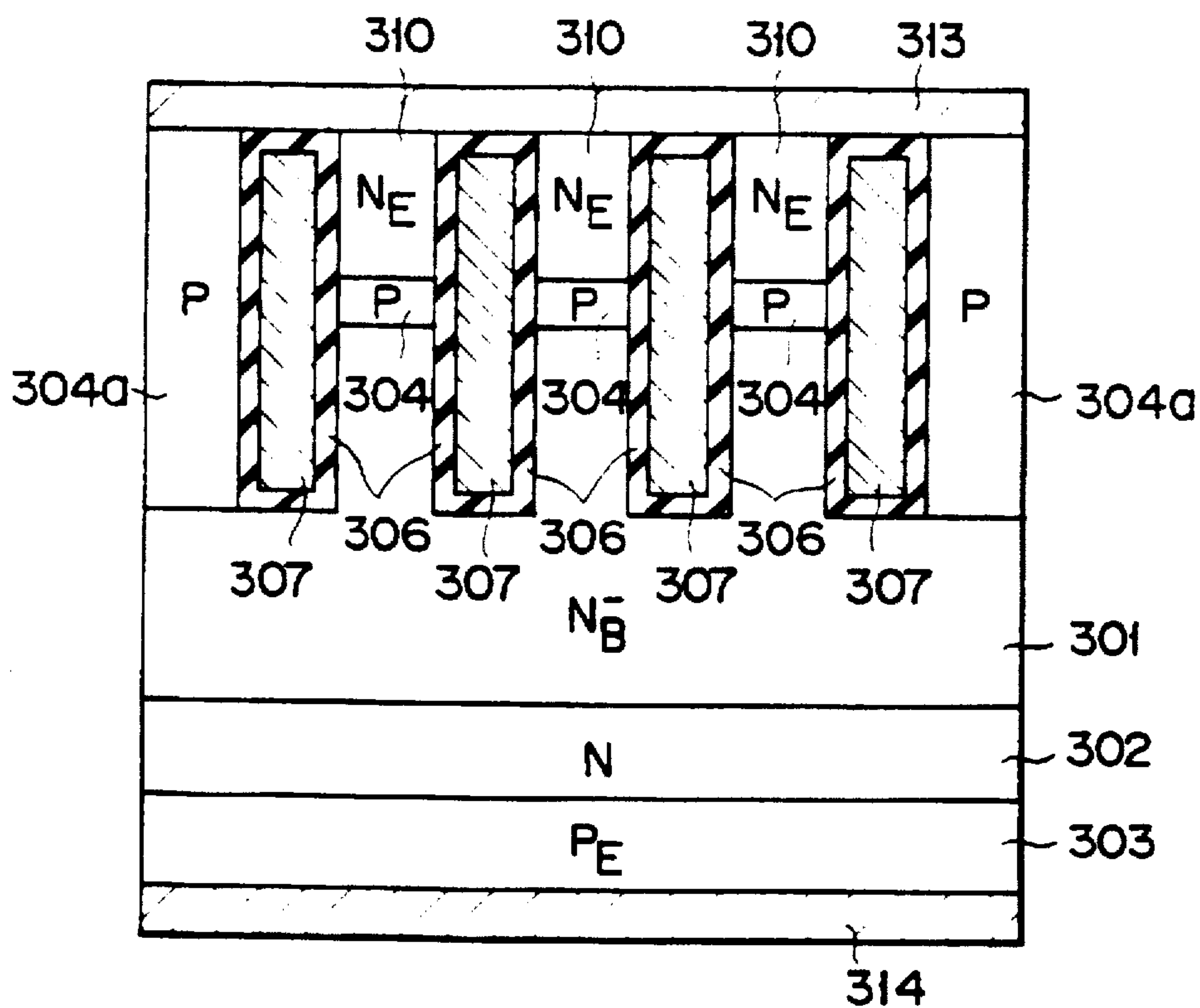
A-A' CROSS SECTION
