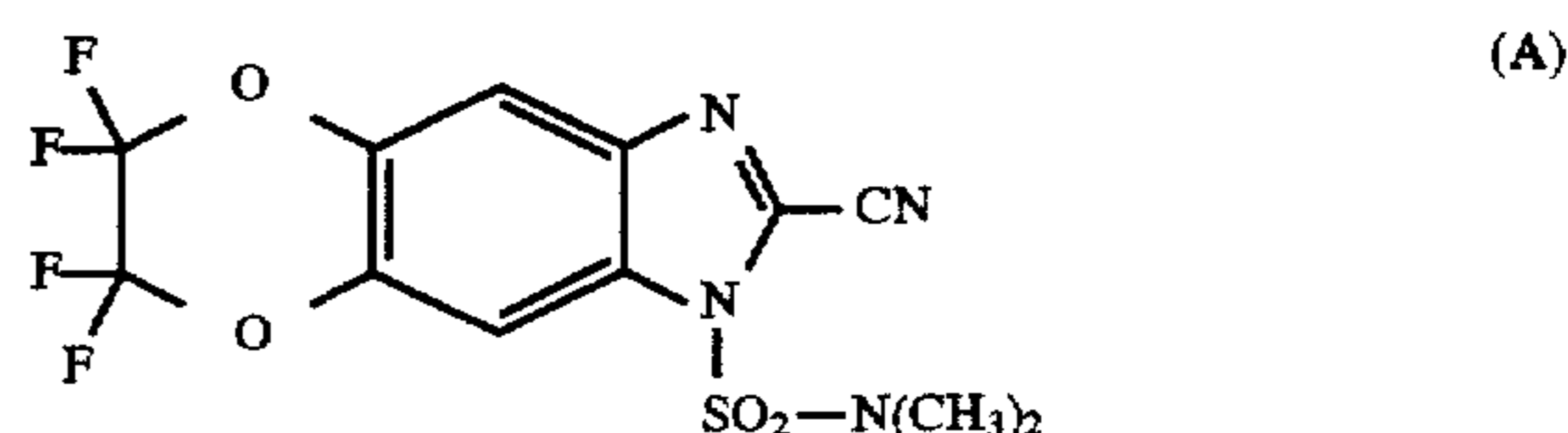
2-cyano-3-dimethylaminosulphonyl-6,6,7,7-tetrafluoro-[1,4]dioxino[2,3-f]benzimidazole
