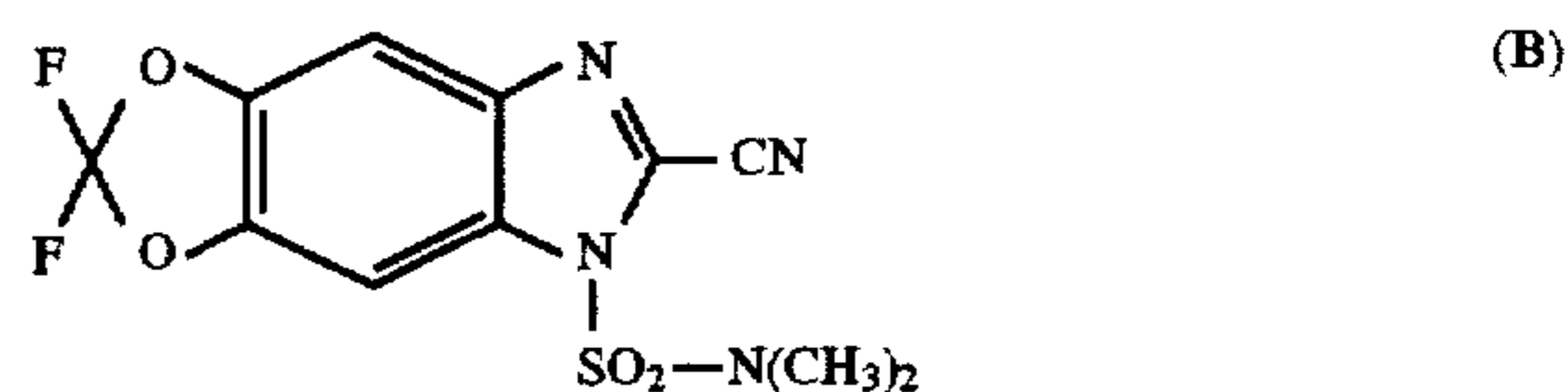
2-cyano-6,6-difluoro-3-dimethylaminosulphonyl-[1,3]dioxolo[4,5-f]benzimidazole
