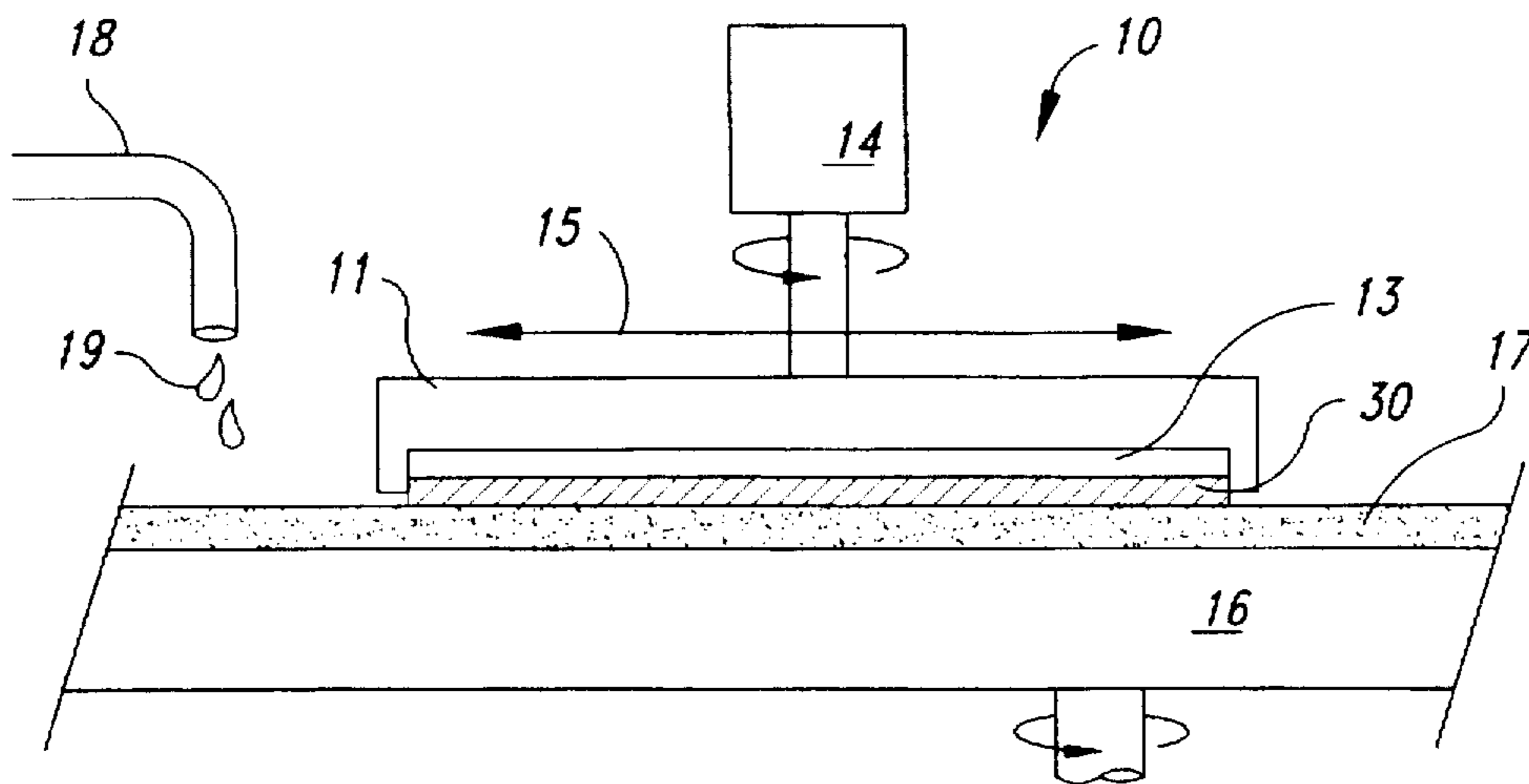
Fig. 1 (PRIOR ART)
