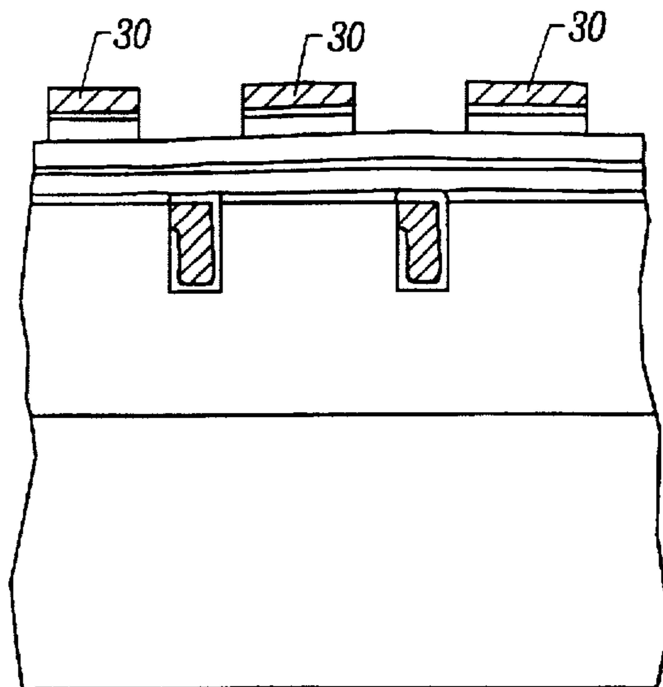
BIT-LINE STRUCTURE
