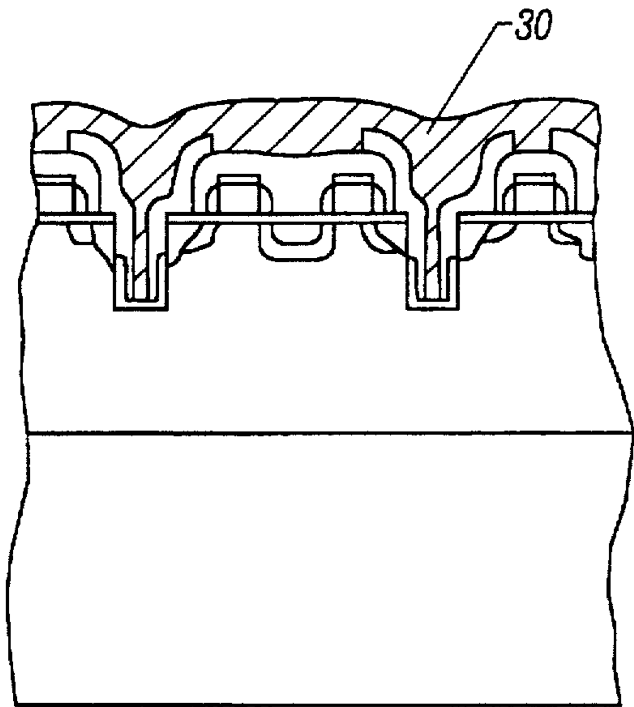
CAPACITOR STRUCTURE
