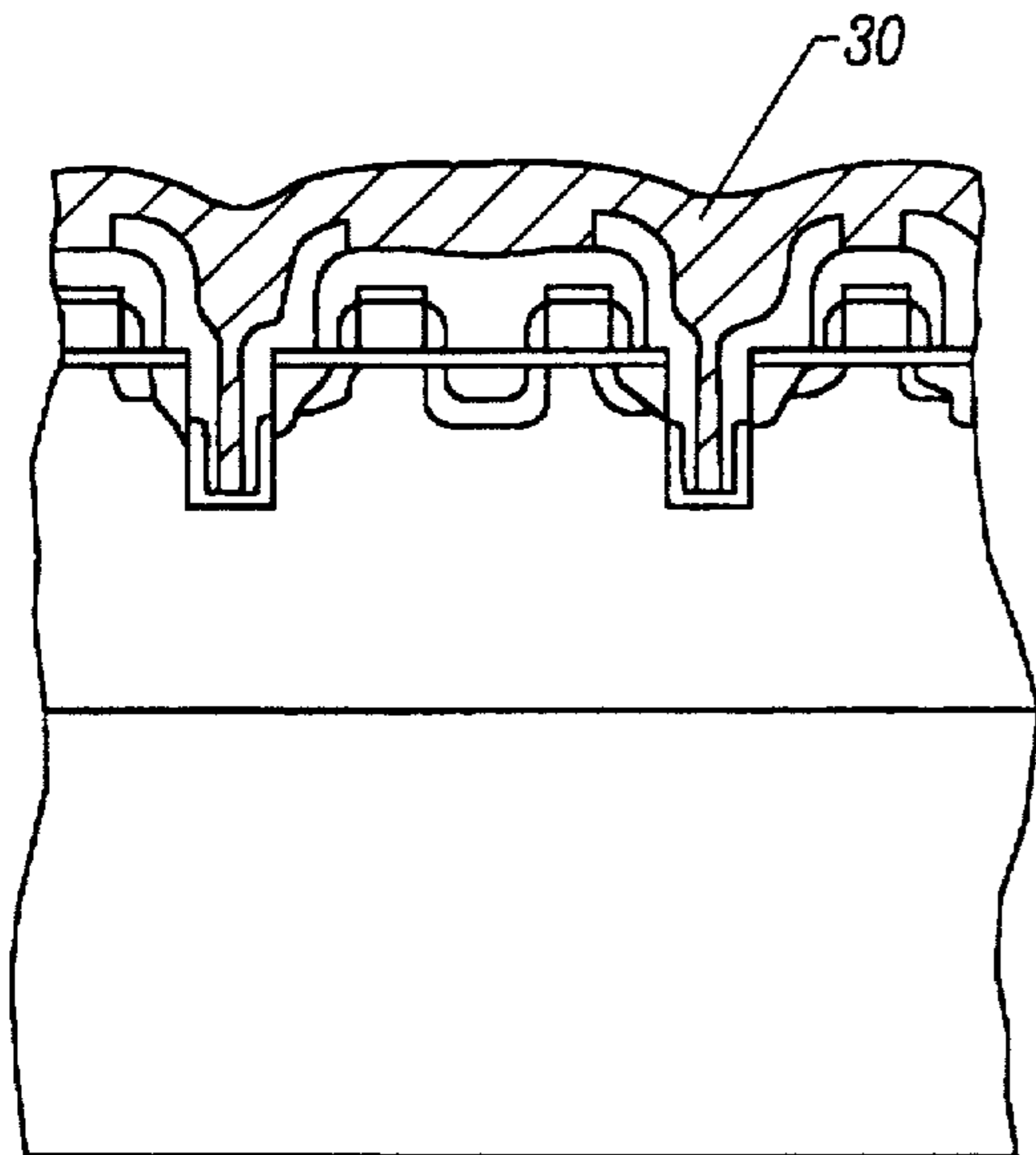
CAPACITOR STRUCTURE
