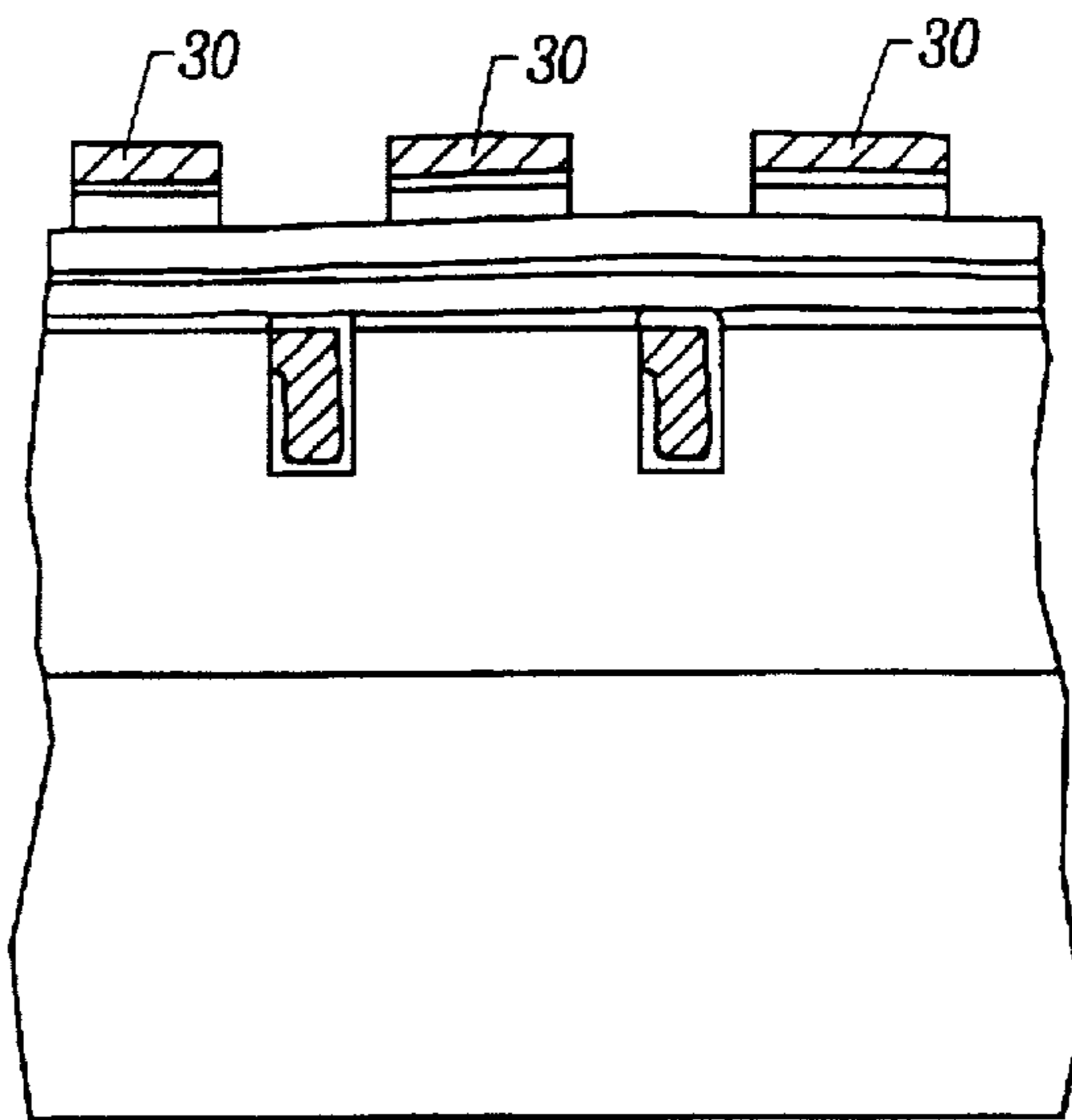
BIT-LINE STRUCTURE
