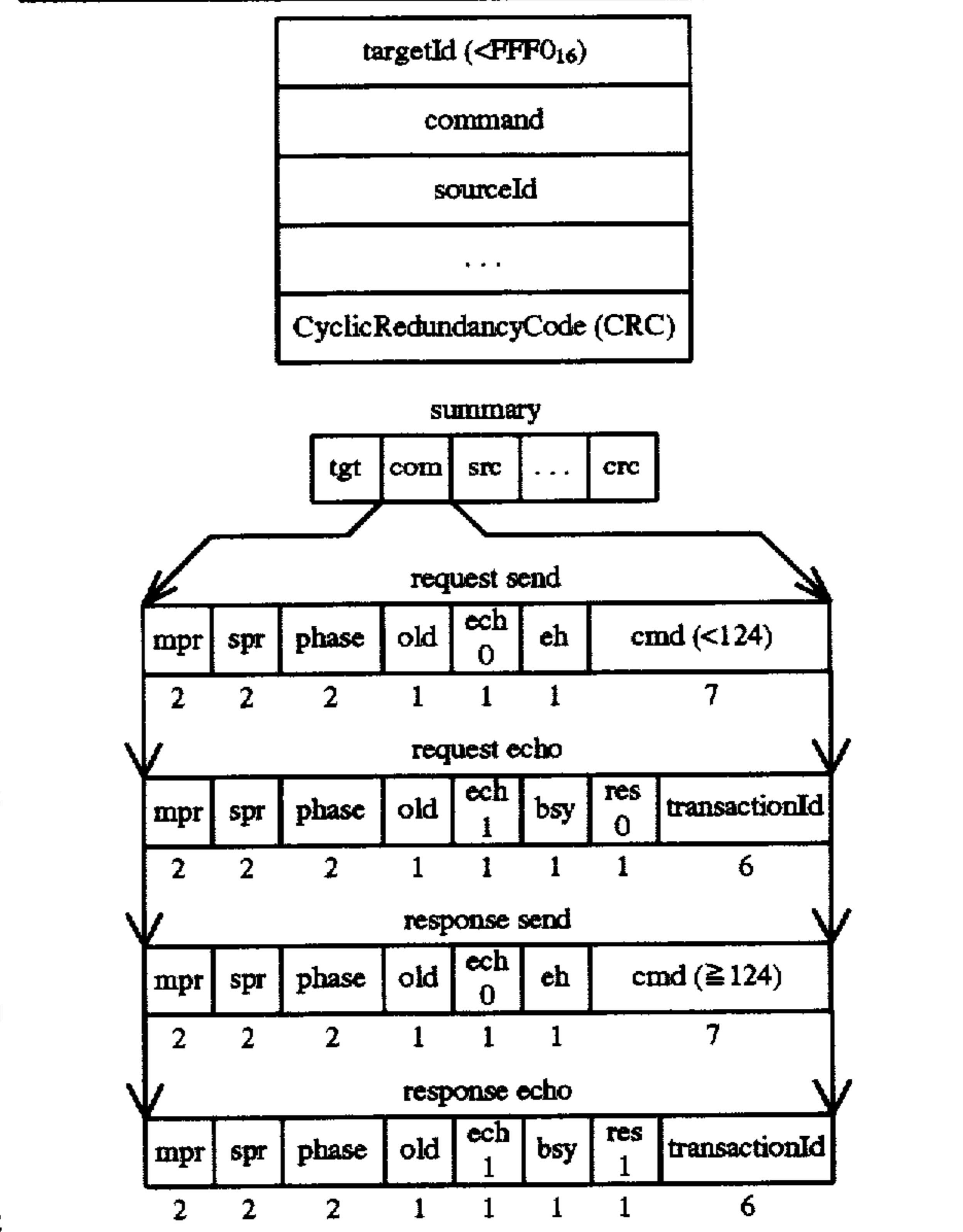
Send and Echo Packet Formats
