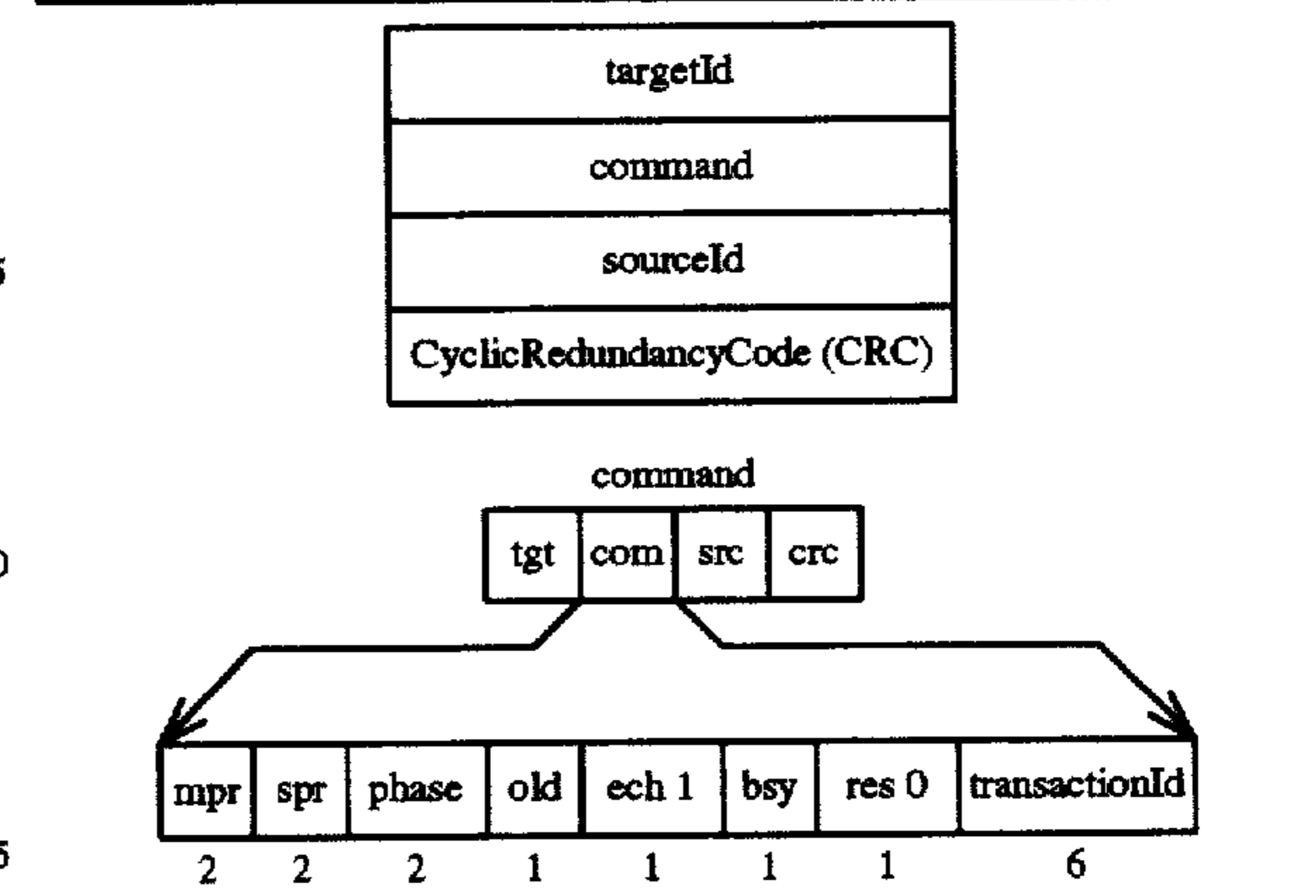
Request-Echo Packet Format
