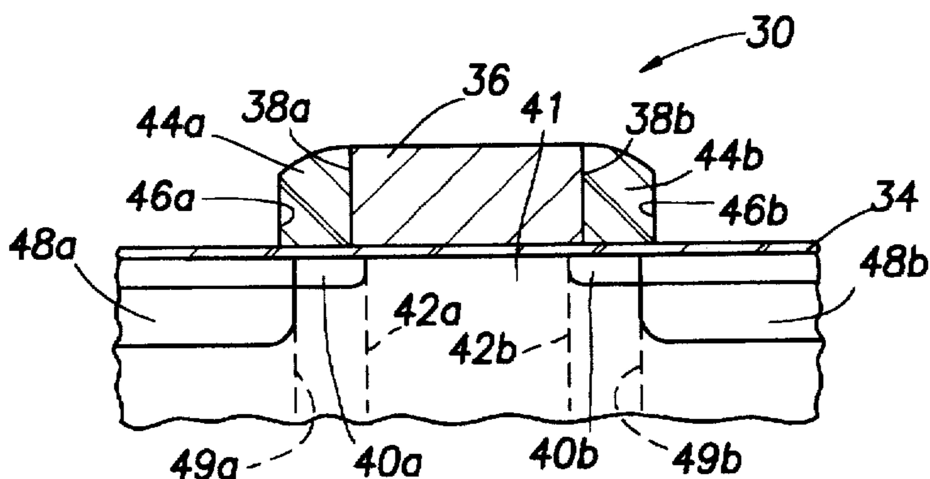
FIG. 2 (PRIOR ART)
