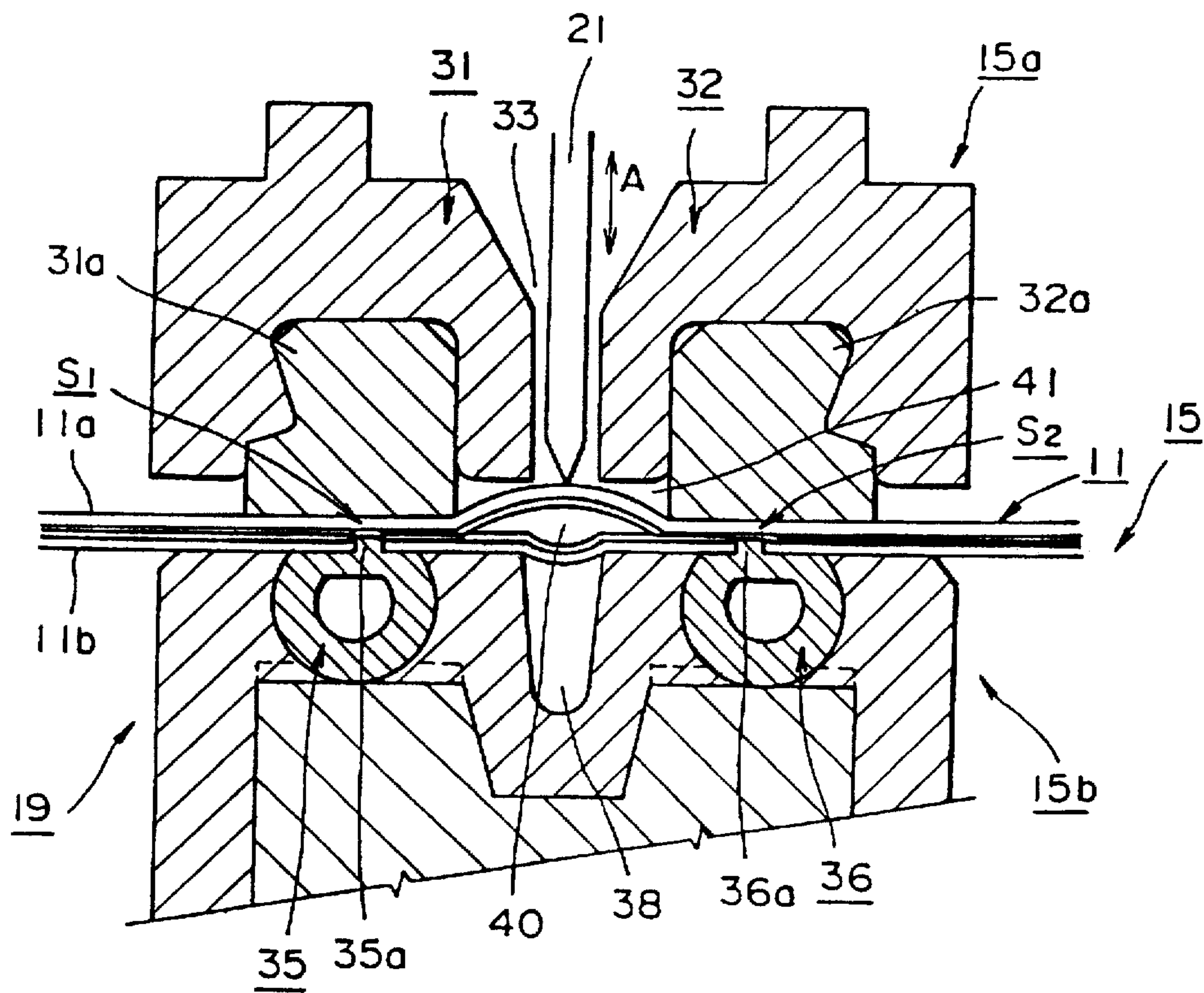
FIG. 2 (PRIOR ART)
