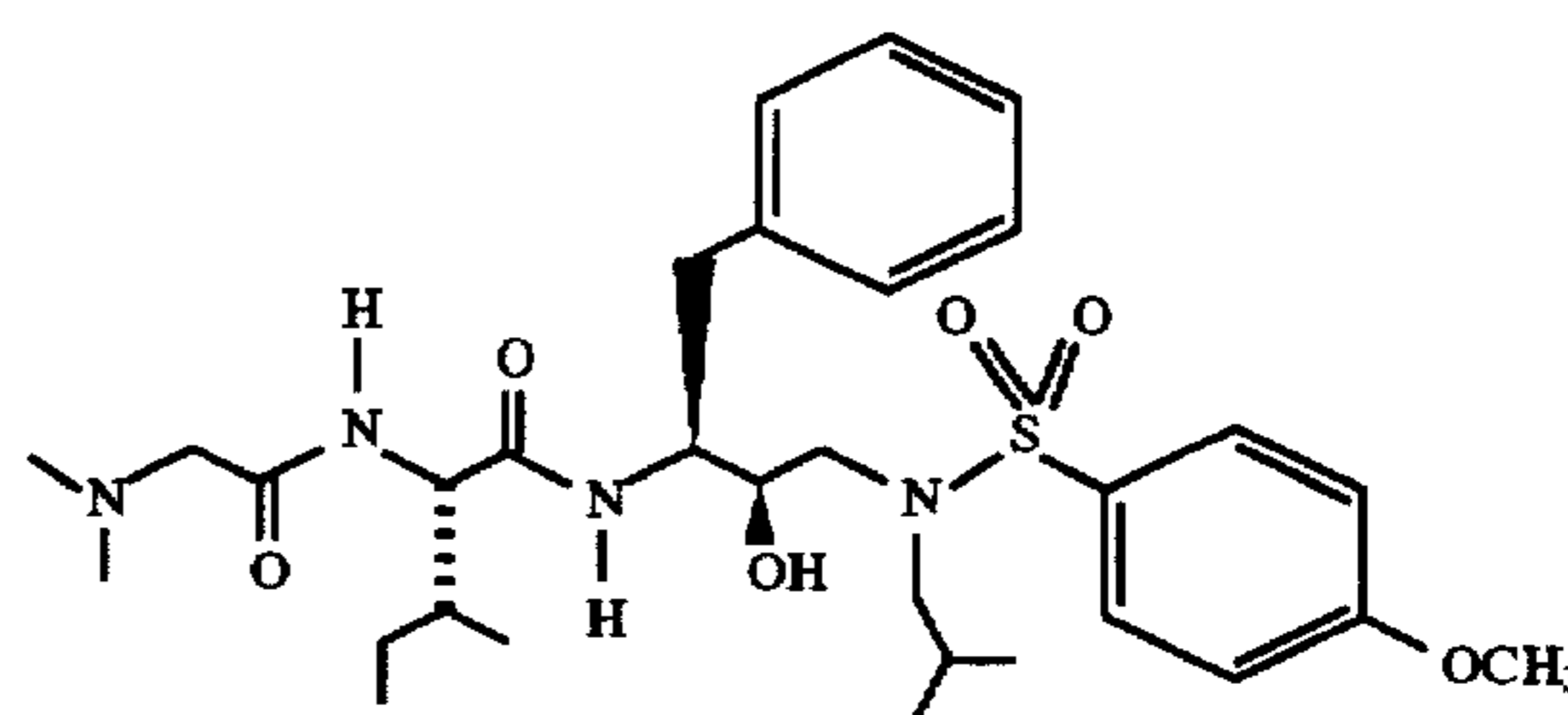
Preparation of Pentanamide, 2S-[[methylamino]acetyl]amino]-N-[2R-hydroxy-3-[(3-methylpropyl)(4-methoxyphenylsulfonyl)amino]-1S-(phenylmethyl)propyl]-3S-methyl-
