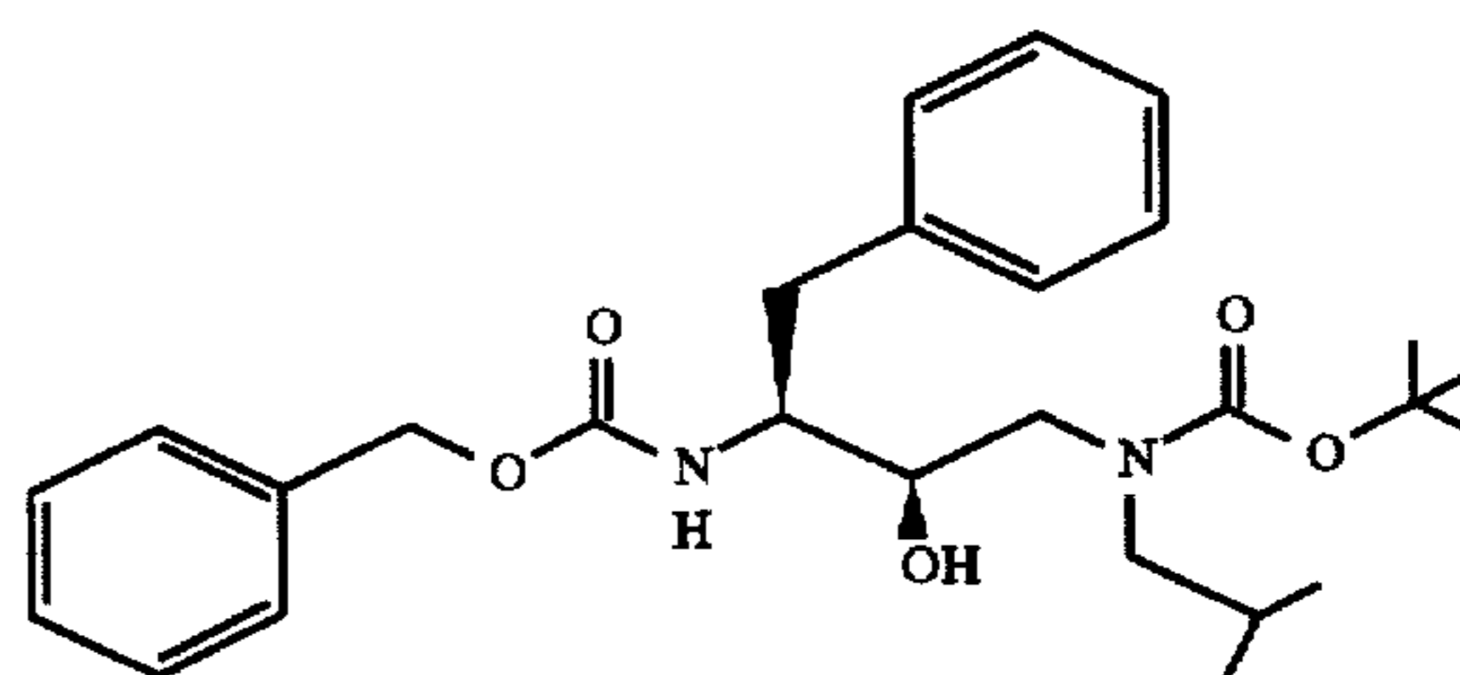
Preparation of N-[[3S-(phenylmethylcarbamoyl) amino]-2R-hydroxy-4-phenyl]-1-[(2-methylpropyl) amino]-2-(1,1-dimethylethoxy) carbonyl]butane
