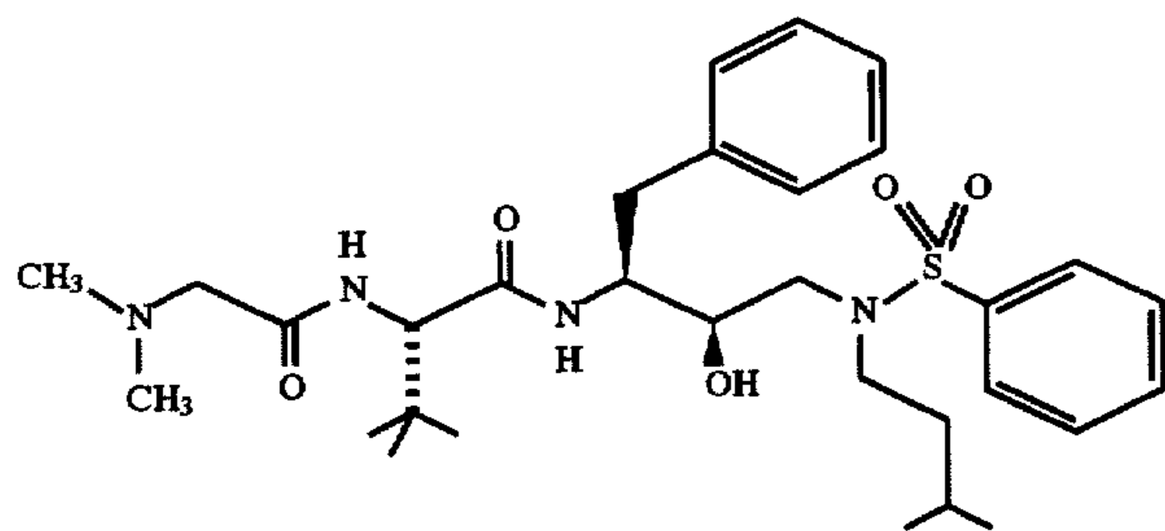
Preparation of 2S-[[[(dimethylamino)acetyl]amino]-N-[2R-hydroxy-3-[(3-methylbutyl)(phenylsulfonyl)amino]-1S-(phenylmethyl)propyl]-3,3-dimethylbutaneamide
