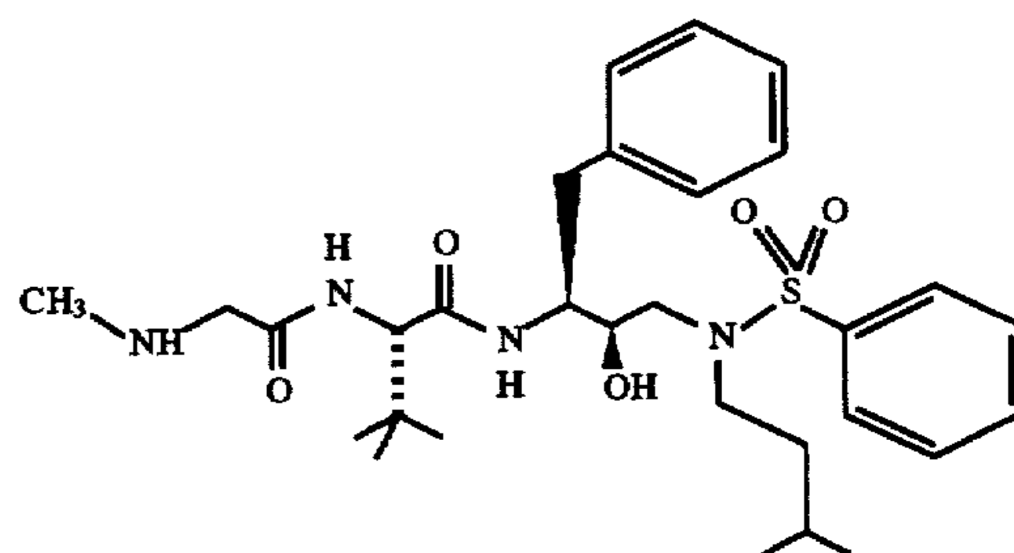
Preparation of 2S-[[[(methylamino)acetyl]amino]-N-[2R-hydroxy-3-[(3-methylbutyl)(phenylsulfonyl)amino]-1S-(phenylmethyl)propyl]-3,3-dimethylbutaneamide
