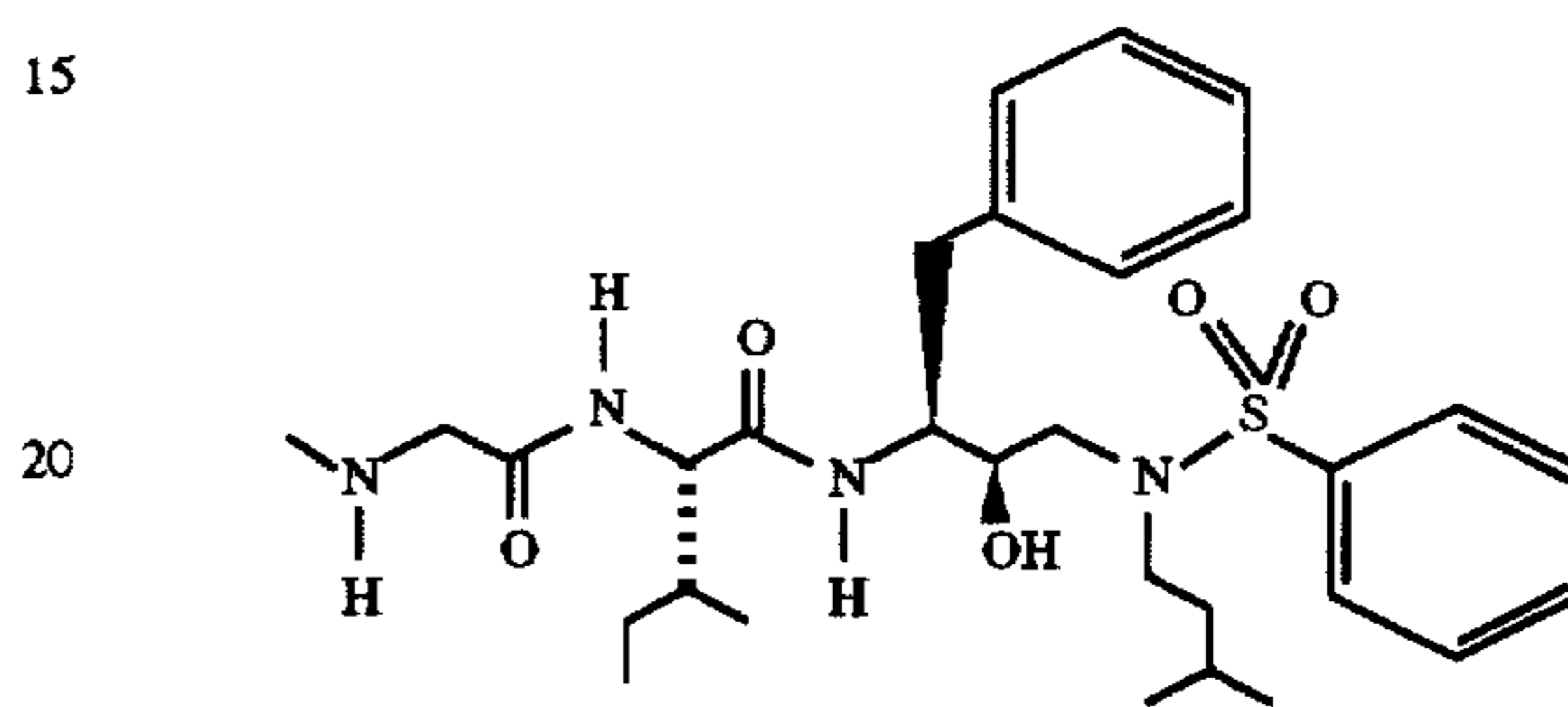
Preparation of Pentanamide, 2S-[[methylamino]acetyl]amino]-N-[2R-hydroxy-3-[(3-methylbutyl)(phenylsulfonyl)amino]-1S-(phenylmethyl)propyl]-3S-methyl-
