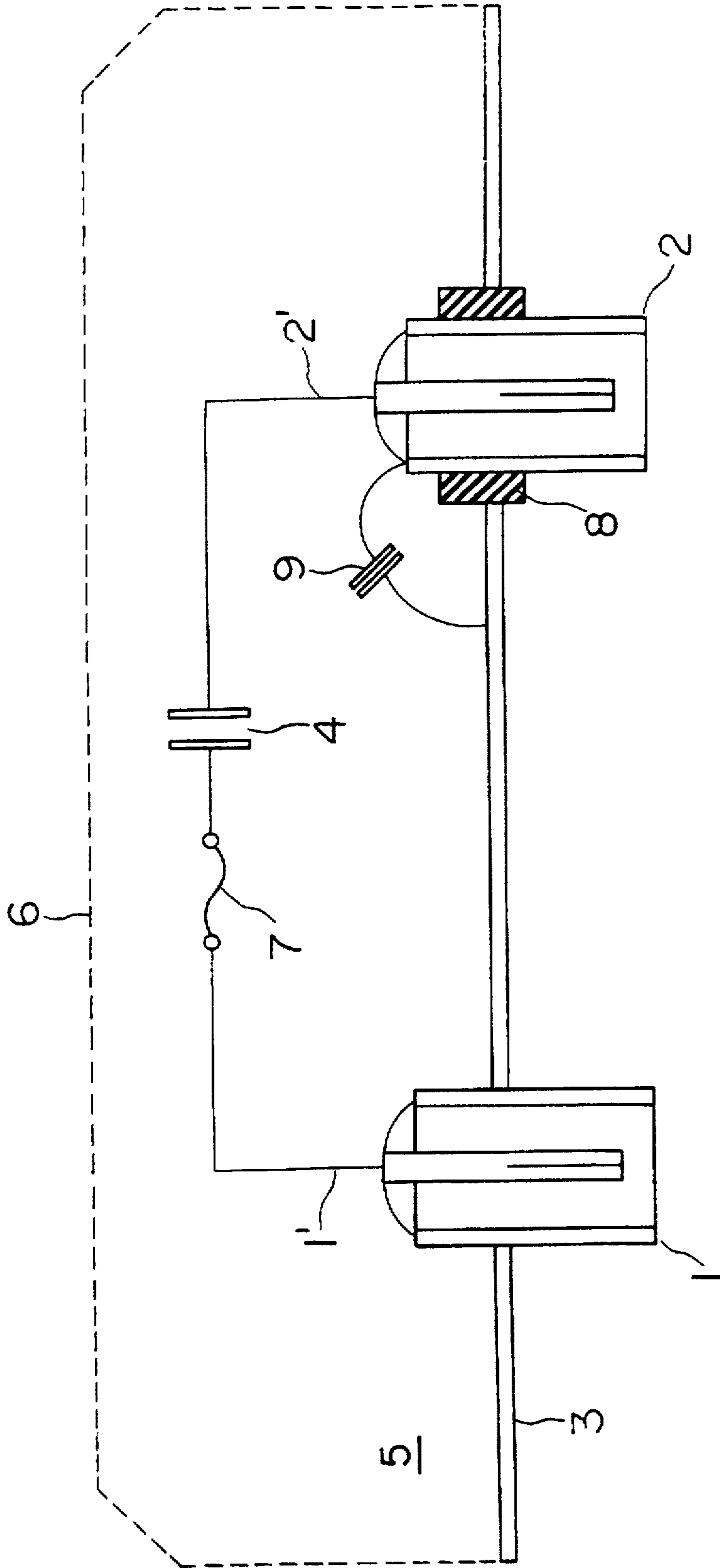
FIG. 12 (PRIOR ART)
