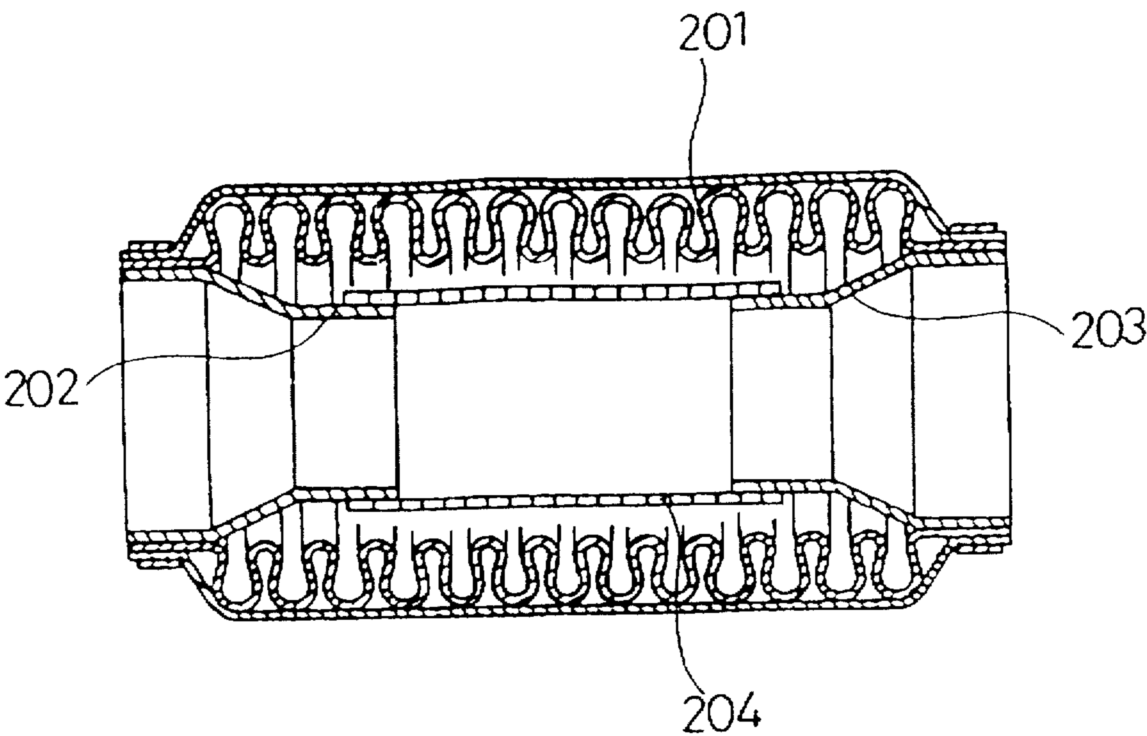
FIG.3 (PRIOR ART)
