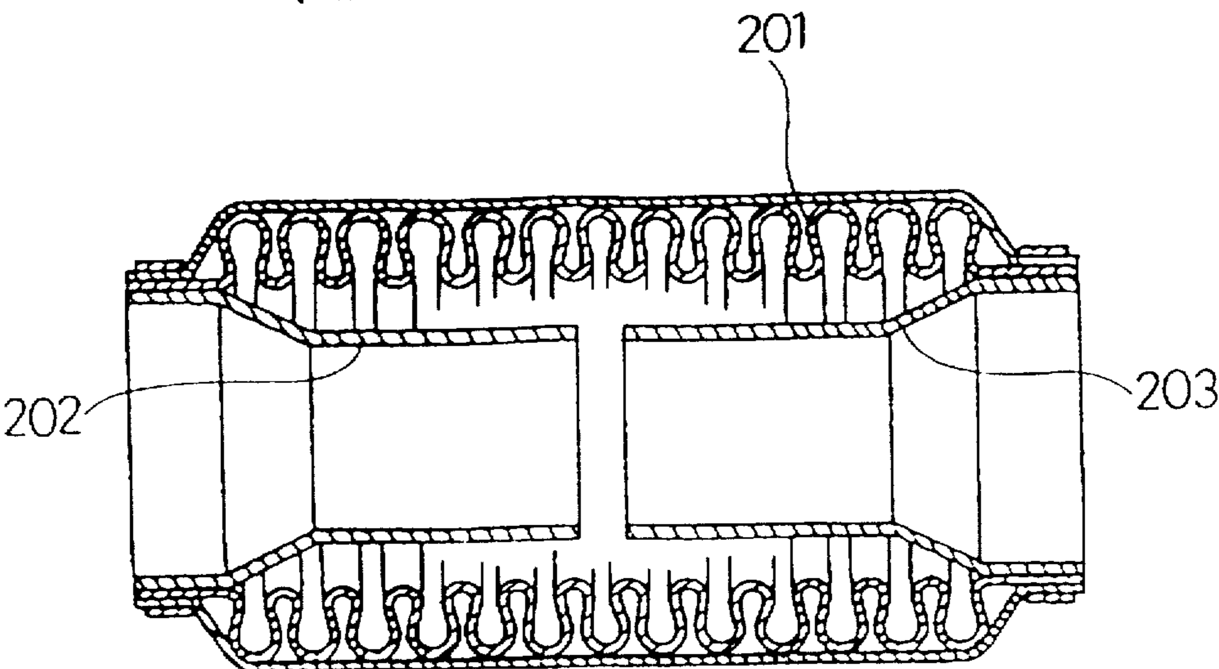
FIG.4 (RELATED ART)
