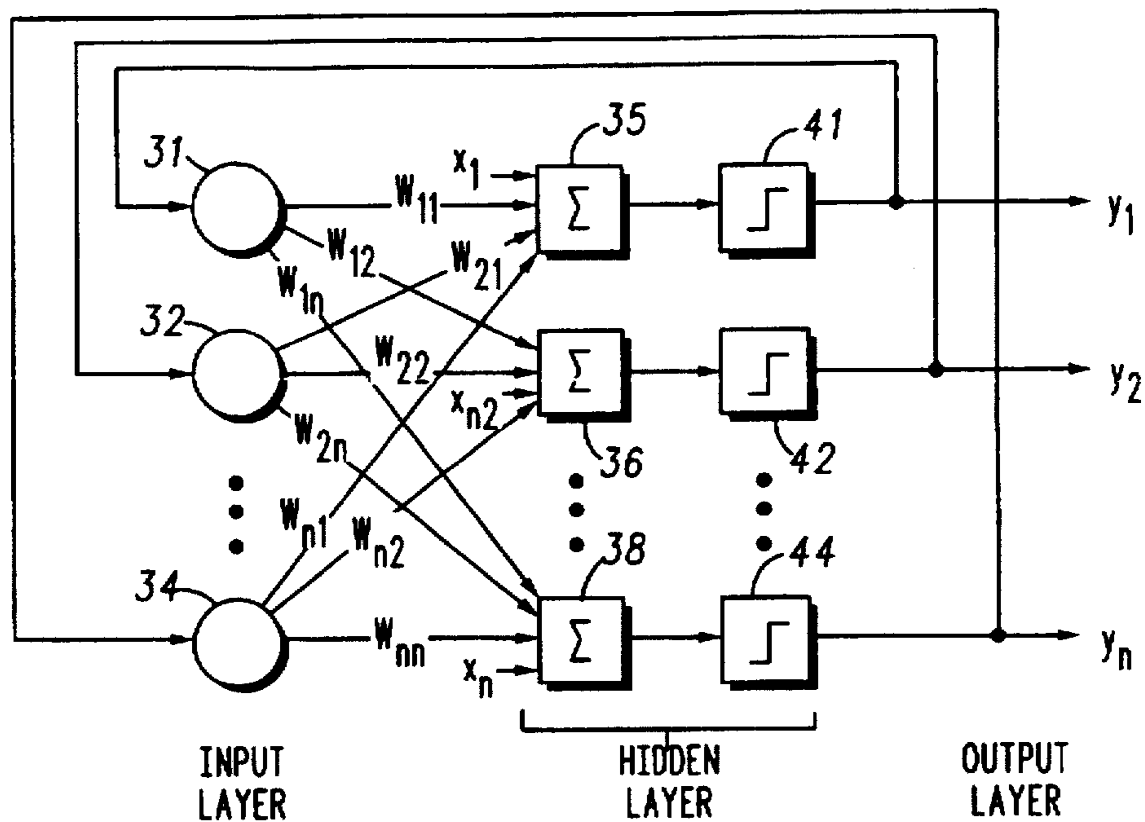
FIG. 3 —PRIOR ART—
