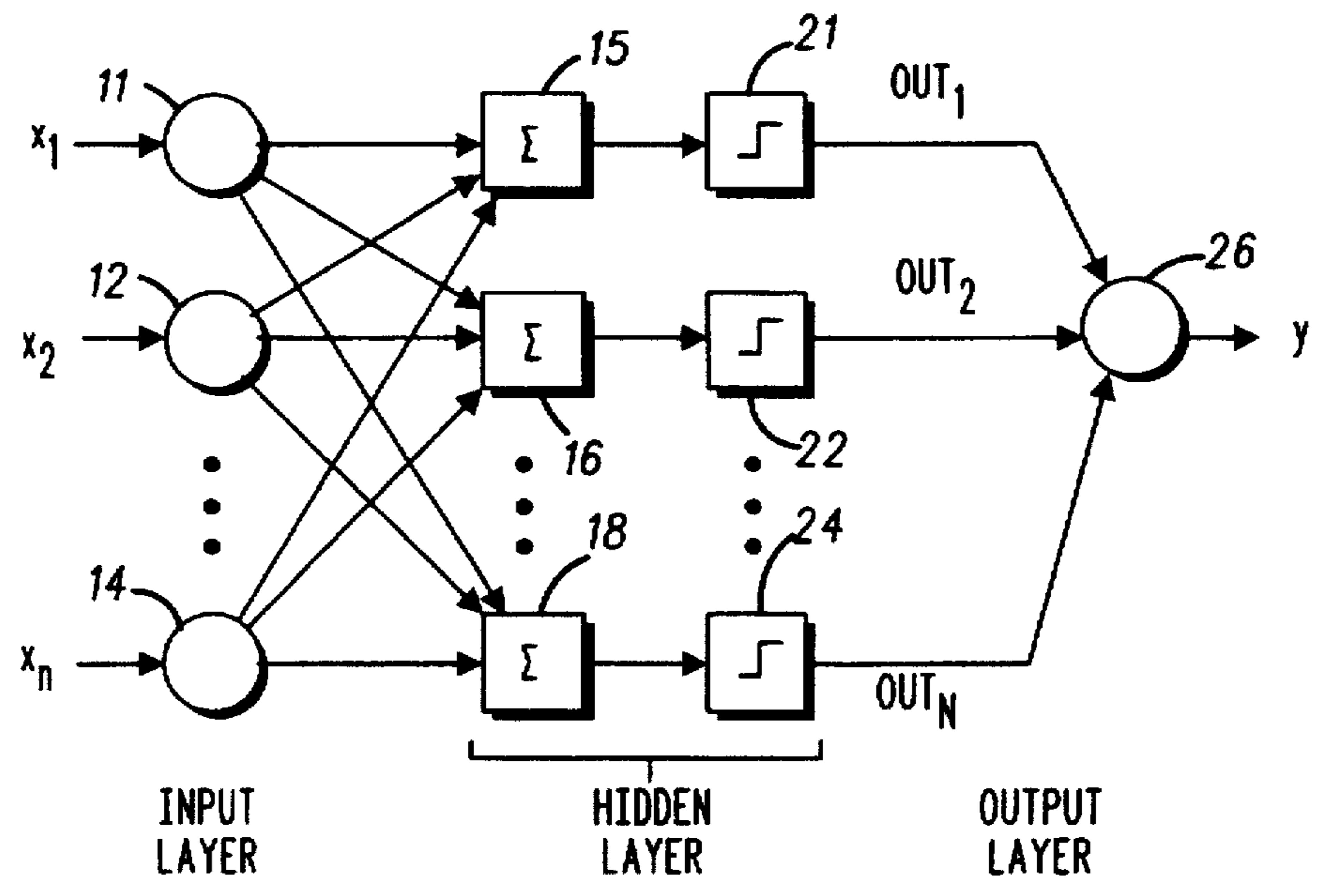
FIG. 2 —PRIOR ART—
